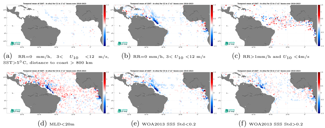
Figure 14: Temporal mean gridded over spatial boxes of size 1^\circ \times 1^\circ of \Delta\text{SSS} (SMOS SSS L3 v9 - 18 Days (CATDS-CEC-LOCEAN) - Argo) for 6 different subdatasets corresponding to:RR=0 mm/h, 3 < U_{10} < 12 m/s, SST>5°C, distance to coast > 800 km (a), RR=0 mm/h, 3 < U_{10} < 12 m/s (b), RR>1mm/h and U_{10} < 4 m/s (c),MLD<20m (d),WOA2013 SSS Std<0.2 (e),WOA2013 SSS Std>0.2 (f).
