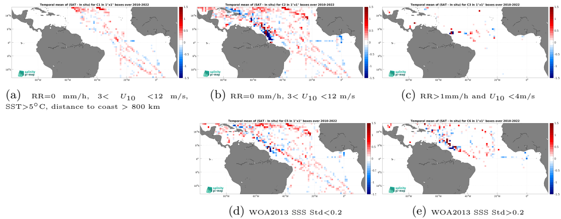
Figure 12: Temporal mean gridded over spatial boxes of size 1^\circ \times 1^\circ of \Delta SSS (SMOS SSS L3 v8 - 9 Days (CATDS-CEC-LOCEAN) - TSG (SAMOS)) for 5 different subdatasets corresponding to:RR=0 mm/h, 3 < U_{10} < 12 m/s, SST >5^\circ\text{C} , distance to coast > 800 km (a), RR=0 mm/h, 3 < U_{10} < 12 m/s (b), RR >1 mm/h and U_{10} < 4 m/s (c), WOA2013 SSS Std <0.2 (d), WOA2013 SSS Std >0.2 (e).
