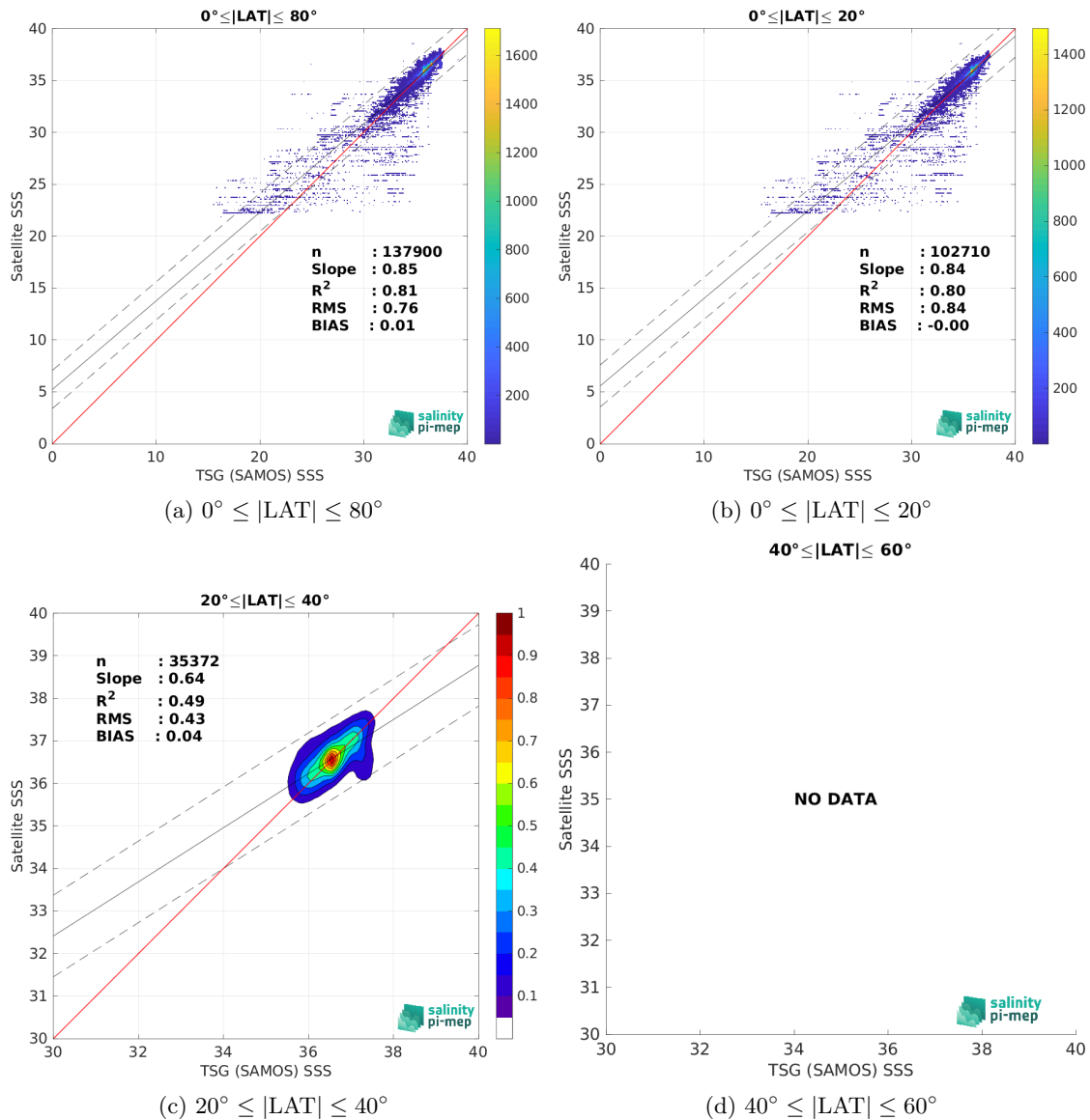
Figure 9: Contour maps of the concentration of SMOS SSS L3 v8 - 9 Days (CATDS-CEC-LOCEAN) SSS (y-axis) versus TSG (SAMOS) SSS (x-axis) at match-up pairs for different latitude bands. For each plot, the red line shows x=y . The black thin and dashed lines indicate a linear fit through the data cloud and the \pm 95\% confidence levels, respectively. The number match-up pairs n , the slope and R^2 coefficient of the linear fit, the root mean square (RMS) and the mean bias between satellite and in situ data are indicated for each latitude band in each plots.
