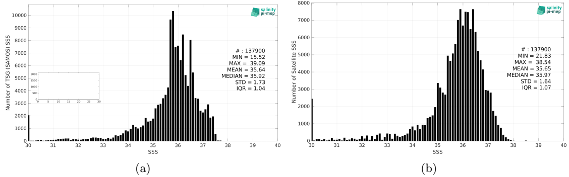
Figure 2: Histograms of SSS from TSG (SAMOS) (a) and SMOS SSS L3 v8 - 9 Days (CATDS-CEC-LOCEAN) (b) considering all match-up pairs per bins of 0.1 over the Tropical Atlantic Ocean Pi-MEP region and for the full satellite product period.
