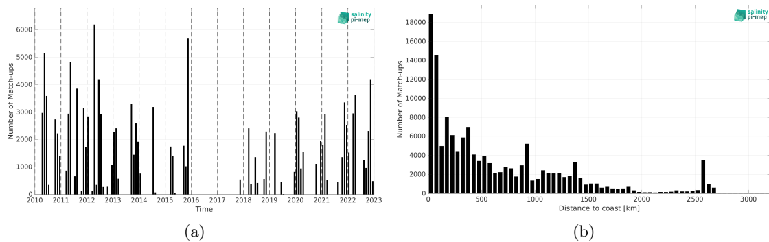
Figure 1: Number of match-ups between TSG (SAMOS) and SMOS SSS L3 v8 - 9 Days (CATDS-CEC-LOCEAN) SSS as a function of time (a) and as function of the distance to coast (b) over the Tropical Atlantic Ocean Pi-MEP region and for the full satellite product period.
