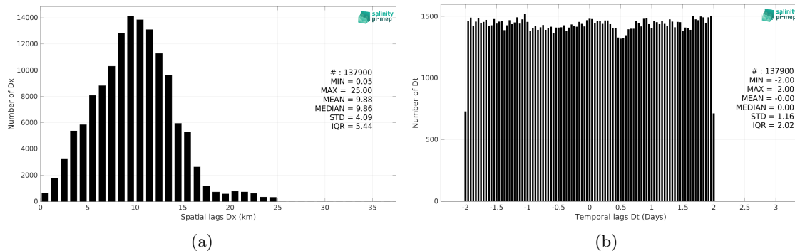
Figure 5: Histograms of the spatial (a) and temporal (b) lags between the location/time of the TSG (SAMOS) measurement and the date of the corresponding SMOS SSS L3 v8 - 9 Days (CATDS-CEC-LOCEAN) SSS pixel.
