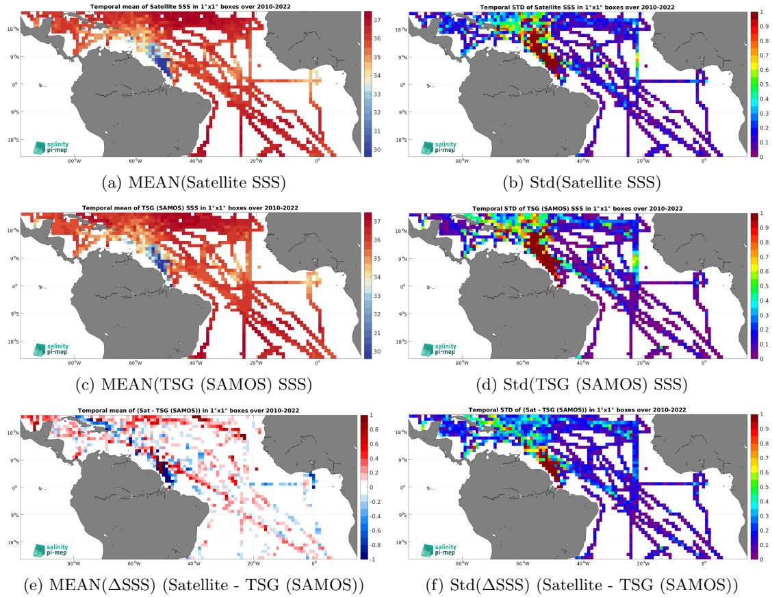
Figure 6: Temporal mean (left) and Std (right) of SSS from SMOS SSS L3 v8 - 9 Days (CATDS-CEC-LOCEAN) (top), TSG (SAMOS) (middle), and of \Delta\text{SSS} (Satellite - TSG (SAMOS)). Only match-up pairs are used to generate these maps.
