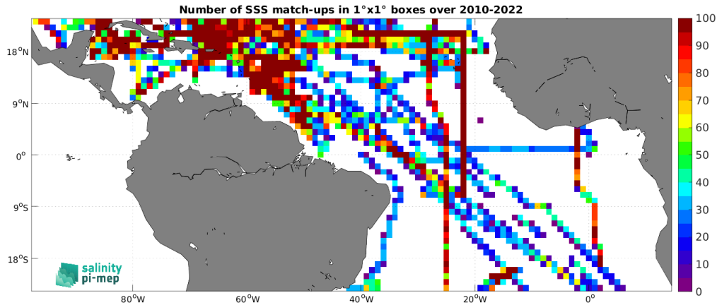
Figure 4: Number of SSS match-ups between TSG (SAMOS) SSS and the SMOS SSS L3 v8 - 9 Days (CATDS-CEC-LOCEAN) SSS product for the Tropical Atlantic Ocean Pi-MEP region over 1^\circ \times 1^\circ boxes and for the full satellite product period.
