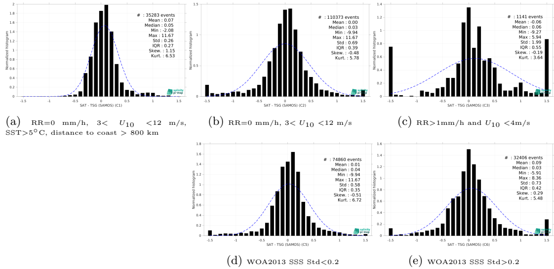
Figure 13: Normalized histogram of \Delta SSS (SMOS SSS L3 v8 - 9 Days (CATDS-CEC-LOCEAN) - TSG (SAMOS)) for 5 different subdatasets corresponding to: RR=0 mm/h, 3 < U_{10} < 12 m/s, SST > 5°C, distance to coast > 800 km (a), RR=0 mm/h, 3 < U_{10} < 12 m/s (b), RR > 1mm/h and U_{10} < 4 m/s (c), WOA2013 SSS Std < 0.2 (d), WOA2013 SSS Std > 0.2 (e).
