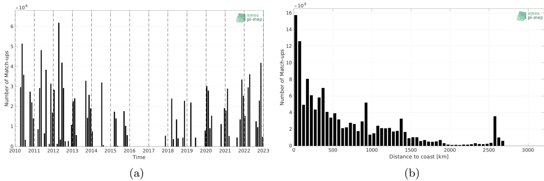
Figure 1: Number of match-ups between TSG (SAMOS) and SMOS SSS L3 v8 - 9 Days (CATDS-CECOS-LOCEAN) SSS as a function of time (a) and as function of the distance to coast (b) over the Tropical Atlantic Ocean Pi-MEP region and for the full satellite product period.
