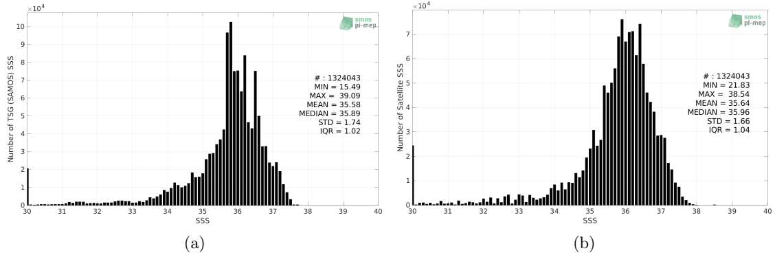
Figure 2: Histograms of SSS from TSG (SAMOS) (a) and SMOS SSS L3 v8 - 9 Days (CATDS-CECOS-LOCEAN) (b) considering all match-up pairs per bins of 0.1 over the Tropical Atlantic Ocean Pi-MEP region and for the full satellite product period.
