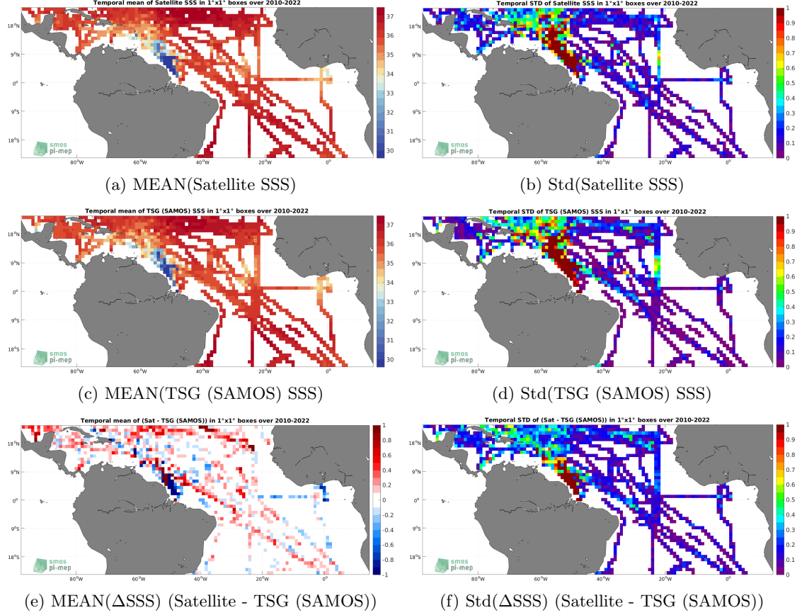
Figure 6: Temporal mean (left) and Std (right) of SSS from SMOS SSS L3 v8 - 9 Days (CATDS-CECOS-LOCEAN) (top), TSG (SAMOS) (middle), and of \Delta\text{SSS} (Satellite - TSG (SAMOS)). Only match-up pairs are used to generate these maps.
