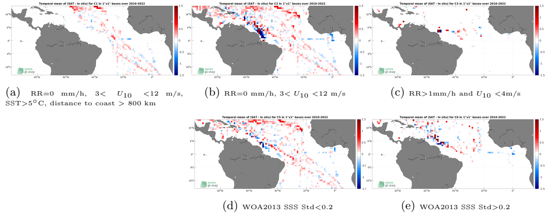
Figure 12: Temporal mean gridded over spatial boxes of size 1^{\circ}\times 1^{\circ} of \Delta\text{SSS} (SMOS SSS L3 v8 - 9 Days (CATDS-CECOS-LOCEAN) - TSG (SAMOS)) for 5 different subdatasets corresponding to:RR=0 mm/h, 3 < U_{10} < 12 m/s, SST > 5^{\circ}\text{C} , distance to coast > 800 km (a), RR=0 mm/h, 3 < U_{10} < 12 m/s (b), RR > 1 mm/h and U_{10} < 4 m/s (c), WOA2013 SSS Std < 0.2 (d), WOA2013 SSS Std > 0.2 (e).
