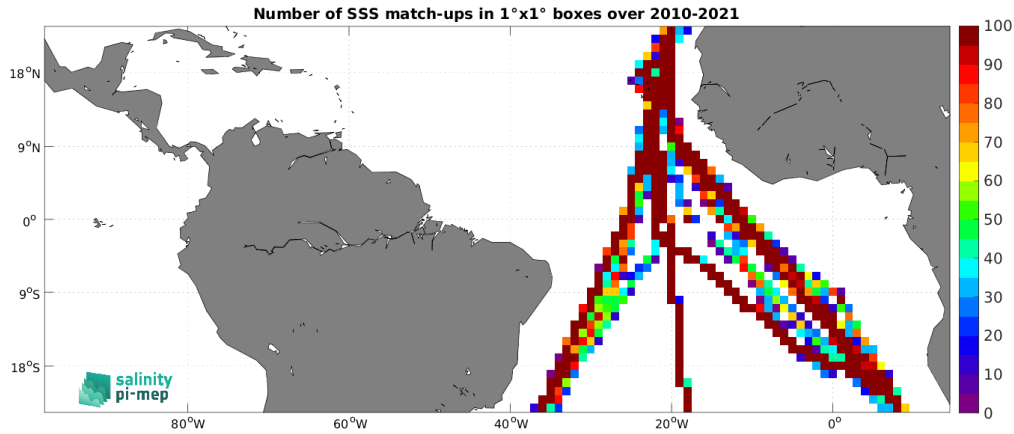
Figure 4: Number of SSS match-ups between TSG (Polarstern) SSS and the SMOS SSS L3 v8 - 9 Days (CATDS-CEC-LOCEAN) SSS product for the Tropical Atlantic Ocean Pi-MEP region over 1^\circ \times 1^\circ boxes and for the full satellite product period.
