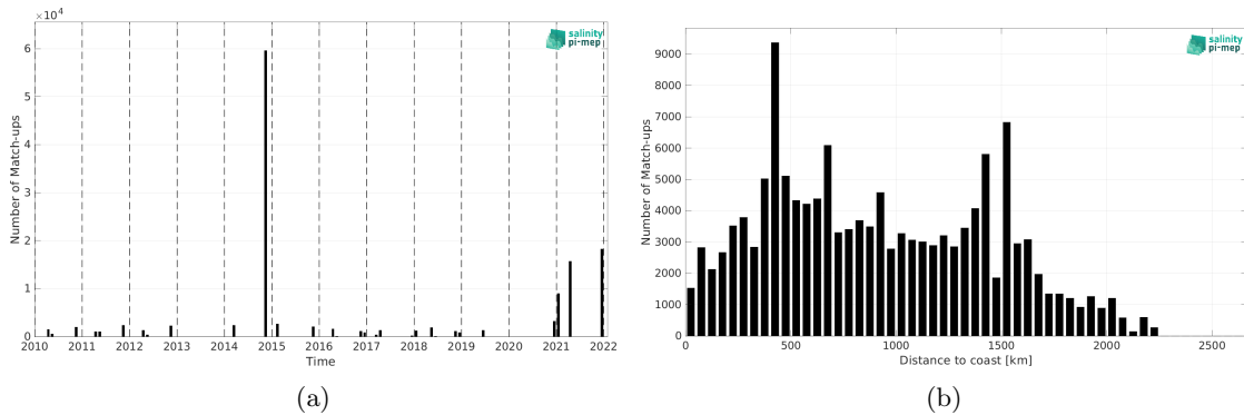
Figure 1: Number of match-ups between TSG (Polarstern) and SMOS SSS L3 v8 - 9 Days (CATDS-CEC-LOCEAN) SSS as a function of time (a) and as function of the distance to coast (b) over the Tropical Atlantic Ocean Pi-MEP region and for the full satellite product period.
