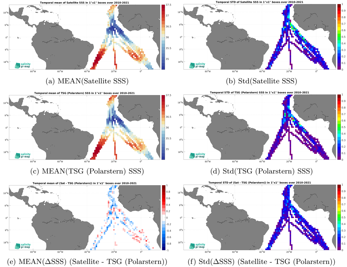
Figure 6: Temporal mean (left) and Std (right) of SSS from SMOS SSS L3 v8 - 9 Days (CATDS-CEC-LOCEAN) (top), TSG (Polarstern) (middle), and of \Delta\text{SSS}(\text{Satellite} - \text{TSG}(\text{Polarstern})) . Only match-up pairs are used to generate these maps.
