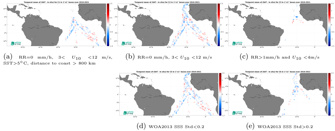
Figure 12: Temporal mean gridded over spatial boxes of size 1^{\circ}\times 1^{\circ} of \Delta\text{SSS} (SMOS SSS L3 v8 - 9 Days (CATDS-CEC-LOCEAN) - TSG (Polarstern)) for 5 different subdatasets corresponding to:RR=0 mm/h, 3 < U_{10} < 12 m/s, SST > 5^{\circ}\text{C} , distance to coast > 800 km (a), RR=0 mm/h, 3 < U_{10} < 12 m/s (b), RR > 1 mm/h and U_{10} < 4 m/s (c), WOA2013 SSS Std < 0.2 (d), WOA2013 SSS Std > 0.2 (e).
