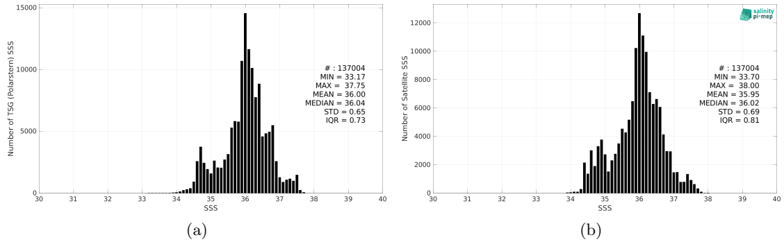
Figure 2: Histograms of SSS from TSG (Polarstern) (a) and SMOS SSS L3 v8 - 9 Days (CATDS-CEC-LOCEAN) (b) considering all match-up pairs per bins of 0.1 over the Tropical Atlantic Ocean Pi-MEP region and for the full satellite product period.
