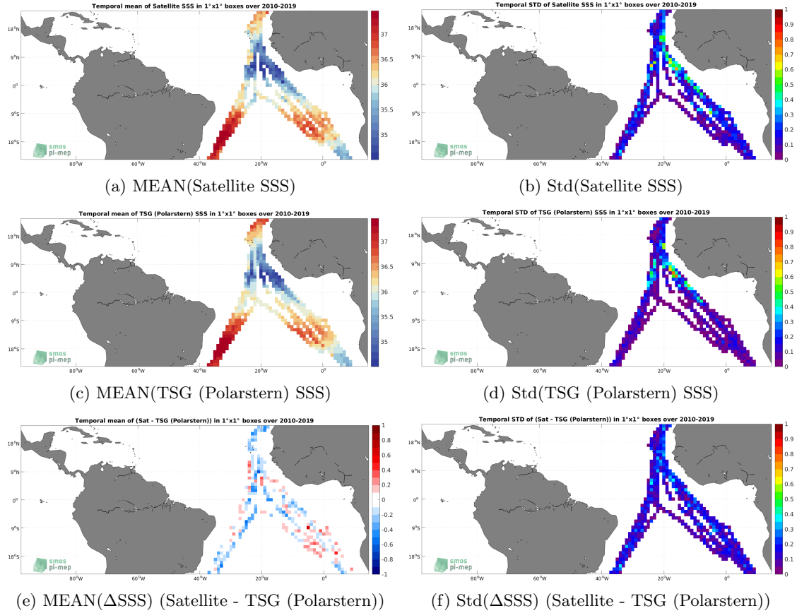
Figure 6: Temporal mean (left) and Std (right) of SSS from SMOS SSS L3 v8 - 9 Days (CATDS-CECOS-LOCEAN) (top), TSG (Polarstern) (middle), and of \Delta\text{SSS} (Satellite - TSG (Polarstern)). Only match-up pairs are used to generate these maps.
