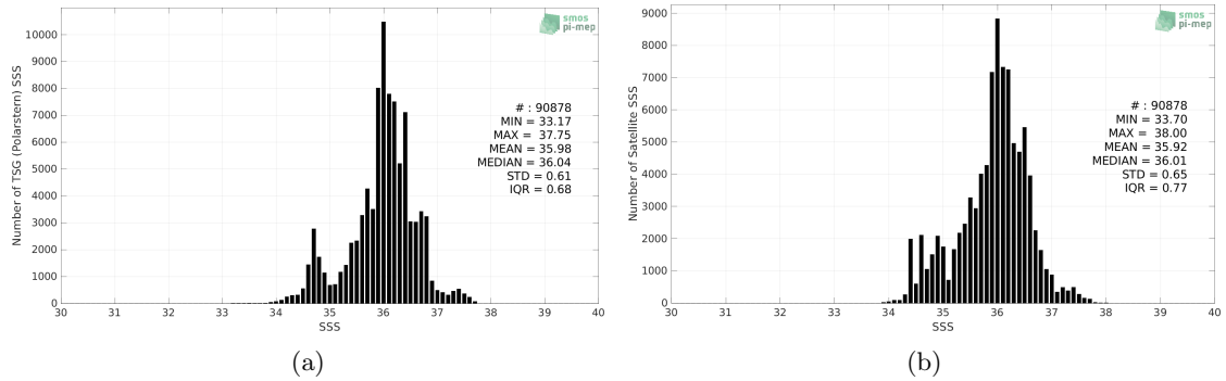
Figure 2: Histograms of SSS from TSG (Polarstern) (a) and SMOS SSS L3 v8 - 9 Days (CATDS-CECOS-LOCEAN) (b) considering all match-up pairs per bins of 0.1 over the Tropical Atlantic Ocean Pi-MEP region and for the full satellite product period.
