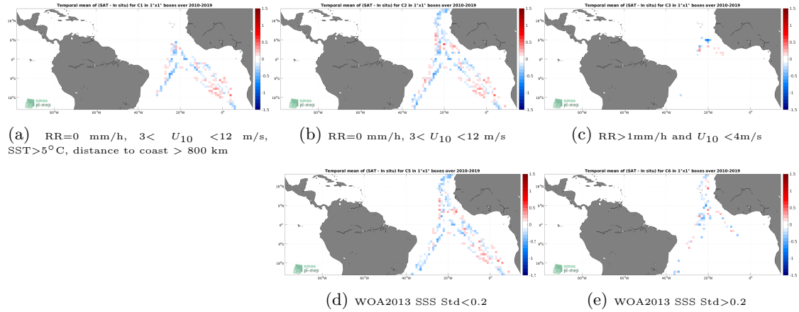
Figure 12: Temporal mean gridded over spatial boxes of size 1^{\circ}\times 1^{\circ} of \Delta\text{SSS} (SMOS SSS L3 v8 - 9 Days (CATDS-CECOS-LOCEAN) - TSG (Polarstern)) for 5 different subdatasets corresponding to:RR=0 mm/h, 3 < U_{10} < 12 m/s, SST > 5^{\circ}\text{C} , distance to coast > 800 km (a), RR=0 mm/h, 3 < U_{10} < 12 m/s (b), RR > 1 mm/h and U_{10} < 4 m/s (c), WOA2013 SSS Std < 0.2 (d), WOA2013 SSS Std > 0.2 (e).
