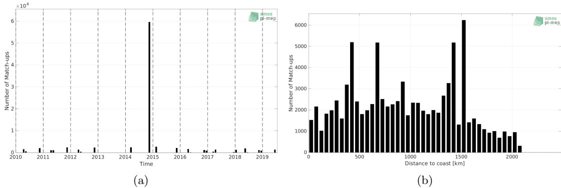
Figure 1: Number of match-ups between TSG (Polarstern) and SMOS SSS L3 v8 - 9 Days (CATDS-CECOS-LOCEAN) SSS as a function of time (a) and as function of the distance to coast (b) over the Tropical Atlantic Ocean Pi-MEP region and for the full satellite product period.
