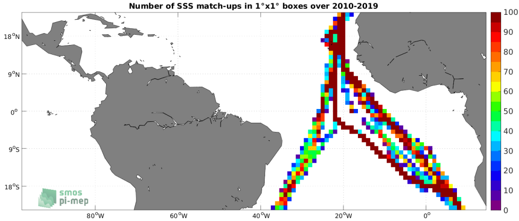
Figure 4: Number of SSS match-ups between TSG (Polarstern) SSS and the SMOS SSS L3 v8 - 9 Days (CATDS-CECOS-LOCEAN) SSS product for the Tropical Atlantic Ocean Pi-MEP region over 1^\circ \times 1^\circ boxes and for the full satellite product period.
