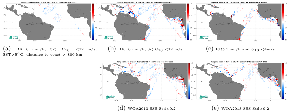
Figure 12: Temporal mean gridded over spatial boxes of size 1^\circ \times 1^\circ of \Delta\text{SSS} (SMOS SSS L3 v8 - 9 Days (CATDS-CEC-LOCEAN) - TSG (LEGOS-DM)) for 5 different subdatasets corresponding to:RR=0 mm/h, 3 < U_{10} < 12 m/s, SST >5^\circ\text{C} , distance to coast > 800 km (a), RR=0 mm/h, 3 < U_{10} < 12 m/s (b), RR >1 mm/h and U_{10} < 4 m/s (c), WOA2013 SSS Std <0.2 (d), WOA2013 SSS Std >0.2 (e).
