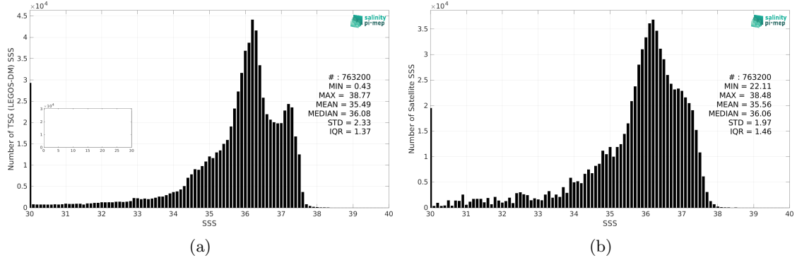
Figure 2: Histograms of SSS from TSG (LEGOS-DM) (a) and SMOS SSS L3 v8 - 9 Days (CATDS-CEC-LOCEAN) (b) considering all match-up pairs per bins of 0.1 over the Tropical Atlantic Ocean Pi-MEP region and for the full satellite product period.
