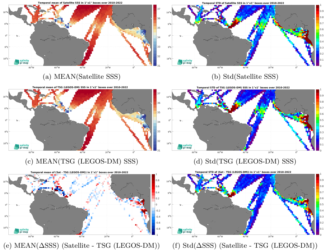
Figure 6: Temporal mean (left) and Std (right) of SSS from SMOS SSS L3 v8 - 9 Days (CATDS-CEC-LOCEAN) (top), TSG (LEGOS-DM) (middle), and of \Delta\text{SSS} (Satellite - TSG (LEGOS-DM)). Only match-up pairs are used to generate these maps.
