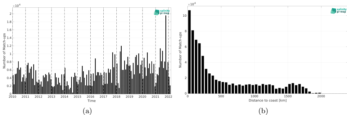
Figure 1: Number of match-ups between TSG (LEGOS-DM) and SMOS SSS L3 v8 - 9 Days (CATDS-CEC-LOCEAN) SSS as a function of time (a) and as function of the distance to coast (b) over the Tropical Atlantic Ocean Pi-MEP region and for the full satellite product period.
