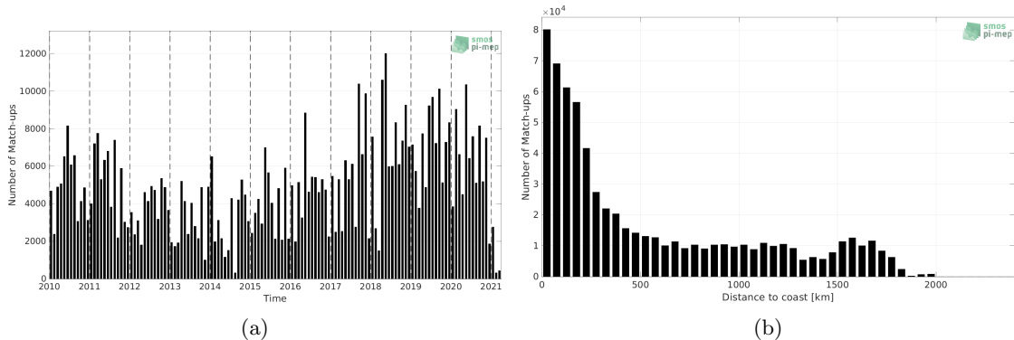
Figure 1: Number of match-ups between TSG (LEGOS-DM) and SMOS SSS L3 v8 - 9 Days (CATDS-CECOS-LOCEAN) SSS as a function of time (a) and as function of the distance to coast (b) over the Tropical Atlantic Ocean Pi-MEP region and for the full satellite product period.
