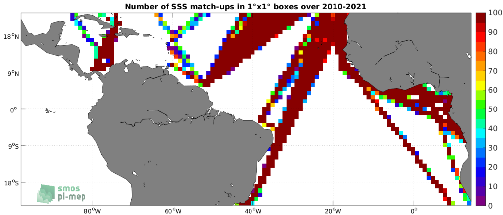
Figure 4: Number of SSS match-ups between TSG (LEGOS-DM) SSS and the SMOS SSS L3 v8 - 9 Days (CATDS-CECOS-LOCEAN) SSS product for the Tropical Atlantic Ocean Pi-MEP region over 1^\circ \times 1^\circ boxes and for the full satellite product period.
