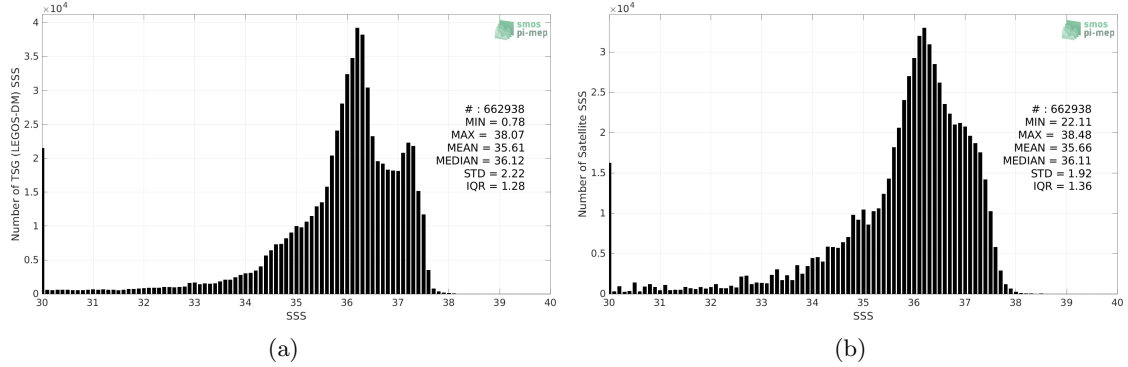
Figure 2: Histograms of SSS from TSG (LEGOS-DM) (a) and SMOS SSS L3 v8 - 9 Days (CATDS-CECOS-LOCEAN) (b) considering all match-up pairs per bins of 0.1 over the Tropical Atlantic Ocean Pi-MEP region and for the full satellite product period.
