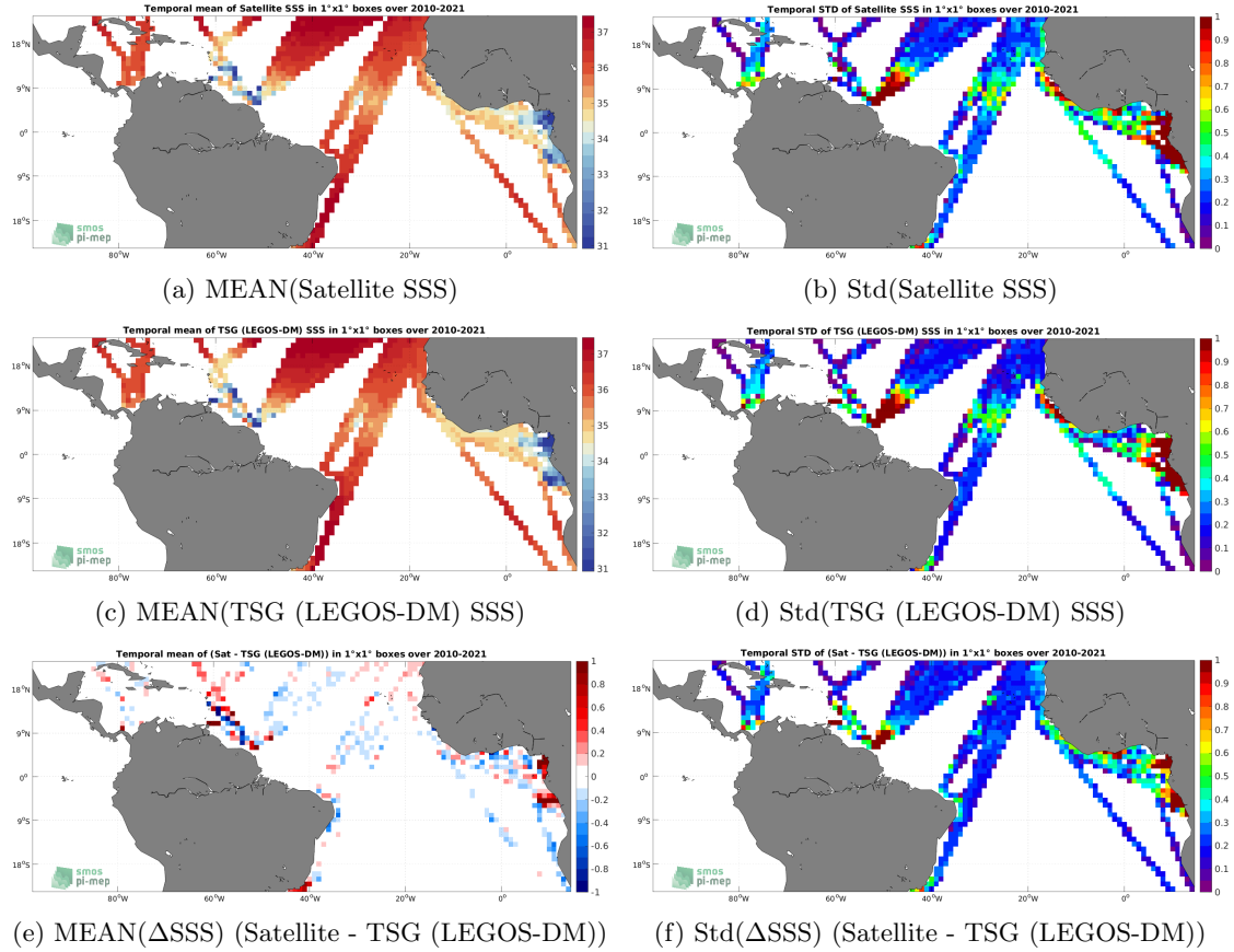
Figure 6: Temporal mean (left) and Std (right) of SSS from SMOS SSS L3 v8 - 9 Days (CATDS-CECOS-LOCEAN) (top), TSG (LEGOS-DM) (middle), and of \Delta\text{SSS} (Satellite - TSG (LEGOS-DM)). Only match-up pairs are used to generate these maps.
