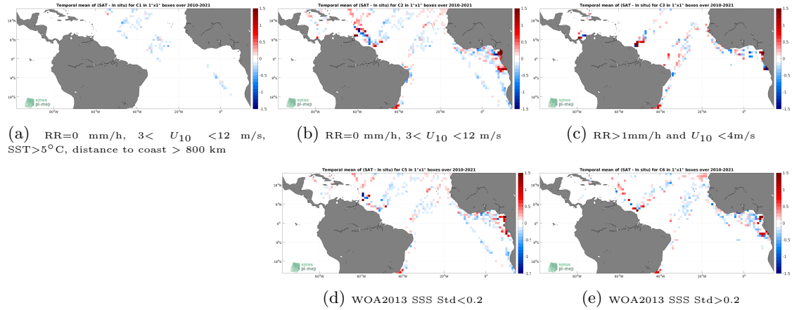
Figure 12: Temporal mean gridded over spatial boxes of size 1^{\circ}\times 1^{\circ} of \Delta\text{SSS} (SMOS SSS L3 v8 - 9 Days (CATDS-CECOS-LOCEAN) - TSG (LEGOS-DM)) for 5 different subdatasets corresponding to: RR=0 mm/h, 3 < U_{10} < 12 m/s, SST > 5^{\circ}\text{C} , distance to coast > 800 km (a), RR=0 mm/h, 3 < U_{10} < 12 m/s (b), RR > 1 mm/h and U_{10} < 4 m/s (c), WOA2013 SSS Std < 0.2 (d), WOA2013 SSS Std > 0.2 (e).
