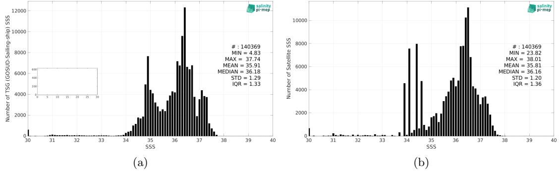
Figure 2: Histograms of SSS from TSG (GOSUD-Sailing-ship) (a) and SMOS SSS L3 v8 - 9 Days (CATDS-CEC-LOCEAN) (b) considering all match-up pairs per bins of 0.1 over the Tropical Atlantic Ocean Pi-MEP region and for the full satellite product period.
