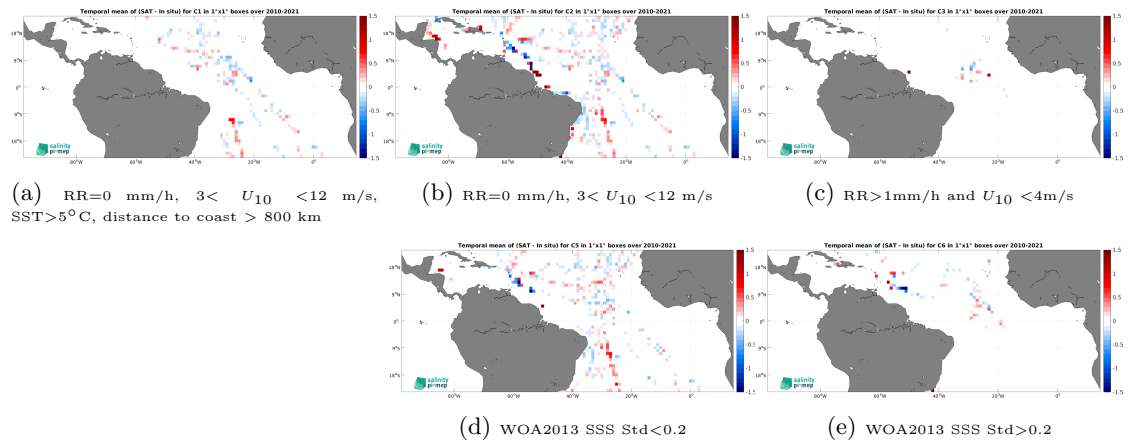
Figure 12: Temporal mean gridded over spatial boxes of size 1^{\circ}\times 1^{\circ} of \Delta SSS (SMOS SSS L3 v8 - 9 Days (CATDS-CEC-LOCEAN) - TSG (GOSUD-Sailing-ship)) for 5 different subdatasets corresponding to:RR=0 mm/h, 3 < U_{10} < 12 m/s, SST >5^{\circ}\text{C} , distance to coast > 800 km (a), RR=0 mm/h, 3 < U_{10} < 12 m/s (b), RR >1 mm/h and U_{10} < 4 m/s (c), WOA2013 SSS Std <0.2 (d), WOA2013 SSS Std >0.2 (e).
