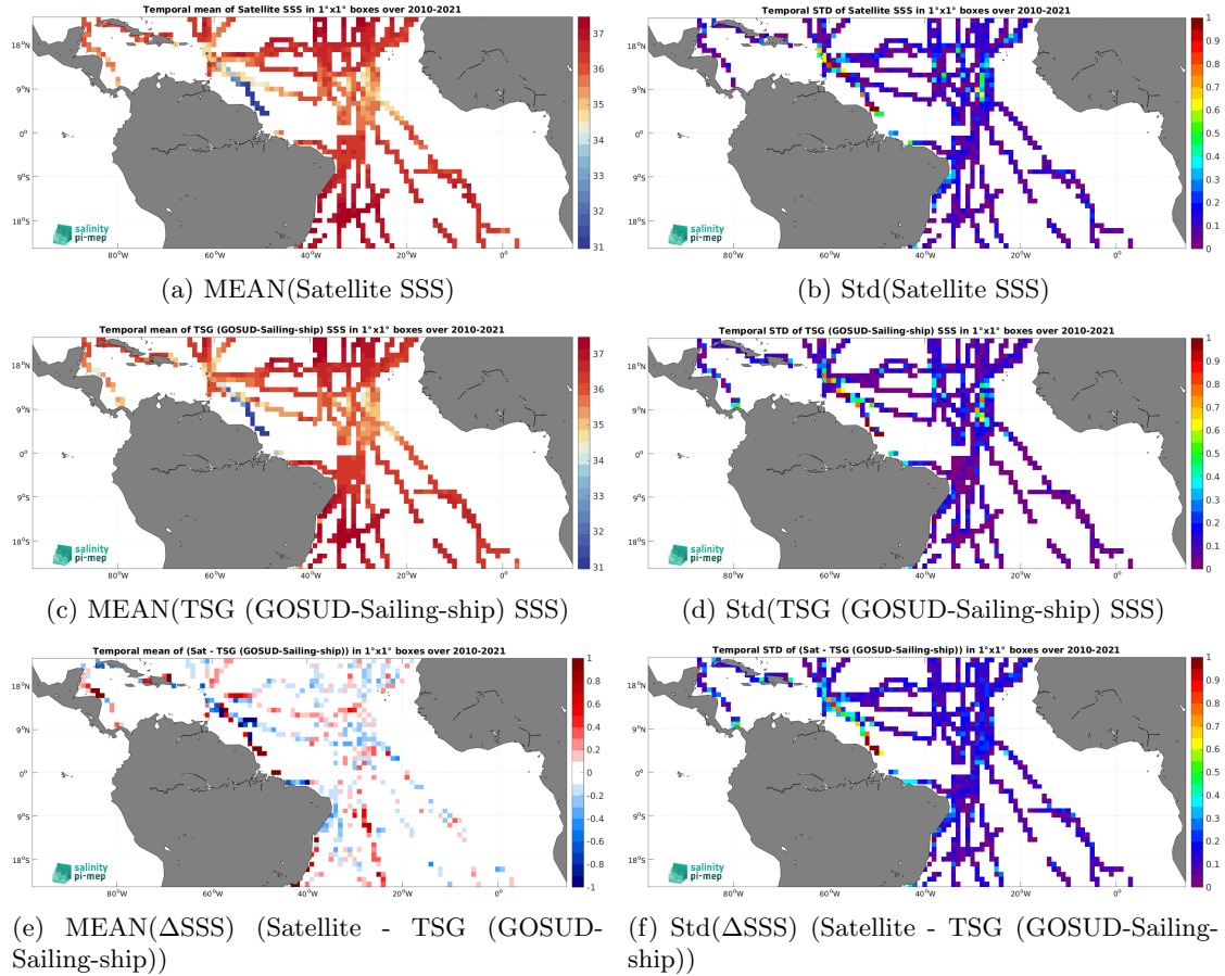
Figure 6: Temporal mean (left) and Std (right) of SSS from SMOS SSS L3 v8 - 9 Days (CATDS-CEC-LOCEAN) (top), TSG (GOSUD-Sailing-ship) (middle), and of \Delta\text{SSS} (Satellite - TSG (GOSUD-Sailing-ship)). Only match-up pairs are used to generate these maps.
