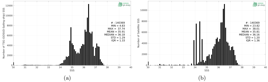
Figure 2: Histograms of SSS from TSG (GOSUD-Sailing-ship) (a) and SMOS SSS L3 v8 - 9 Days (CATDS-CECOS-LOCEAN) (b) considering all match-up pairs per bins of 0.1 over the Tropical Atlantic Ocean Pi-MEP region and for the full satellite product period.
