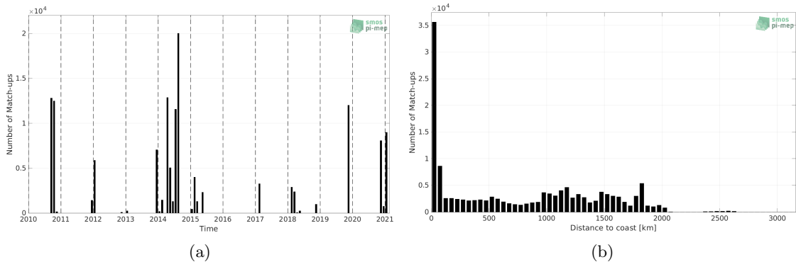
Figure 1: Number of match-ups between TSG (GOSUD-Sailing-ship) and SMOS SSS L3 v8 - 9 Days (CATDS-CECOS-LOCEAN) SSS as a function of time (a) and as function of the distance to coast (b) over the Tropical Atlantic Ocean Pi-MEP region and for the full satellite product period.
