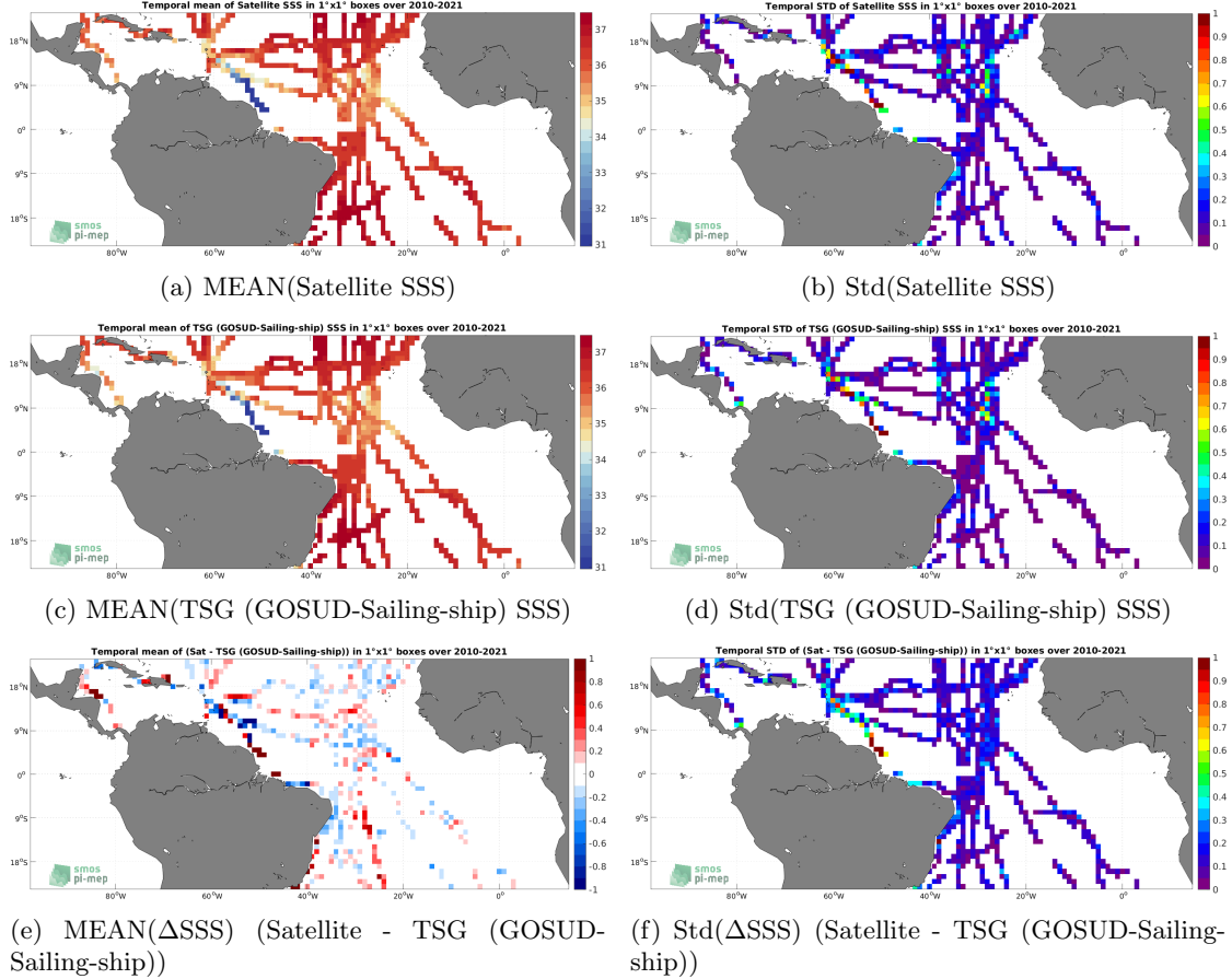
Figure 6: Temporal mean (left) and Std (right) of SSS from SMOS SSS L3 v8 - 9 Days (CATDS-CECOS-LOCEAN) (top), TSG (GOSUD-Sailing-ship) (middle), and of \Delta SSS (Satellite - TSG (GOSUD-Sailing-ship)). Only match-up pairs are used to generate these maps.
