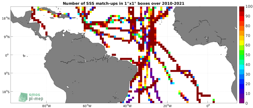
Figure 4: Number of SSS match-ups between TSG (GOSUD-Sailing-ship) SSS and the SMOS SSS L3 v8 - 9 Days (CATDS-CECOS-LOCEAN) SSS product for the Tropical Atlantic Ocean Pi-MEP region over 1^\circ \times 1^\circ boxes and for the full satellite product period.
