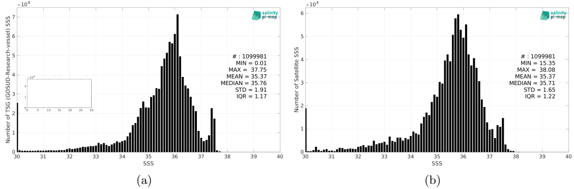
Figure 2: Histograms of SSS from TSG (GOSUD-Research-vessel) (a) and SMOS SSS L3 v8 - 9 Days (CATDS-CEC-LOCEAN) (b) considering all match-up pairs per bins of 0.1 over the Tropical Atlantic Ocean Pi-MEP region and for the full satellite product period.
