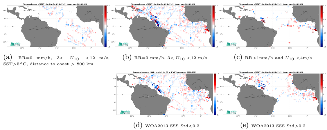
Figure 12: Temporal mean gridded over spatial boxes of size 1^\circ \times 1^\circ of \Delta\text{SSS} (SMOS SSS L3 v8 - 9 Days (CATDS-CEC-LOCEAN) - TSG (GOSUD-Research-vessel)) for 5 different subdatasets corresponding to:RR=0 mm/h, 3 < U_{10} < 12 m/s, SST >5^\circ\text{C} , distance to coast > 800 km (a), RR=0 mm/h, 3 < U_{10} < 12 m/s (b), RR >1 mm/h and U_{10} < 4 m/s (c), WOA2013 SSS Std <0.2 (d), WOA2013 SSS Std >0.2 (e).
