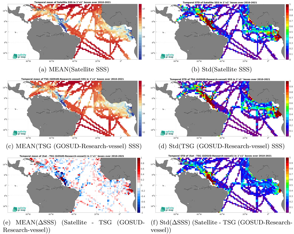
Figure 6: Temporal mean (left) and Std (right) of SSS from SMOS SSS L3 v8 - 9 Days (CATDS-CEC-LOCEAN) (top), TSG (GOSUD-Research-vessel) (middle), and of \Delta\text{SSS} (Satellite - TSG (GOSUD-Research-vessel)). Only match-up pairs are used to generate these maps.
