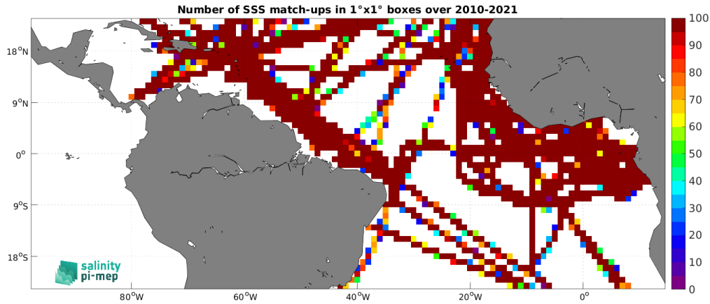
Figure 4: Number of SSS match-ups between TSG (GOSUD-Research-vessel) SSS and the SMOS SSS L3 v8 - 9 Days (CATDS-CEC-LOCEAN) SSS product for the Tropical Atlantic Ocean Pi-MEP region over 1^\circ \times 1^\circ boxes and for the full satellite product period.
