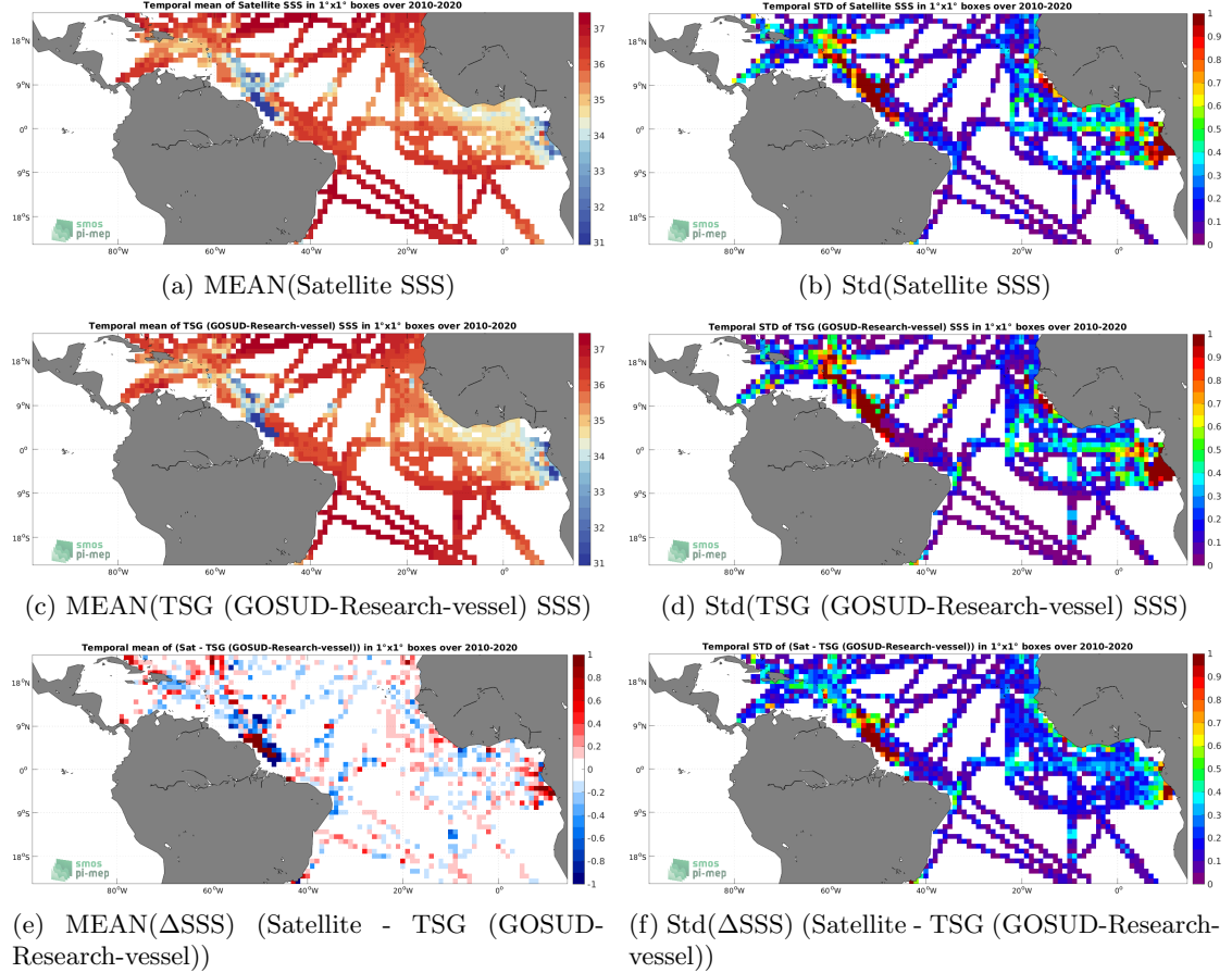
Figure 6: Temporal mean (left) and Std (right) of SSS from SMOS SSS L3 v8 - 9 Days (CATDS-CECOS-LOCEAN) (top), TSG (GOSUD-Research-vessel) (middle), and of \Delta SSS (Satellite - TSG (GOSUD-Research-vessel)). Only match-up pairs are used to generate these maps.
