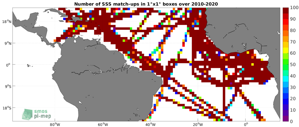
Figure 4: Number of SSS match-ups between TSG (GOSUD-Research-vessel) SSS and the SMOS SSS L3 v8 - 9 Days (CATDS-CECOS-LOCEAN) SSS product for the Tropical Atlantic Ocean Pi-MEP region over 1^\circ \times 1^\circ boxes and for the full satellite product period.
