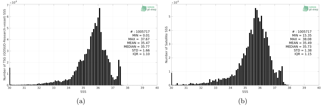
Figure 2: Histograms of SSS from TSG (GOSUD-Research-vessel) (a) and SMOS SSS L3 v8 - 9 Days (CATDS-CECOS-LOCEAN) (b) considering all match-up pairs per bins of 0.1 over the Tropical Atlantic Ocean Pi-MEP region and for the full satellite product period.
