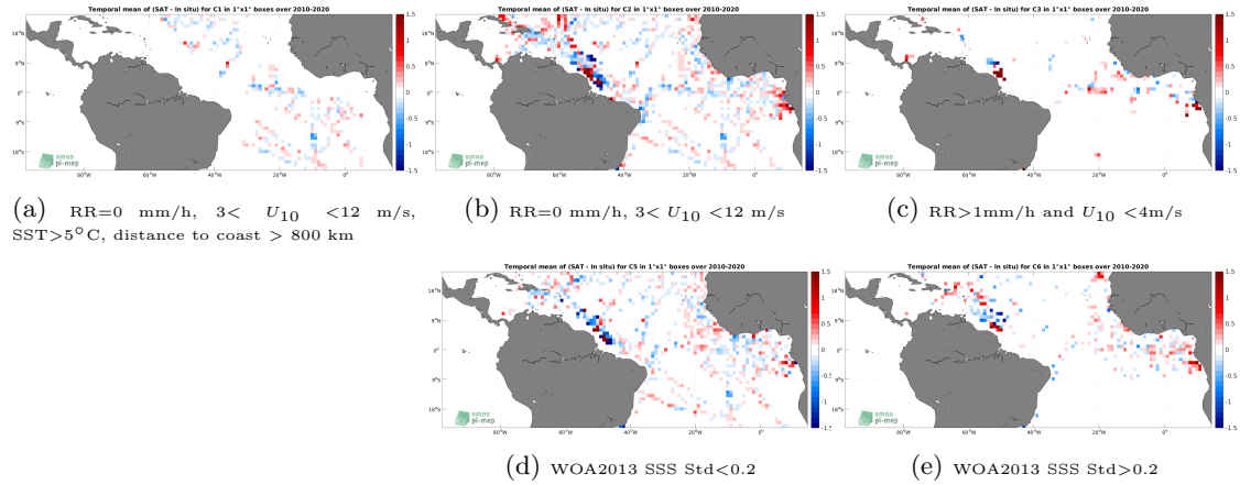
Figure 12: Temporal mean gridded over spatial boxes of size 1^{\circ}\times 1^{\circ} of \Delta SSS (SMOS SSS L3 v8 - 9 Days (CATDS-CECOS-LOCEAN) - TSG (GOSUD-Research-vessel)) for 5 different subdatasets corresponding to:RR=0 mm/h, 3 < U_{10} < 12 m/s, SST >5^{\circ}\text{C} , distance to coast > 800 km (a), RR=0 mm/h, 3 < U_{10} < 12 m/s (b), RR >1 mm/h and U_{10} < 4 m/s (c), WOA2013 SSS Std <0.2 (d), WOA2013 SSS Std >0.2 (e).
