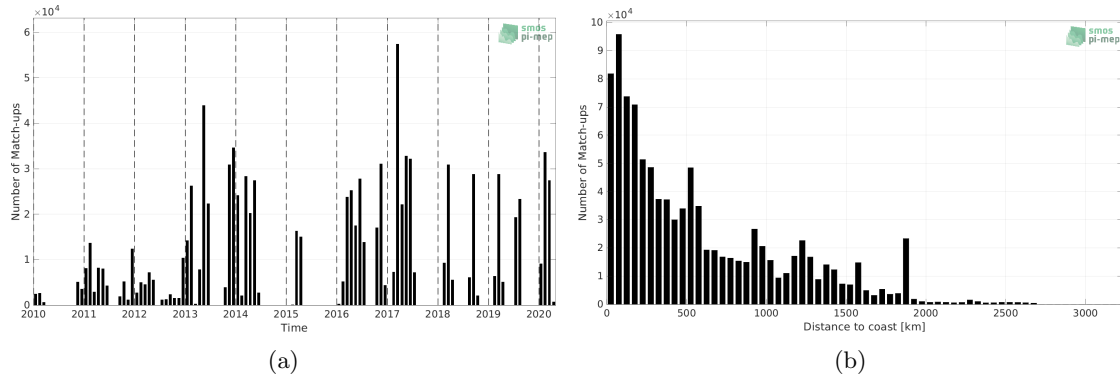
Figure 1: Number of match-ups between TSG (GOSUD-Research-vessel) and SMOS SSS L3 v8 - 9 Days (CATDS-CECOS-LOCEAN) SSS as a function of time (a) and as function of the distance to coast (b) over the Tropical Atlantic Ocean Pi-MEP region and for the full satellite product period.
