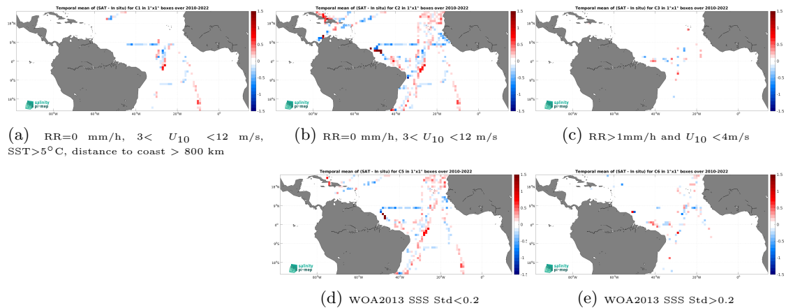
Figure 12: Temporal mean gridded over spatial boxes of size 1^\circ \times 1^\circ of \Delta\text{SSS} (SMOS SSS L3 v8 - 9 Days (CATDS-CEC-LOCEAN) - TSG (CSIC-UTM)) for 5 different subdatasets corresponding to:RR=0 mm/h, 3 < U_{10} < 12 m/s, SST >5^\circ\text{C} , distance to coast > 800 km (a), RR=0 mm/h, 3 < U_{10} < 12 m/s (b), RR >1 mm/h and U_{10} < 4 m/s (c), WOA2013 SSS Std <0.2 (d), WOA2013 SSS Std >0.2 (e).
