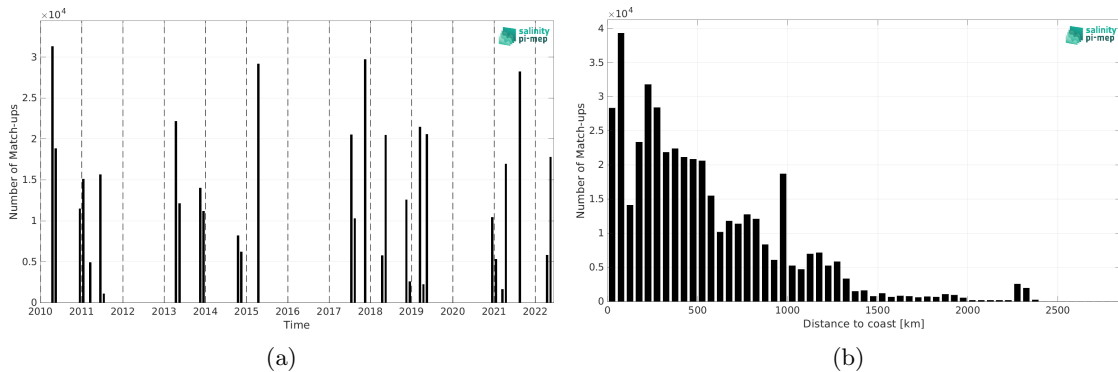
Figure 1: Number of match-ups between TSG (CSIC-UTM) and SMOS SSS L3 v8 - 9 Days (CATDS-CEC-LOCEAN) SSS as a function of time (a) and as function of the distance to coast (b) over the Tropical Atlantic Ocean Pi-MEP region and for the full satellite product period.
