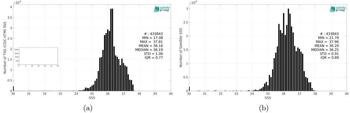
Figure 2: Histograms of SSS from TSG (CSIC-UTM) (a) and SMOS SSS L3 v8 - 9 Days (CATDS-CEC-LOCEAN) (b) considering all match-up pairs per bins of 0.1 over the Tropical Atlantic Ocean Pi-MEP region and for the full satellite product period.
