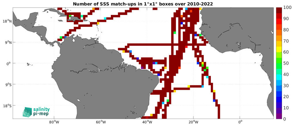
Figure 4: Number of SSS match-ups between TSG (CSIC-UTM) SSS and the SMOS SSS L3 v8 - 9 Days (CATDS-CEC-LOCEAN) SSS product for the Tropical Atlantic Ocean Pi-MEP region over 1^\circ \times 1^\circ boxes and for the full satellite product period.
