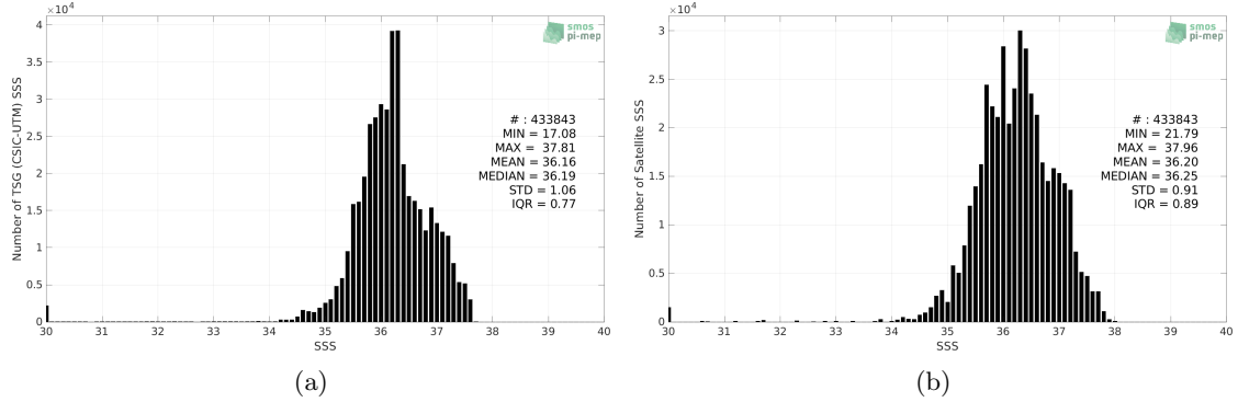
Figure 2: Histograms of SSS from TSG (CSIC-UTM) (a) and SMOS SSS L3 v8 - 9 Days (CATDS-CECOS-LOCEAN) (b) considering all match-up pairs per bins of 0.1 over the Tropical Atlantic Ocean Pi-MEP region and for the full satellite product period.
