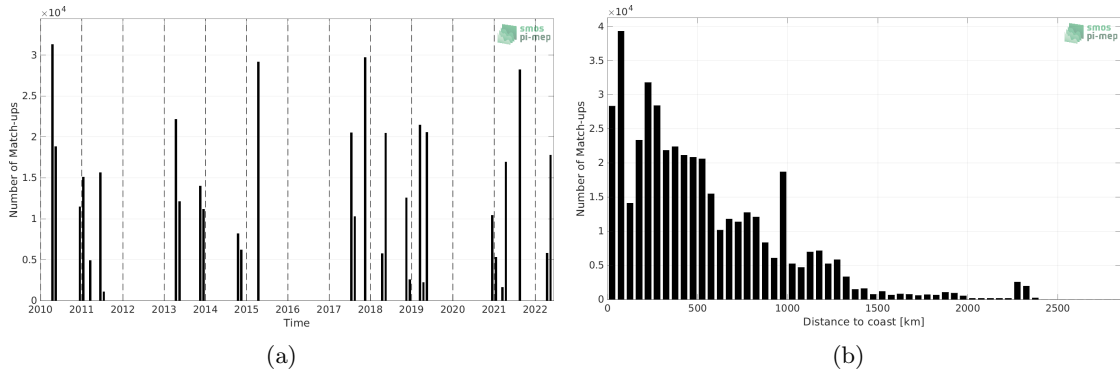
Figure 1: Number of match-ups between TSG (CSIC-UTM) and SMOS SSS L3 v8 - 9 Days (CATDS-CECOS-LOCEAN) SSS as a function of time (a) and as function of the distance to coast (b) over the Tropical Atlantic Ocean Pi-MEP region and for the full satellite product period.
