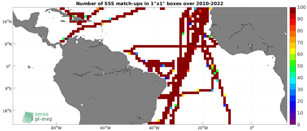
Figure 4: Number of SSS match-ups between TSG (CSIC-UTM) SSS and the SMOS SSS L3 v8 - 9 Days (CATDS-CECOS-LOCEAN) SSS product for the Tropical Atlantic Ocean Pi-MEP region over 1^\circ \times 1^\circ boxes and for the full satellite product period.
