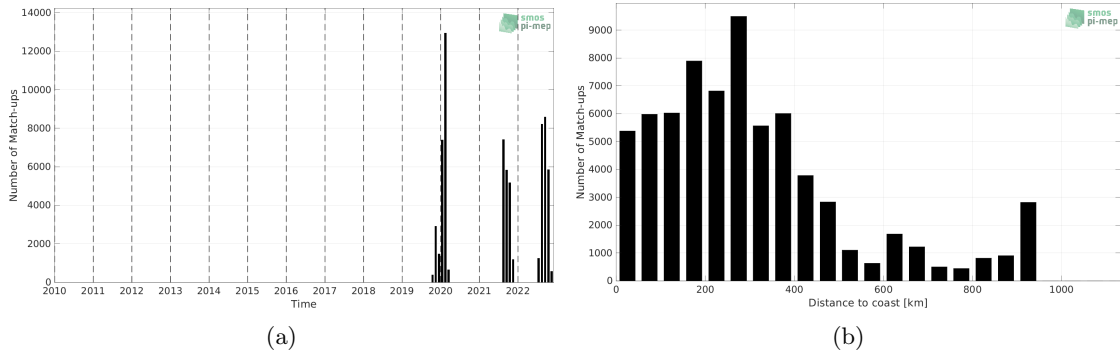
Figure 1: Number of match-ups between Saildrone and SMOS SSS L3 v8 - 9 Days (CATDS-CECOS-LOCEAN) SSS as a function of time (a) and as function of the distance to coast (b) over the Tropical Atlantic Ocean Pi-MEP region and for the full satellite product period.
