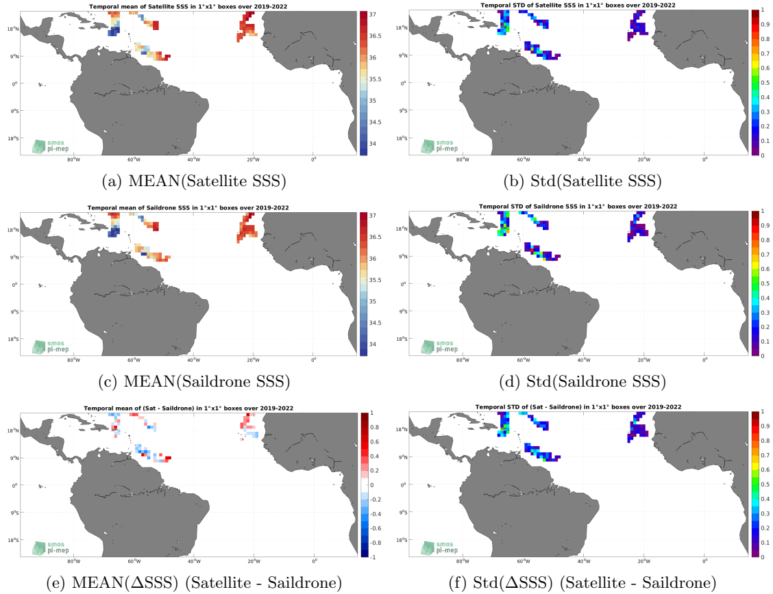
Figure 6: Temporal mean (left) and Std (right) of SSS from SMOS SSS L3 v8 - 9 Days (CATDS-CECOS-LOCEAN) (top), Saildrone (middle), and of \Delta\text{SSS} (Satellite - Saildrone). Only match-up pairs are used to generate these maps.
