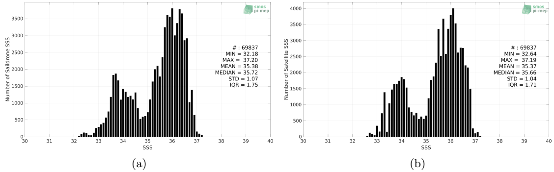
Figure 2: Histograms of SSS from Saildrone (a) and SMOS SSS L3 v8 - 9 Days (CATDS-CECOS-LOCEAN) (b) considering all match-up pairs per bins of 0.1 over the Tropical Atlantic Ocean Pi-MEP region and for the full satellite product period.
