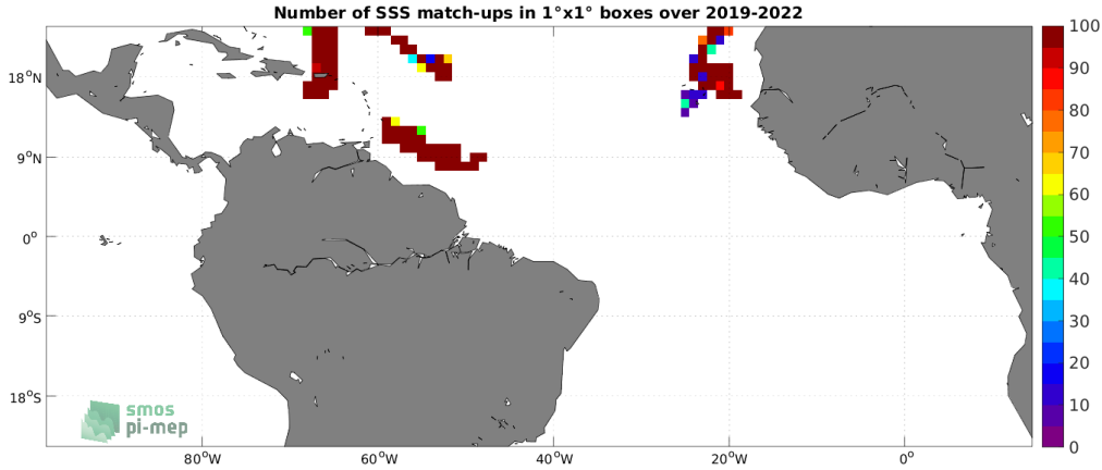
Figure 4: Number of SSS match-ups between Saildrone SSS and the SMOS SSS L3 v8 - 9 Days (CATDS-CECOS-LOCEAN) SSS product for the Tropical Atlantic Ocean Pi-MEP region over 1^\circ \times 1^\circ boxes and for the full satellite product period.
