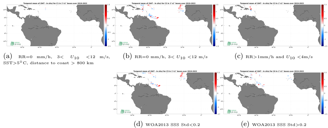
Figure 12: Temporal mean gridded over spatial boxes of size 1^\circ \times 1^\circ of \Delta SSS (SMOS SSS L3 v8 - 9 Days (CATDS-CECOS-LOCEAN) - Saildrone) for 5 different subdatasets corresponding to:RR=0 mm/h, 3 < U_{10} < 12 m/s, SST >5^\circ\text{C} , distance to coast > 800 km (a), RR=0 mm/h, 3 < U_{10} < 12 m/s (b), RR >1 mm/h and U_{10} < 4 m/s (c), WOA2013 SSS Std <0.2 (d), WOA2013 SSS Std >0.2 (e).
