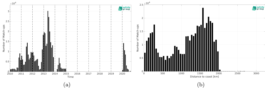
Figure 1: Number of match-ups between Surface drifters and SMOS SSS L3 v8 - 9 Days (CATDS-CEC-LOCEAN) SSS as a function of time (a) and as function of the distance to coast (b) over the Tropical Atlantic Ocean Pi-MEP region and for the full satellite product period.
