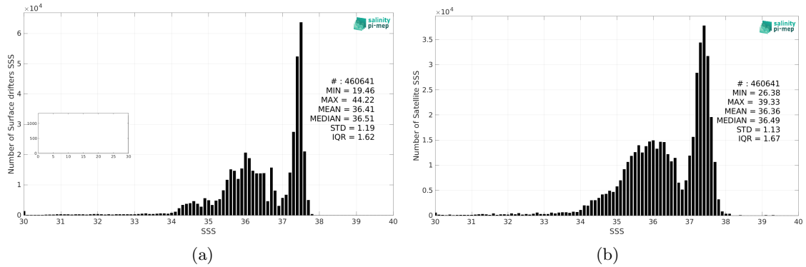
Figure 2: Histograms of SSS from Surface drifters (a) and SMOS SSS L3 v8 - 9 Days (CATDS-CEC-LOCEAN) (b) considering all match-up pairs per bins of 0.1 over the Tropical Atlantic Ocean Pi-MEP region and for the full satellite product period.
