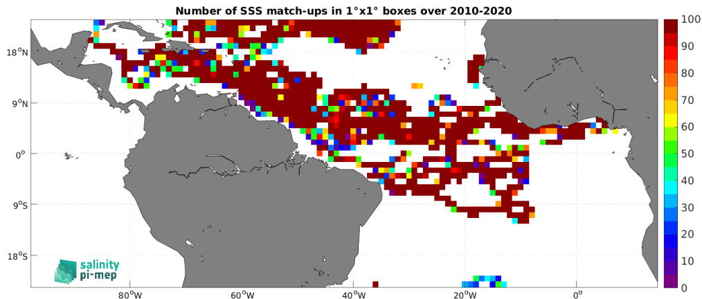
Figure 3: Number of SSS match-ups between Surface drifters SSS and the SMOS SSS L3 v8 - 9 Days (CATDS-CEC-LOCEAN) SSS product for the Tropical Atlantic Ocean Pi-MEP region over 1^\circ \times 1^\circ boxes and for the full satellite product period.
