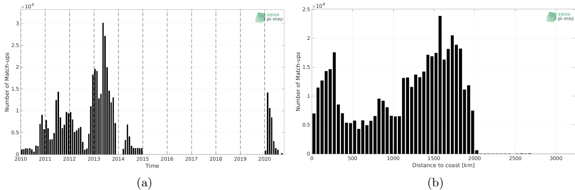
Figure 1: Number of match-ups between Surface drifters and SMOS SSS L3 v8 - 9 Days (CATDS-CECOS-LOCEAN) SSS as a function of time (a) and as function of the distance to coast (b) over the Tropical Atlantic Ocean Pi-MEP region and for the full satellite product period.
