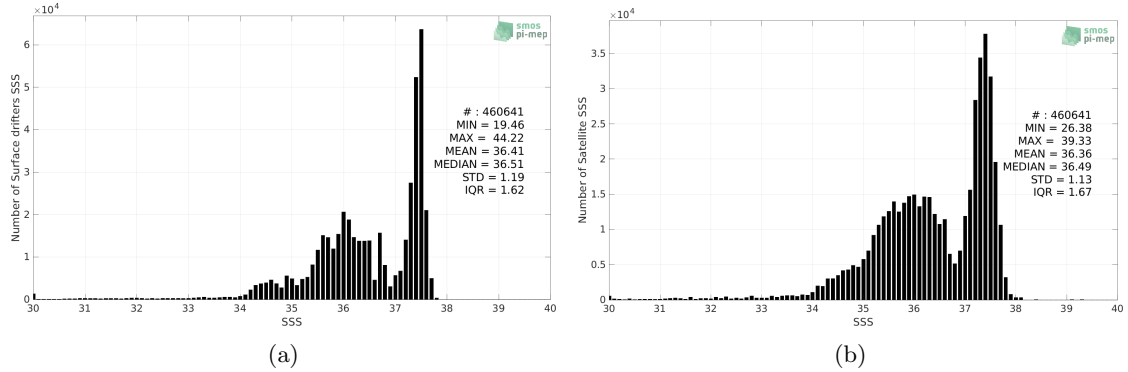
Figure 2: Histograms of SSS from Surface drifters (a) and SMOS SSS L3 v8 - 9 Days (CATDS-CECOS-LOCEAN) (b) considering all match-up pairs per bins of 0.1 over the Tropical Atlantic Ocean Pi-MEP region and for the full satellite product period.
