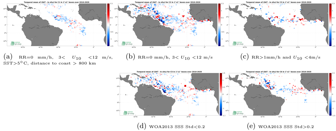
Figure 11: Temporal mean gridded over spatial boxes of size 1^{\circ}\times 1^{\circ} of \Delta\text{SSS} (SMOS SSS L3 v8 - 9 Days (CATDS-CECOS-LOCEAN) - Surface drifters) for 5 different subdatasets corresponding to:RR=0 mm/h, 3 < U_{10} < 12 m/s, SST > 5^{\circ}\text{C} , distance to coast > 800 km (a), RR=0 mm/h, 3 < U_{10} < 12 m/s (b), RR > 1 mm/h and U_{10} < 4 m/s (c), WOA2013 SSS Std < 0.2 (d), WOA2013 SSS Std > 0.2 (e).
