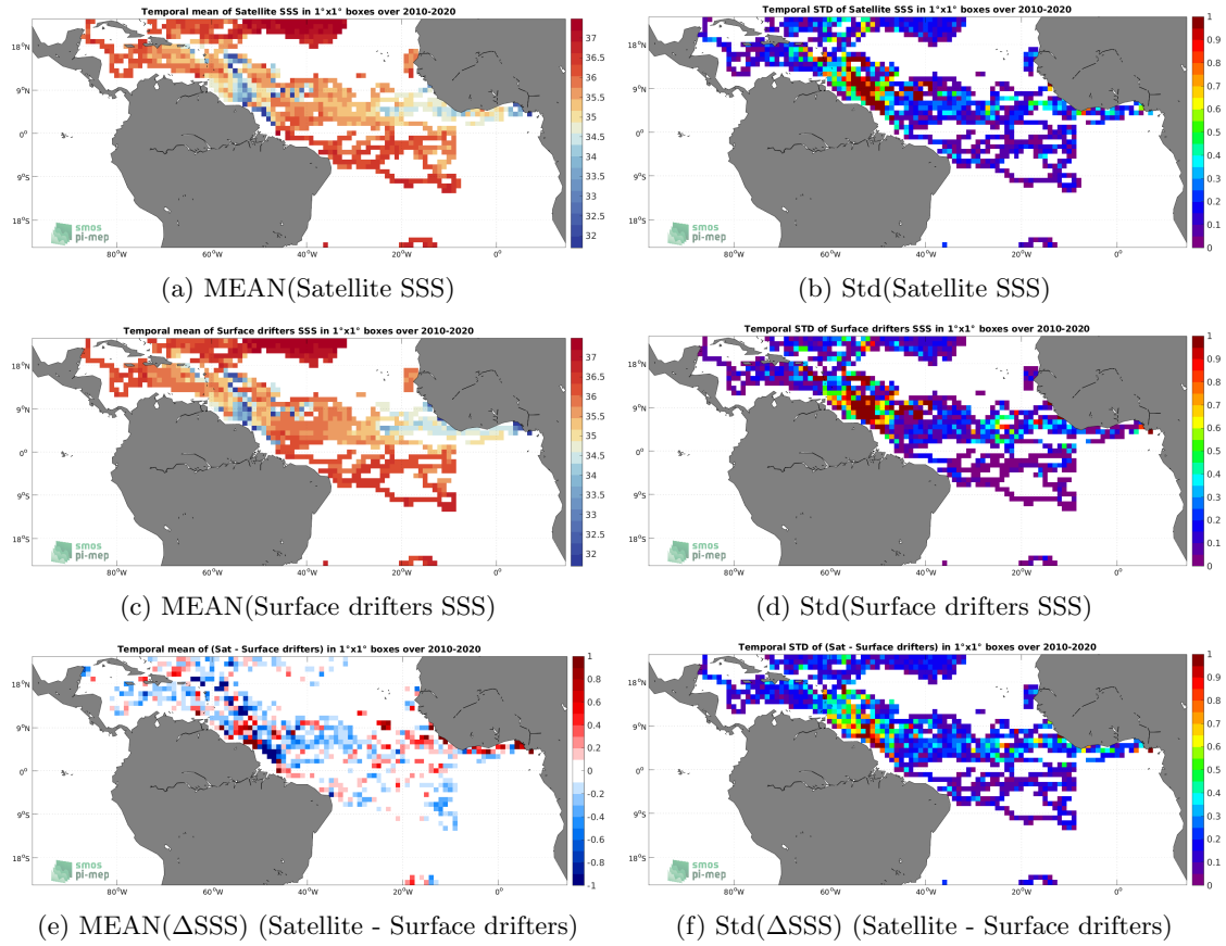
Figure 5: Temporal mean (left) and Std (right) of SSS from SMOS SSS L3 v8 - 9 Days (CATDS-CECOS-LOCEAN) (top), Surface drifters (middle), and of \Delta SSS (Satellite - Surface drifters). Only match-up pairs are used to generate these maps.
