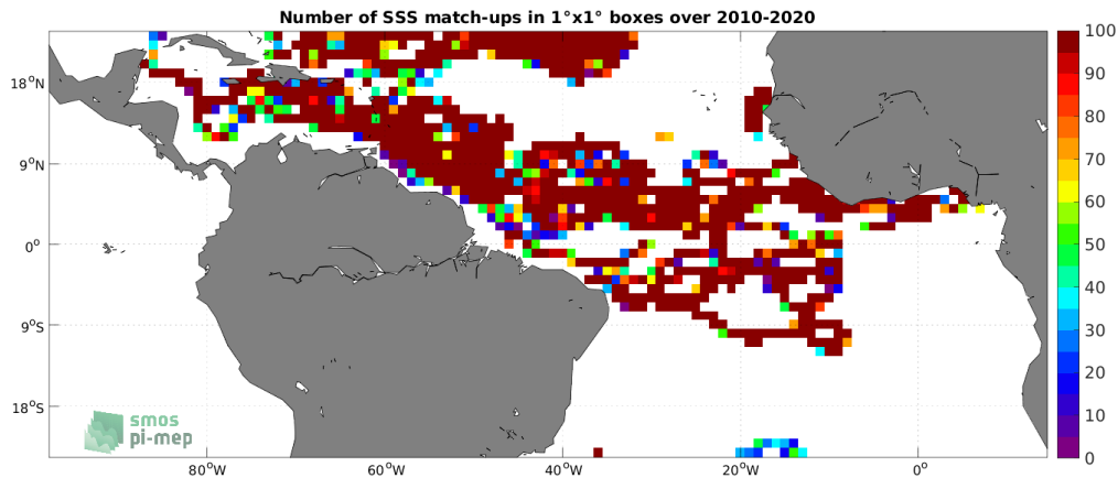
Figure 3: Number of SSS match-ups between Surface drifters SSS and the SMOS SSS L3 v8 - 9 Days (CATDS-CECOS-LOCEAN) SSS product for the Tropical Atlantic Ocean Pi-MEP region over 1^\circ \times 1^\circ boxes and for the full satellite product period.
