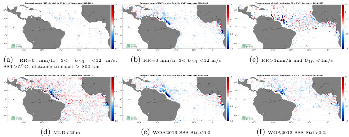
Figure 12: Temporal mean gridded over spatial boxes of size 1^\circ \times 1^\circ of \Delta SSS (SMOS SSS L3 v8 - 9 Days (CATDS-CECOS-LOCEAN) - Argo) for 6 different subdatasets corresponding to:RR=0 mm/h, 3 < U_{10} < 12 m/s, SST >5^\circ C, distance to coast > 800 km (a), RR=0 mm/h, 3 < U_{10} < 12 m/s (b), RR >1 mm/h and U_{10} < 4 m/s (c),MLD <20 m (d),WOA2013 SSS Std <0.2 (e),WOA2013 SSS Std >0.2 (f).
