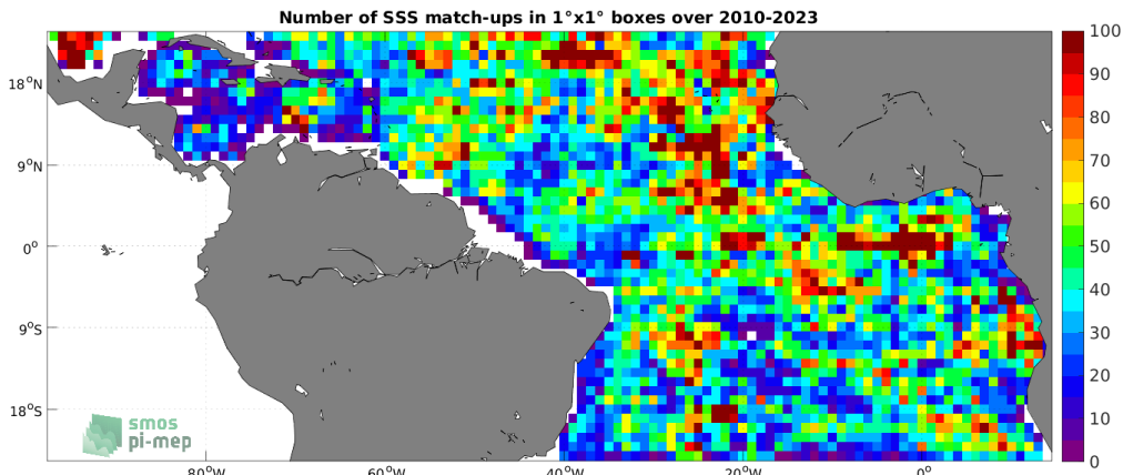
Figure 4: Number of SSS match-ups between Argo SSS and the SMOS SSS L3 v8 - 9 Days (CATDS-CECOS-LOCEAN) SSS product for the Tropical Atlantic Ocean Pi-MEP region over 1^\circ \times 1^\circ boxes and for the full satellite product period.
