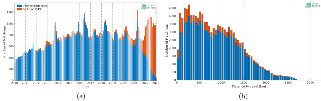
Figure 1: Number of match-ups between Argo and SMOS SSS L3 v8 - 9 Days (CATDS-CECOS-LOCEAN) SSS as a function of time (a) and as function of the distance to coast (b) over the Tropical Atlantic Ocean Pi-MEP region and for the full satellite product period.
