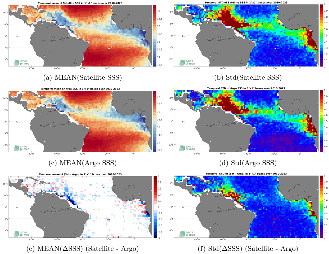
Figure 6: Temporal mean (left) and Std (right) of SSS from SMOS SSS L3 v8 - 9 Days (CATDS-CECOS-LOCEAN) (top), Argo (middle), and of \Delta SSS (Satellite - Argo). Only match-up pairs are used to generate these maps.
