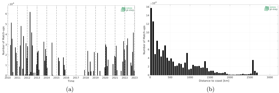
Figure 1: Number of match-ups between TSG (SAMOS) and SMOS SSS L3 v8 - 18 Days (CATDS-CECOS-LOCEAN) SSS as a function of time (a) and as function of the distance to coast (b) over the Tropical Atlantic Ocean Pi-MEP region and for the full satellite product period.
