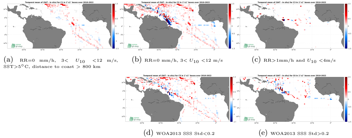
Figure 12: Temporal mean gridded over spatial boxes of size 1^{\circ}\times 1^{\circ} of \Delta\text{SSS} (SMOS SSS L3 v8 - 18 Days (CATDS-CECOS-LOCEAN) - TSG (SAMOS)) for 5 different subdatasets corresponding to:RR=0 mm/h, 3 < U_{10} < 12 m/s, SST > 5^{\circ}\text{C} , distance to coast > 800 km (a), RR=0 mm/h, 3 < U_{10} < 12 m/s (b), RR > 1 mm/h and U_{10} < 4 m/s (c), WOA2013 SSS Std < 0.2 (d), WOA2013 SSS Std > 0.2 (e).
