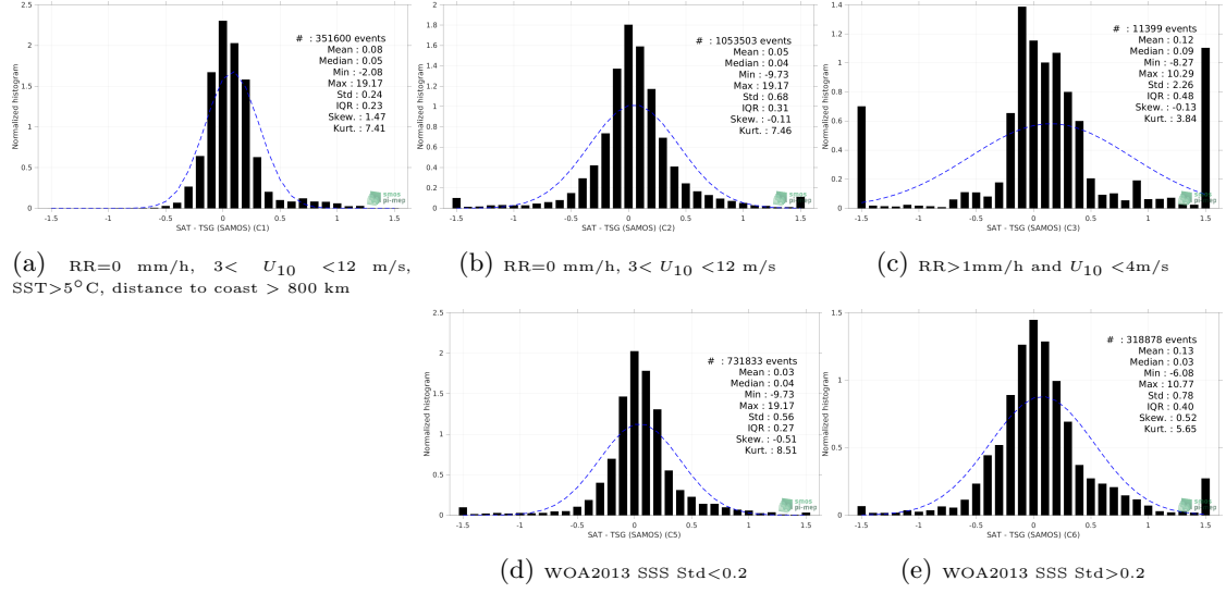
Figure 13: Normalized histogram of \Delta\text{SSS} (SMOS SSS L3 v8 - 18 Days (CATDS-CECOS-LOCEAN) - TSG (SAMOS)) for 5 different subdatasets corresponding to: RR=0 mm/h, 3 < U_{10} < 12 m/s, SST > 5^\circ\text{C} , distance to coast > 800 km (a), RR=0 mm/h, 3 < U_{10} < 12 m/s (b), RR > 1 mm/h and U_{10} < 4 m/s (c), WOA2013 SSS Std < 0.2 (d), WOA2013 SSS Std > 0.2 (e).
