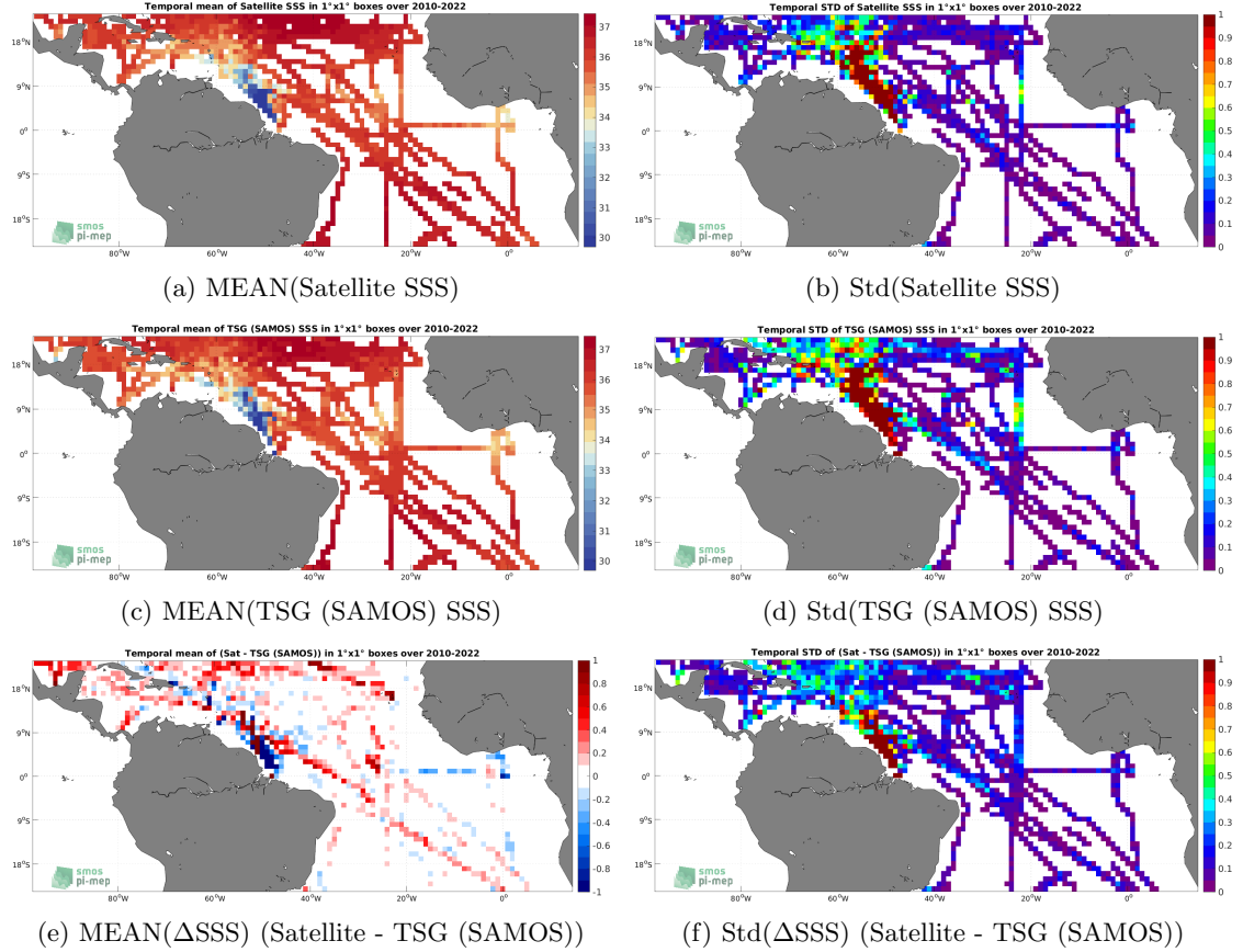
Figure 6: Temporal mean (left) and Std (right) of SSS from SMOS SSS L3 v8 - 18 Days (CATDS-CECOS-LOCEAN) (top), TSG (SAMOS) (middle), and of \Delta\text{SSS} (Satellite - TSG (SAMOS)). Only match-up pairs are used to generate these maps.
