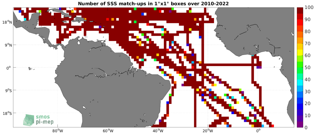
Figure 4: Number of SSS match-ups between TSG (SAMOS) SSS and the SMOS SSS L3 v8 - 18 Days (CATDS-CECOS-LOCEAN) SSS product for the Tropical Atlantic Ocean Pi-MEP region over 1^\circ \times 1^\circ boxes and for the full satellite product period.
