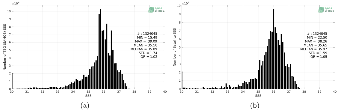
Figure 2: Histograms of SSS from TSG (SAMOS) (a) and SMOS SSS L3 v8 - 18 Days (CATDS-CECOS-LOCEAN) (b) considering all match-up pairs per bins of 0.1 over the Tropical Atlantic Ocean Pi-MEP region and for the full satellite product period.
