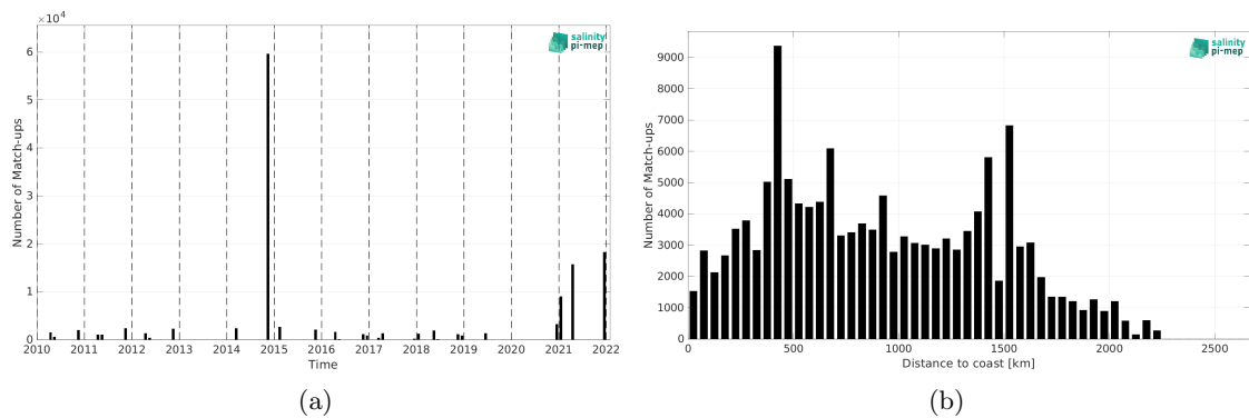
Figure 1: Number of match-ups between TSG (Polarstern) and SMOS SSS L3 v8 - 18 Days (CATDS-CEC-LOCEAN) SSS as a function of time (a) and as function of the distance to coast (b) over the Tropical Atlantic Ocean Pi-MEP region and for the full satellite product period.
