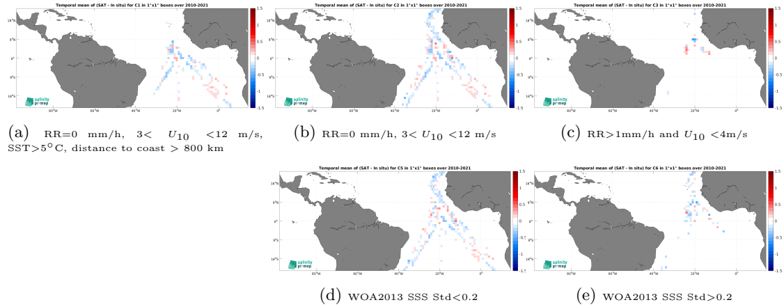
Figure 12: Temporal mean gridded over spatial boxes of size 1^{\circ}\times 1^{\circ} of \Delta\text{SSS} (SMOS SSS L3 v8 - 18 Days (CATDS-CEC-LOCEAN) - TSG (Polarstern)) for 5 different subdatasets corresponding to:RR=0 mm/h, 3 < U_{10} < 12 m/s, SST > 5^{\circ}\text{C} , distance to coast > 800 km (a), RR=0 mm/h, 3 < U_{10} < 12 m/s (b), RR > 1 mm/h and U_{10} < 4 m/s (c), WOA2013 SSS Std < 0.2 (d), WOA2013 SSS Std > 0.2 (e).
