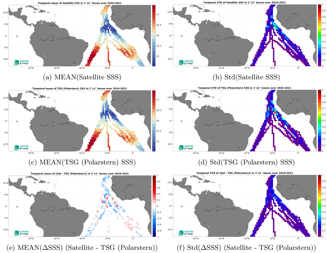
Figure 6: Temporal mean (left) and Std (right) of SSS from SMOS SSS L3 v8 - 18 Days (CATDS-CEC-LOCEAN) (top), TSG (Polarstern) (middle), and of \Delta SSS (Satellite - TSG (Polarstern)). Only match-up pairs are used to generate these maps.
