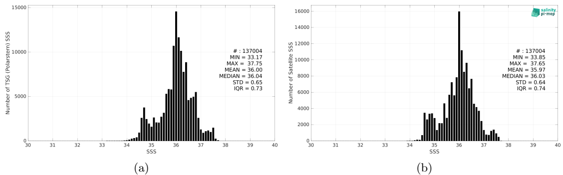
Figure 2: Histograms of SSS from TSG (Polarstern) (a) and SMOS SSS L3 v8 - 18 Days (CATDS-CEC-LOCEAN) (b) considering all match-up pairs per bins of 0.1 over the Tropical Atlantic Ocean Pi-MEP region and for the full satellite product period.
