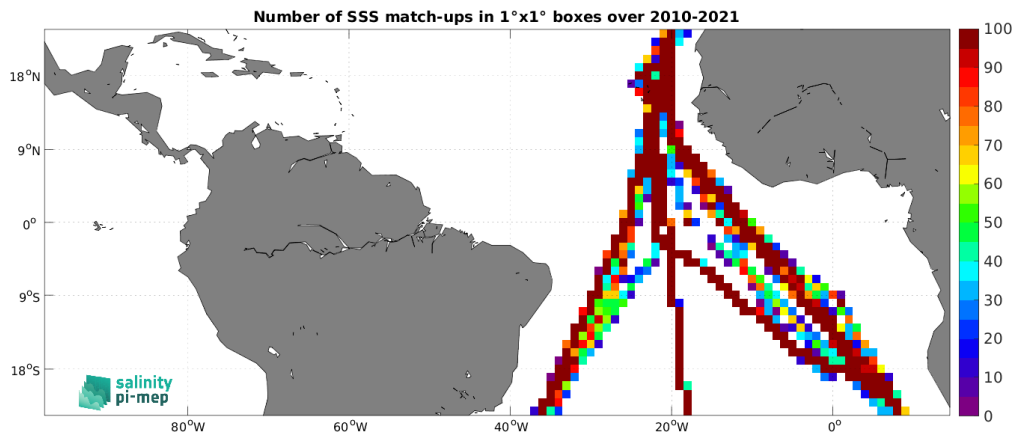
Figure 4: Number of SSS match-ups between TSG (Polarstern) SSS and the SMOS SSS L3 v8 - 18 Days (CATDS-CEC-LOCEAN) SSS product for the Tropical Atlantic Ocean Pi-MEP region over 1^\circ \times 1^\circ boxes and for the full satellite product period.
