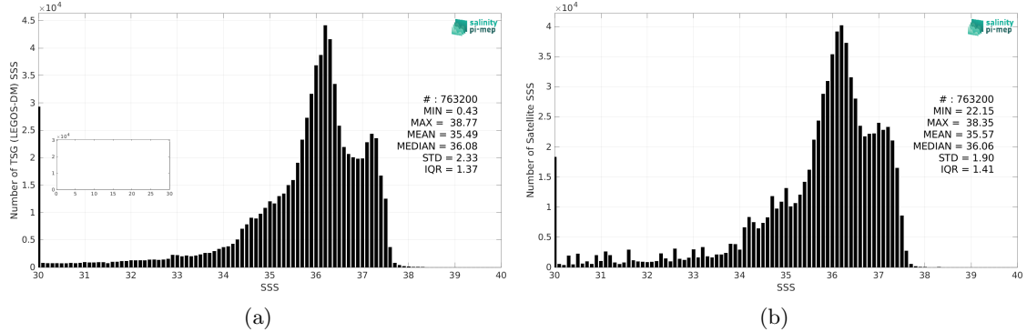
Figure 2: Histograms of SSS from TSG (LEGOS-DM) (a) and SMOS SSS L3 v8 - 18 Days (CATDS-CEC-LOCEAN) (b) considering all match-up pairs per bins of 0.1 over the Tropical Atlantic Ocean Pi-MEP region and for the full satellite product period.
