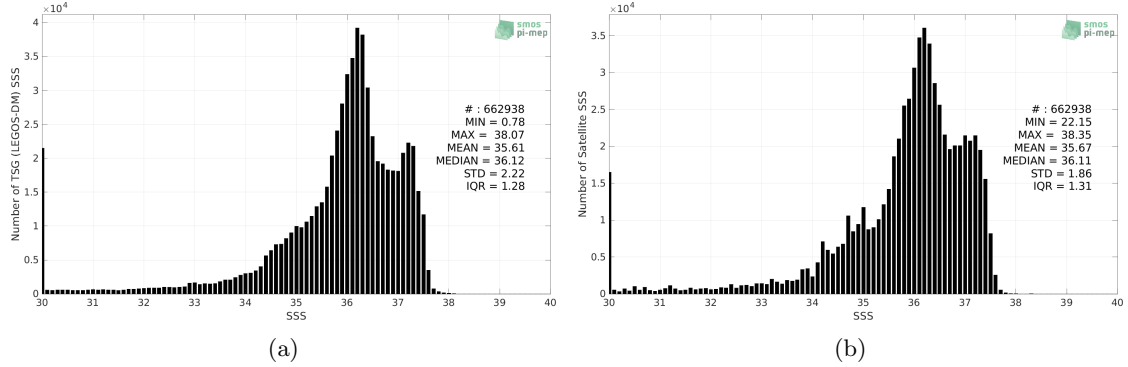
Figure 2: Histograms of SSS from TSG (LEGOS-DM) (a) and SMOS SSS L3 v8 - 18 Days (CATDS-CECOS-LOCEAN) (b) considering all match-up pairs per bins of 0.1 over the Tropical Atlantic Ocean Pi-MEP region and for the full satellite product period.
