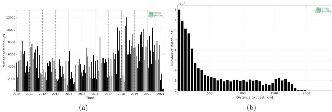
Figure 1: Number of match-ups between TSG (LEGOS-DM) and SMOS SSS L3 v8 - 18 Days (CATDS-CECOS-LOCEAN) SSS as a function of time (a) and as function of the distance to coast (b) over the Tropical Atlantic Ocean Pi-MEP region and for the full satellite product period.
