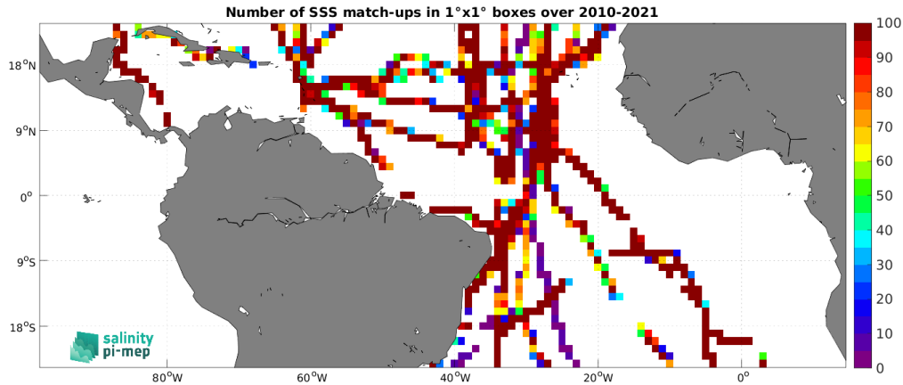
Figure 4: Number of SSS match-ups between TSG (GOSUD-Sailing-ship) SSS and the SMOS SSS L3 v8 - 18 Days (CATDS-CEC-LOCEAN) SSS product for the Tropical Atlantic Ocean Pi-MEP region over 1^\circ \times 1^\circ boxes and for the full satellite product period.
