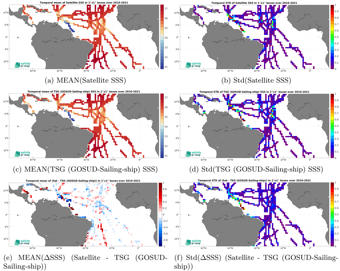
Figure 6: Temporal mean (left) and Std (right) of SSS from SMOS SSS L3 v8 - 18 Days (CATDS-CEC-LOCEAN) (top), TSG (GOSUD-Sailing-ship) (middle), and of \Delta\text{SSS} (Satellite - TSG (GOSUD-Sailing-ship)). Only match-up pairs are used to generate these maps.
