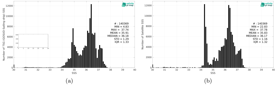
Figure 2: Histograms of SSS from TSG (GOSUD-Sailing-ship) (a) and SMOS SSS L3 v8 - 18 Days (CATDS-CEC-LOCEAN) (b) considering all match-up pairs per bins of 0.1 over the Tropical Atlantic Ocean Pi-MEP region and for the full satellite product period.
