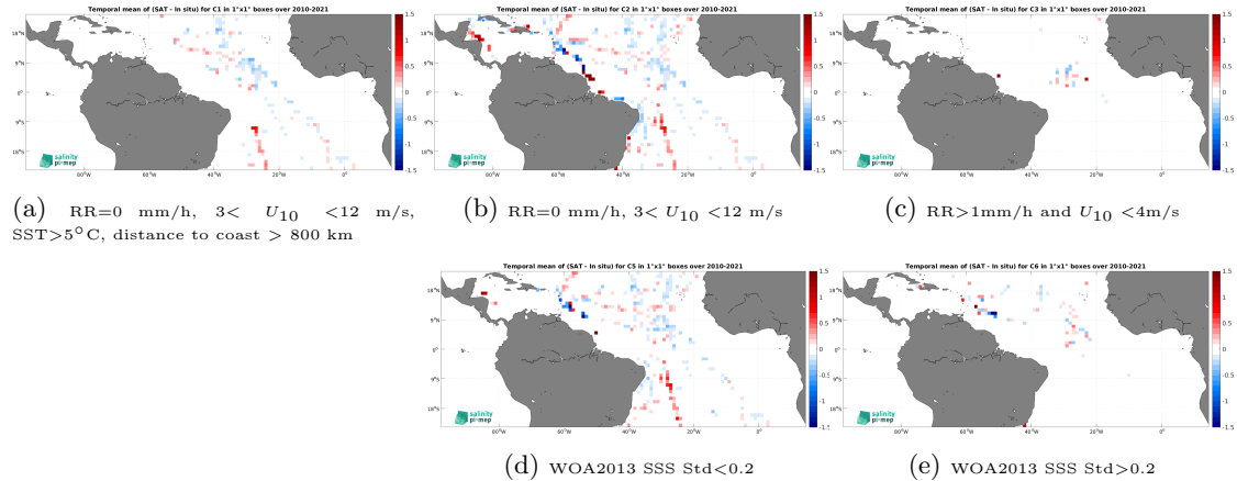
Figure 12: Temporal mean gridded over spatial boxes of size 1^{\circ}\times 1^{\circ} of \Delta SSS (SMOS SSS L3 v8 - 18 Days (CATDS-CEC-LOCEAN) - TSG (GOSUD-Sailing-ship)) for 5 different subdatasets corresponding to:RR=0 mm/h, 3 < U_{10} < 12 m/s, SST >5^{\circ}\text{C} , distance to coast > 800 km (a), RR=0 mm/h, 3 < U_{10} < 12 m/s (b), RR >1 mm/h and U_{10} < 4 m/s (c), WOA2013 SSS Std <0.2 (d), WOA2013 SSS Std >0.2 (e).
