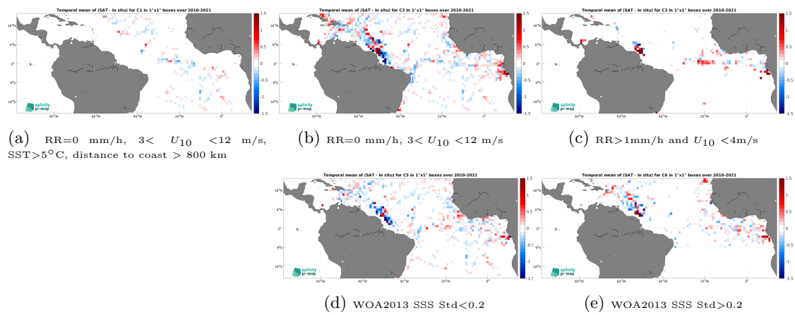
Figure 12: Temporal mean gridded over spatial boxes of size 1^\circ \times 1^\circ of \Delta\text{SSS} (SMOS SSS L3 v8 - 18 Days (CATDS-CEC-LOCEAN) - TSG (GOSUD-Research-vessel)) for 5 different subdatasets corresponding to:RR=0 mm/h, 3 < U_{10} < 12 m/s, SST >5^\circ\text{C} , distance to coast > 800 km (a), RR=0 mm/h, 3 < U_{10} < 12 m/s (b), RR >1 mm/h and U_{10} < 4 m/s (c), WOA2013 SSS Std <0.2 (d), WOA2013 SSS Std >0.2 (e).
