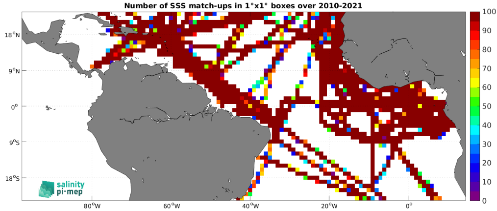
Figure 4: Number of SSS match-ups between TSG (GOSUD-Research-vessel) SSS and the SMOS SSS L3 v8 - 18 Days (CATDS-CEC-LOCEAN) SSS product for the Tropical Atlantic Ocean Pi-MEP region over 1^\circ \times 1^\circ boxes and for the full satellite product period.
