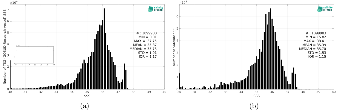
Figure 2: Histograms of SSS from TSG (GOSUD-Research-vessel) (a) and SMOS SSS L3 v8 - 18 Days (CATDS-CEC-LOCEAN) (b) considering all match-up pairs per bins of 0.1 over the Tropical Atlantic Ocean Pi-MEP region and for the full satellite product period.
