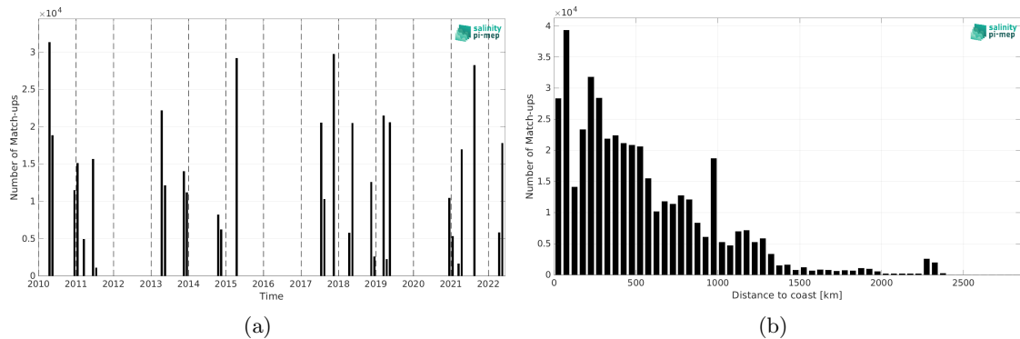
Figure 1: Number of match-ups between TSG (CSIC-UTM) and SMOS SSS L3 v8 - 18 Days (CATDS-CEC-LOCEAN) SSS as a function of time (a) and as function of the distance to coast (b) over the Tropical Atlantic Ocean Pi-MEP region and for the full satellite product period.
