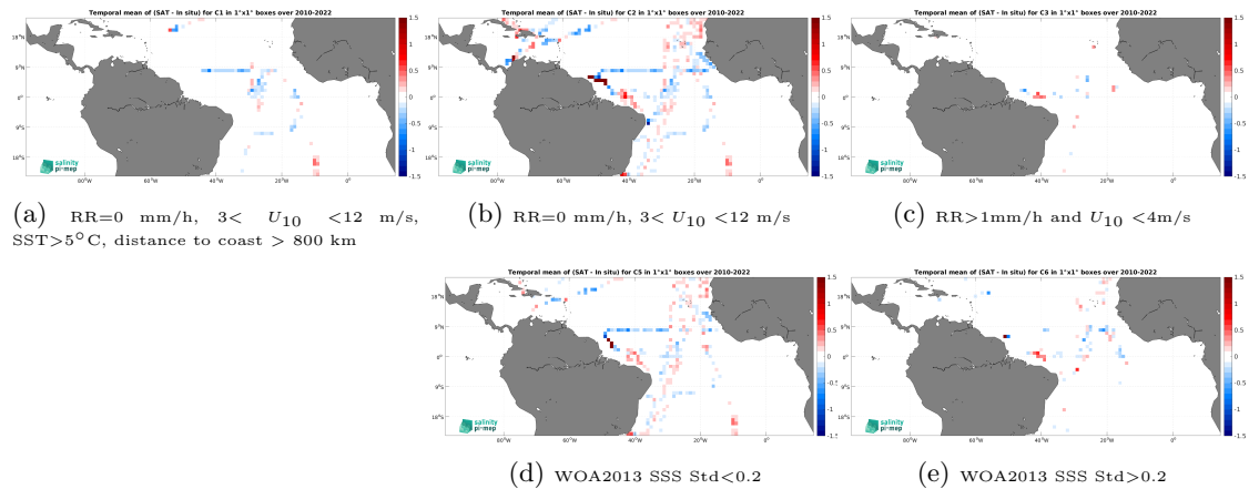
Figure 12: Temporal mean gridded over spatial boxes of size 1^\circ \times 1^\circ of \Delta SSS (SMOS SSS L3 v8 - 18 Days (CATDS-CEC-LOCEAN) - TSG (CSIC-UTM)) for 5 different subdatasets corresponding to:RR=0 mm/h, 3 < U_{10} < 12 m/s, SST >5^\circ\text{C} , distance to coast > 800 km (a), RR=0 mm/h, 3 < U_{10} < 12 m/s (b), RR >1 mm/h and U_{10} < 4 m/s (c), WOA2013 SSS Std <0.2 (d), WOA2013 SSS Std >0.2 (e).
