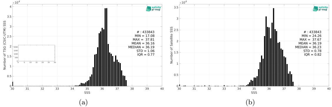
Figure 2: Histograms of SSS from TSG (CSIC-UTM) (a) and SMOS SSS L3 v8 - 18 Days (CATDS-CEC-LOCEAN) (b) considering all match-up pairs per bins of 0.1 over the Tropical Atlantic Ocean Pi-MEP region and for the full satellite product period.
