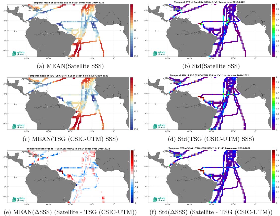
Figure 6: Temporal mean (left) and Std (right) of SSS from SMOS SSS L3 v8 - 18 Days (CATDS-CEC-LOCEAN) (top), TSG (CSIC-UTM) (middle), and of \Delta\text{SSS} (Satellite - TSG (CSIC-UTM)). Only match-up pairs are used to generate these maps.
