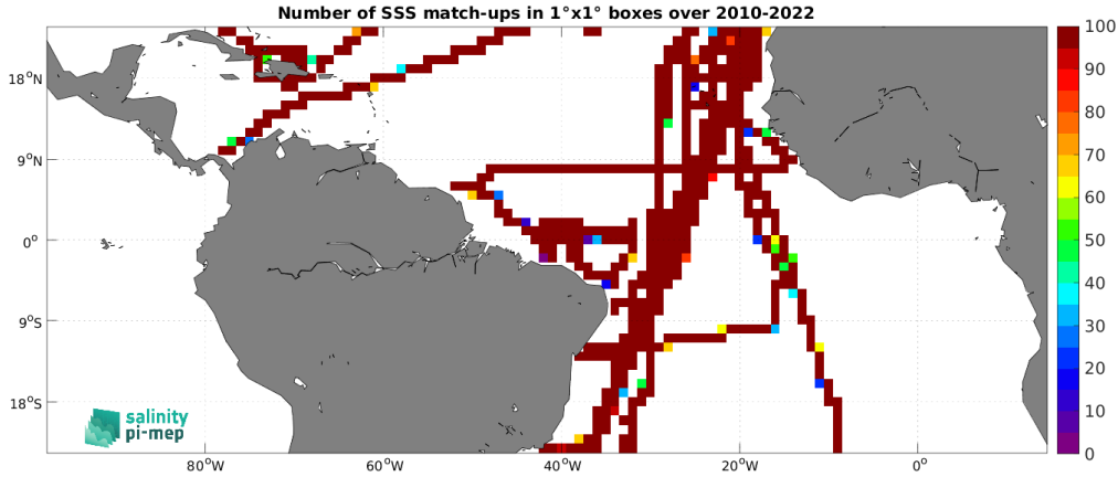
Figure 4: Number of SSS match-ups between TSG (CSIC-UTM) SSS and the SMOS SSS L3 v8 - 18 Days (CATDS-CEC-LOCEAN) SSS product for the Tropical Atlantic Ocean Pi-MEP region over 1^\circ \times 1^\circ boxes and for the full satellite product period.
