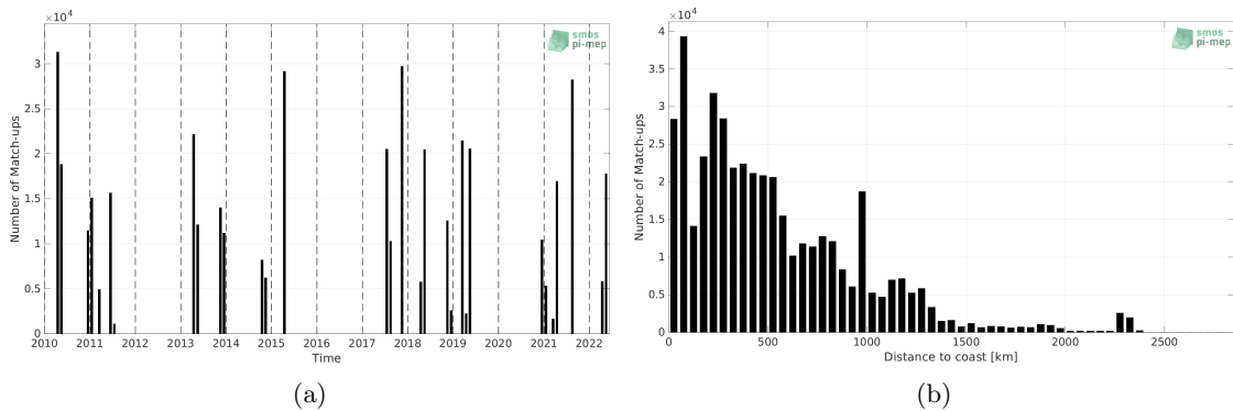
Figure 1: Number of match-ups between TSG (CSIC-UTM) and SMOS SSS L3 v8 - 18 Days (CATDS-CECOS-LOCEAN) SSS as a function of time (a) and as function of the distance to coast (b) over the Tropical Atlantic Ocean Pi-MEP region and for the full satellite product period.
