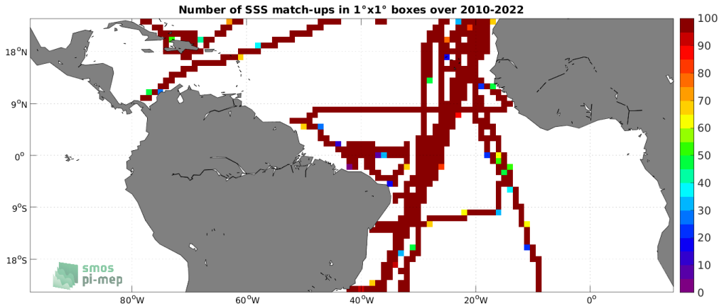
Figure 4: Number of SSS match-ups between TSG (CSIC-UTM) SSS and the SMOS SSS L3 v8 - 18 Days (CATDS-CECOS-LOCEAN) SSS product for the Tropical Atlantic Ocean Pi-MEP region over 1^\circ \times 1^\circ boxes and for the full satellite product period.
