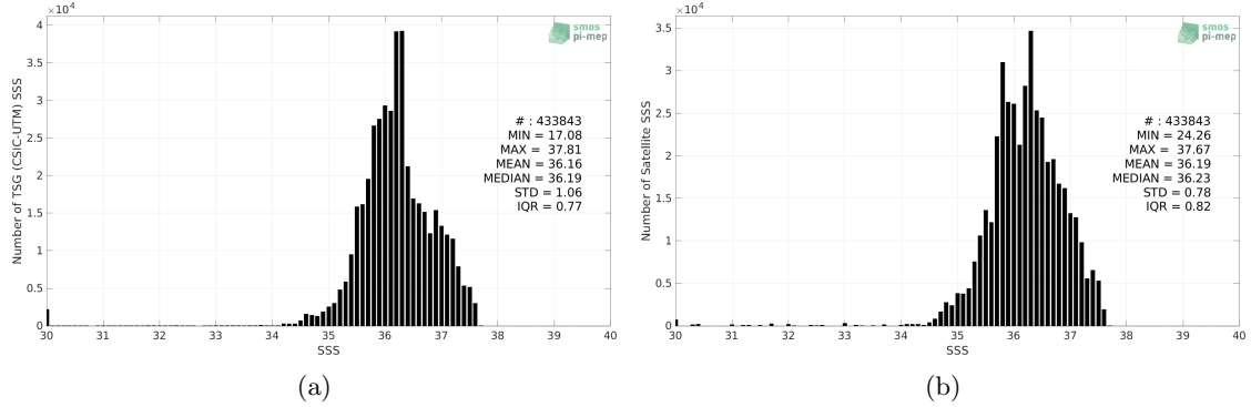
Figure 2: Histograms of SSS from TSG (CSIC-UTM) (a) and SMOS SSS L3 v8 - 18 Days (CATDS-CECOS-LOCEAN) (b) considering all match-up pairs per bins of 0.1 over the Tropical Atlantic Ocean Pi-MEP region and for the full satellite product period.
