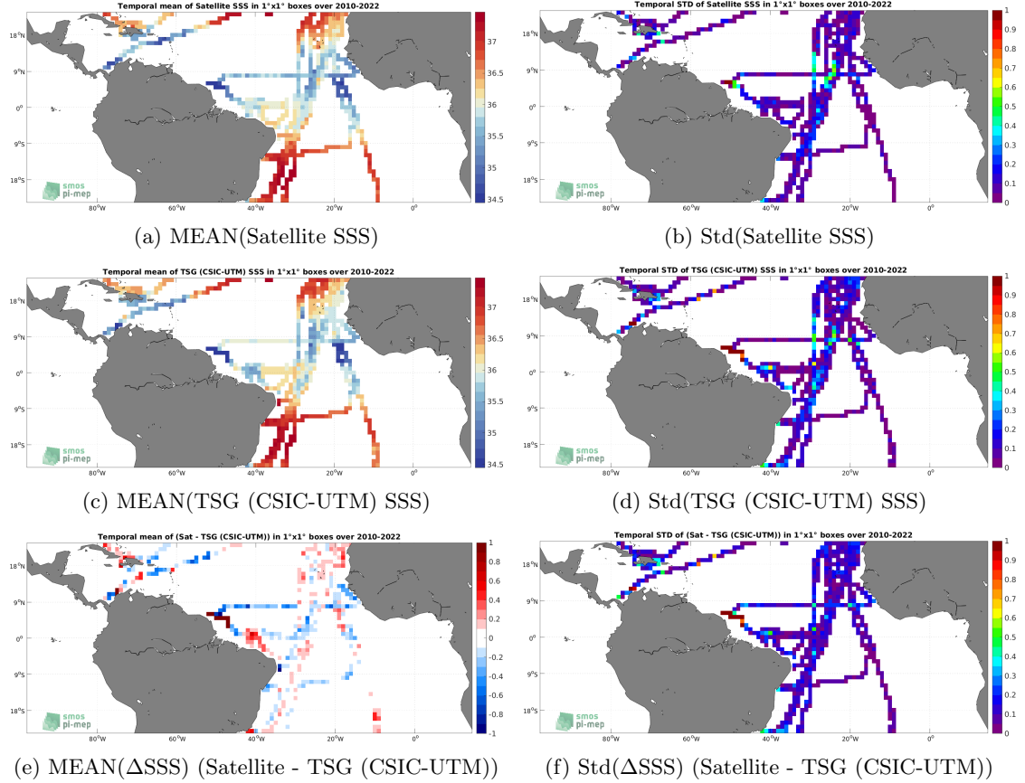
Figure 6: Temporal mean (left) and Std (right) of SSS from SMOS SSS L3 v8 - 18 Days (CATDS-CECOS-LOCEAN) (top), TSG (CSIC-UTM) ( in situ ) dataset (middle), and of \Delta\text{SSS} (Satellite - TSG (CSIC-UTM)). Only match-up pairs are used to generate these maps.
