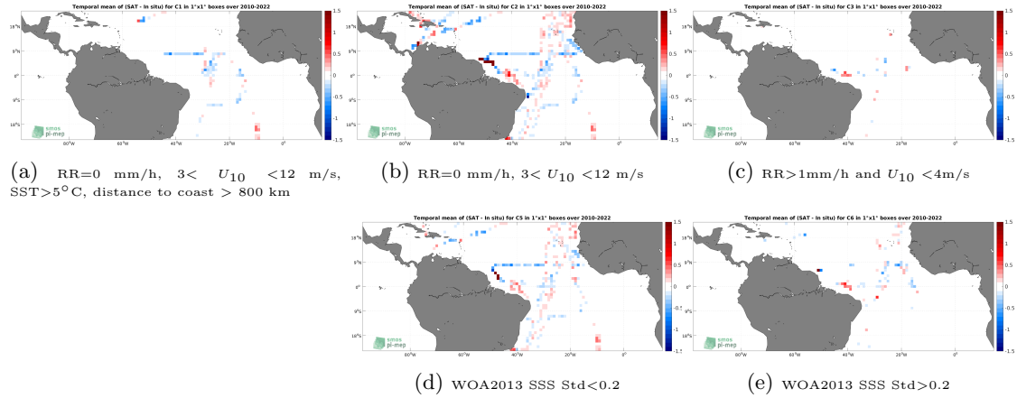
Figure 12: Temporal mean gridded over spatial boxes of size 1^{\circ}\times 1^{\circ} of \Delta\text{SSS} (SMOS SSS L3 v8 - 18 Days (CATDS-CECOS-LOCEAN) - TSG (CSIC-UTM)) for 5 different subdatasets corresponding to:RR=0 mm/h, 3 < U_{10} < 12 m/s, SST > 5^{\circ}\text{C} , distance to coast > 800 km (a), RR=0 mm/h, 3 < U_{10} < 12 m/s (b), RR > 1 mm/h and U_{10} < 4 m/s (c), WOA2013 SSS Std < 0.2 (d), WOA2013 SSS Std > 0.2 (e).
