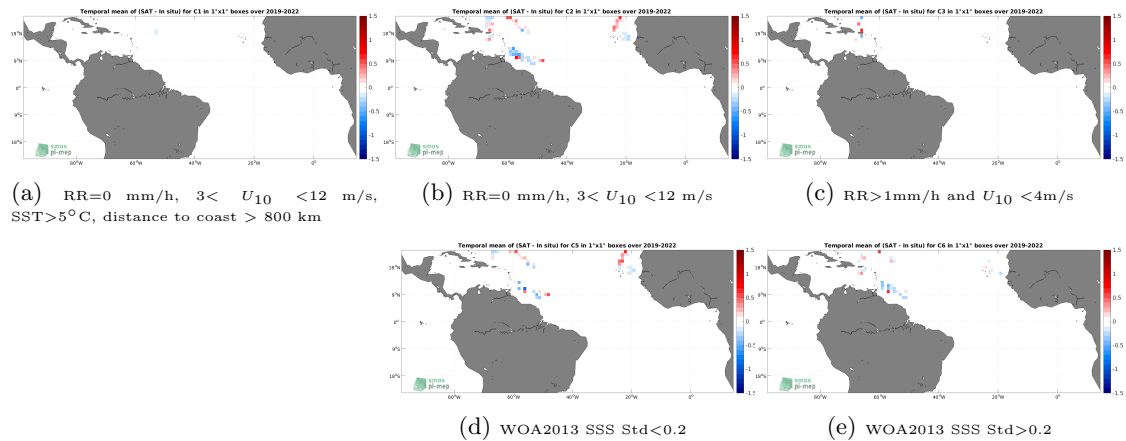
Figure 12: Temporal mean gridded over spatial boxes of size 1^\circ \times 1^\circ of \Delta\text{SSS} (SMOS SSS L3 v8 - 18 Days (CATDS-CECOS-LOCEAN) - Sairdrone) for 5 different subdatasets corresponding to:RR=0 mm/h, 3 < U_{10} < 12 m/s, SST >5^\circ\text{C} , distance to coast > 800 km (a), RR=0 mm/h, 3 < U_{10} < 12 m/s (b), RR >1 mm/h and U_{10} < 4 m/s (c), WOA2013 SSS Std <0.2 (d), WOA2013 SSS Std >0.2 (e).
