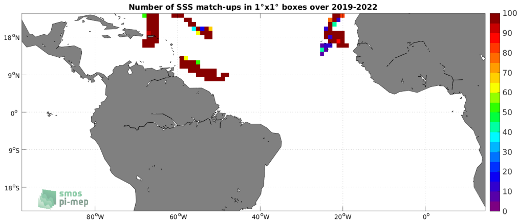
Figure 4: Number of SSS match-ups between Sairdrone SSS and the SMOS SSS L3 v8 - 18 Days (CATDS-CECOS-LOCEAN) SSS product for the Tropical Atlantic Ocean Pi-MEP region over 1^\circ \times 1^\circ boxes and for the full satellite product period.
