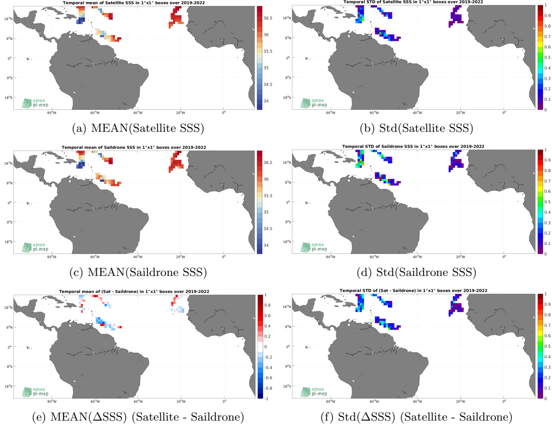
Figure 6: Temporal mean (left) and Std (right) of SSS from SMOS SSS L3 v8 - 18 Days (CATDS-CECOS-LOCEAN) (top), Saildrone (middle), and of \Delta\text{SSS} (Satellite - Saildrone). Only match-up pairs are used to generate these maps.
