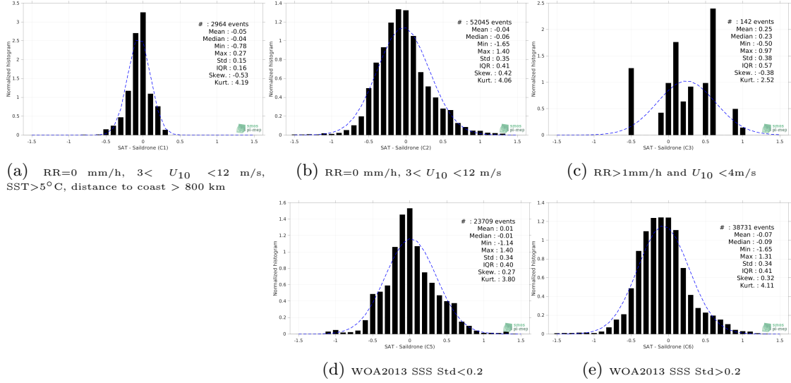
Figure 13: Normalized histogram of \Delta\text{SSS} (SMOS SSS L3 v8 - 18 Days (CATDS-CECOS-LOCEAN) - Saildrone) for 5 different subdatasets corresponding to: RR=0 mm/h, 3 < U_{10} < 12 m/s, SST>5°C, distance to coast > 800 km (a), RR=0 mm/h, 3 < U_{10} < 12 m/s (b), RR>1mm/h and U_{10} < 4 m/s (c), WOA2013 SSS Std<0.2 (d), WOA2013 SSS Std>0.2 (e).
