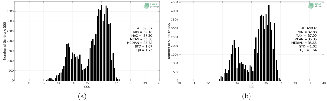
Figure 2: Histograms of SSS from Saildrone (a) and SMOS SSS L3 v8 - 18 Days (CATDS-CECOS-LOCEAN) (b) considering all match-up pairs per bins of 0.1 over the Tropical Atlantic Ocean Pi-MEP region and for the full satellite product period.
