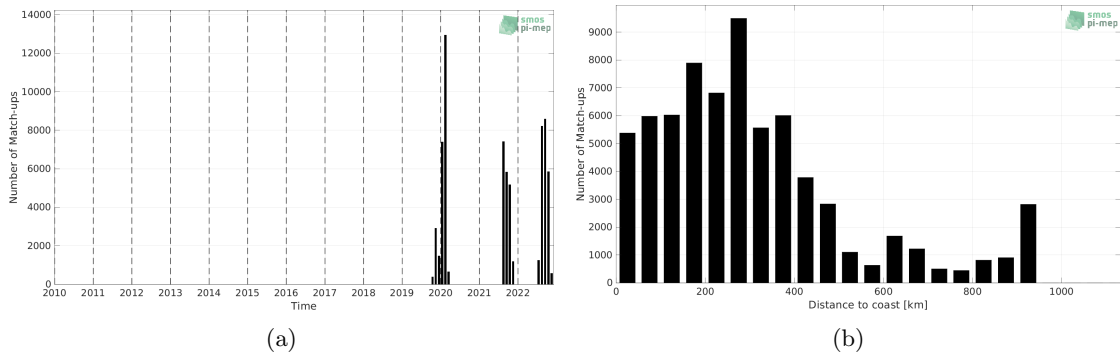
Figure 1: Number of match-ups between Saildrone and SMOS SSS L3 v8 - 18 Days (CATDS-CECOS-LOCEAN) SSS as a function of time (a) and as function of the distance to coast (b) over the Tropical Atlantic Ocean Pi-MEP region and for the full satellite product period.
