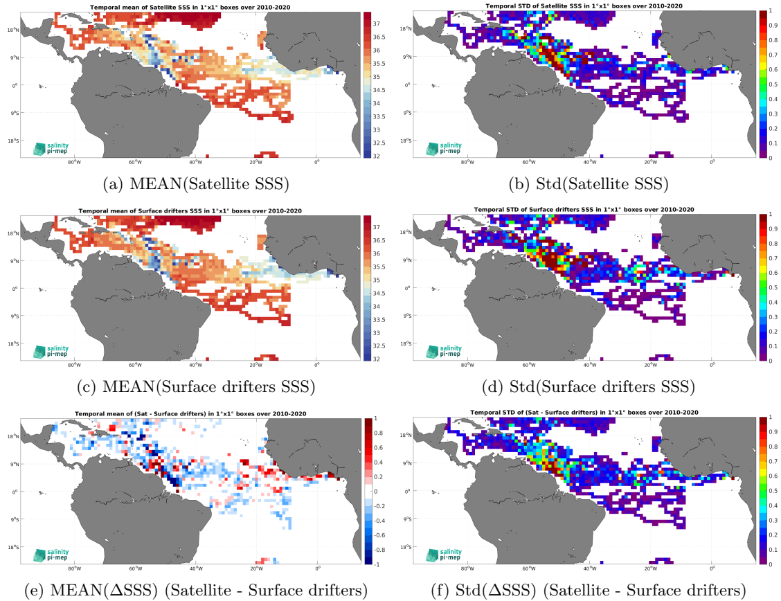
Figure 5: Temporal mean (left) and Std (right) of SSS from SMOS SSS L3 v8 - 18 Days (CATDS-CEC-LOCEAN) (top), Surface drifters (middle), and of \Delta SSS (Satellite - Surface drifters). Only match-up pairs are used to generate these maps.
