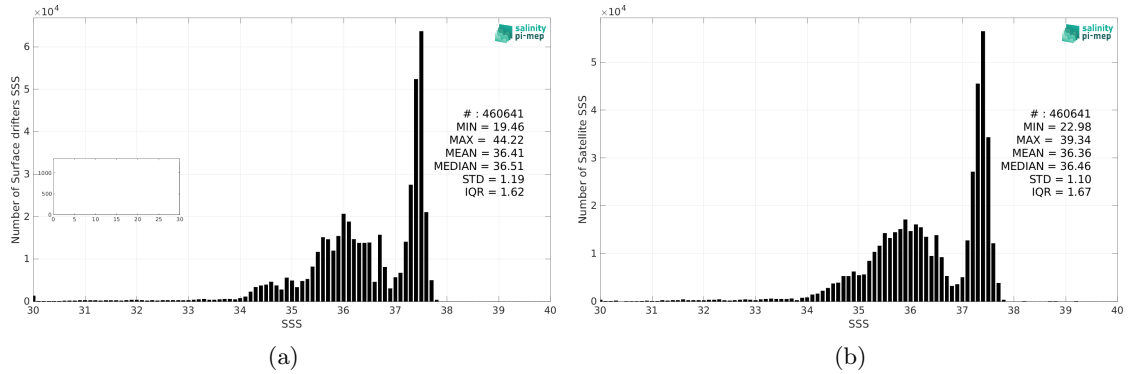
Figure 2: Histograms of SSS from Surface drifters (a) and SMOS SSS L3 v8 - 18 Days (CATDS-CEC-LOCEAN) (b) considering all match-up pairs per bins of 0.1 over the Tropical Atlantic Ocean Pi-MEP region and for the full satellite product period.
