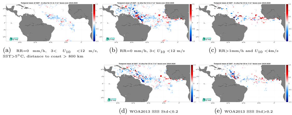
Figure 11: Temporal mean gridded over spatial boxes of size 1^\circ \times 1^\circ of \Delta SSS (SMOS SSS L3 v8 - 18 Days (CATDS-CEC-LOCEAN) - Surface drifters) for 5 different subdatasets corresponding to:RR=0 mm/h, 3 < U_{10} < 12 m/s, SST >5^\circ C, distance to coast > 800 km (a), RR=0 mm/h, 3 < U_{10} < 12 m/s (b), RR >1 mm/h and U_{10} < 4 m/s (c), WOA2013 SSS Std <0.2 (d), WOA2013 SSS Std >0.2 (e).
