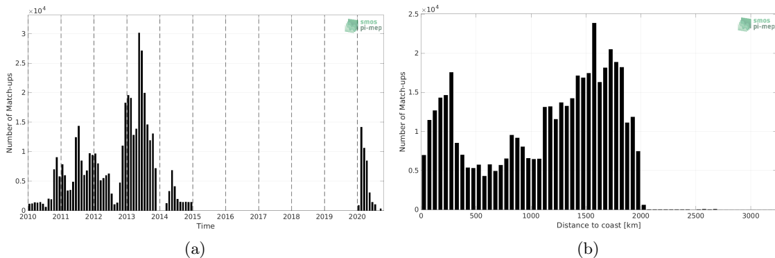
Figure 1: Number of match-ups between Surface drifters and SMOS SSS L3 v8 - 18 Days (CATDS-CECOS-LOCEAN) SSS as a function of time (a) and as function of the distance to coast (b) over the Tropical Atlantic Ocean Pi-MEP region and for the full satellite product period.
