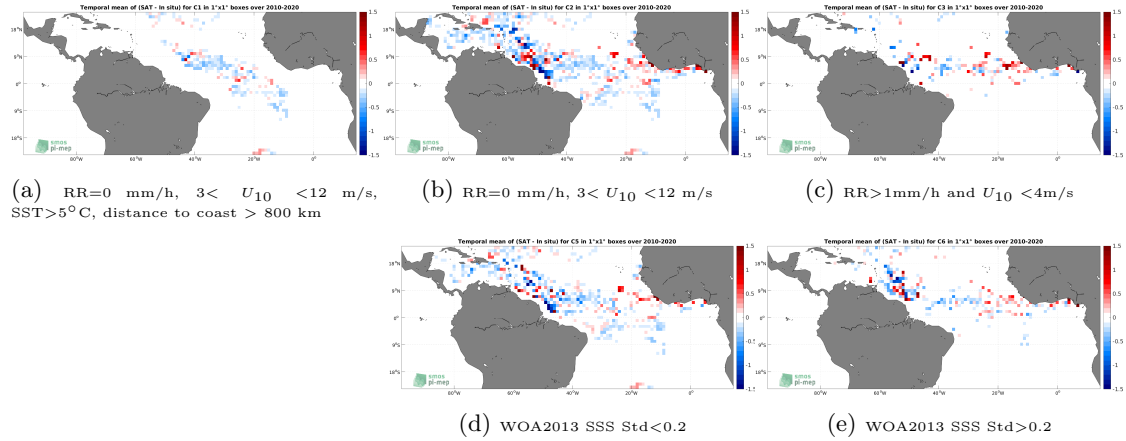
Figure 11: Temporal mean gridded over spatial boxes of size 1^{\circ}\times 1^{\circ} of \Delta\text{SSS} (SMOS SSS L3 v8 - 18 Days (CATDS-CECOS-LOCEAN) - Surface drifters) for 5 different subdatasets corresponding to:RR=0 mm/h, 3 < U_{10} < 12 m/s, SST > 5^{\circ}\text{C} , distance to coast > 800 km (a), RR=0 mm/h, 3 < U_{10} < 12 m/s (b), RR > 1 mm/h and U_{10} < 4 m/s (c), WOA2013 SSS Std < 0.2 (d), WOA2013 SSS Std > 0.2 (e).
