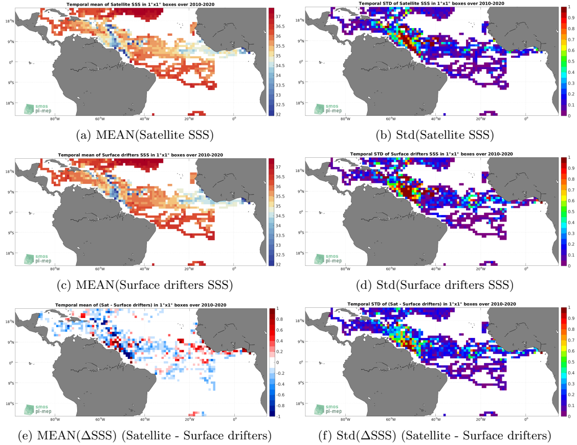
Figure 5: Temporal mean (left) and Std (right) of SSS from SMOS SSS L3 v8 - 18 Days (CATDS-CECOS-LOCEAN) (top), Surface drifters (middle), and of \Delta SSS (Satellite - Surface drifters). Only match-up pairs are used to generate these maps.
