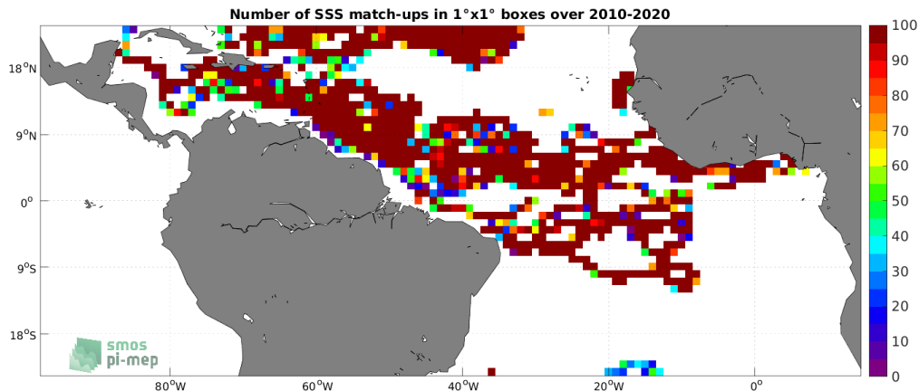
Figure 3: Number of SSS match-ups between Surface drifters SSS and the SMOS SSS L3 v8 - 18 Days (CATDS-CECOS-LOCEAN) SSS product for the Tropical Atlantic Ocean Pi-MEP region over 1^\circ \times 1^\circ boxes and for the full satellite product period.
