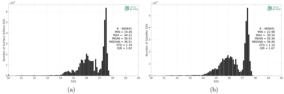
Figure 2: Histograms of SSS from Surface drifters (a) and SMOS SSS L3 v8 - 18 Days (CATDS-CECOS-LOCEAN) (b) considering all match-up pairs per bins of 0.1 over the Tropical Atlantic Ocean Pi-MEP region and for the full satellite product period.
