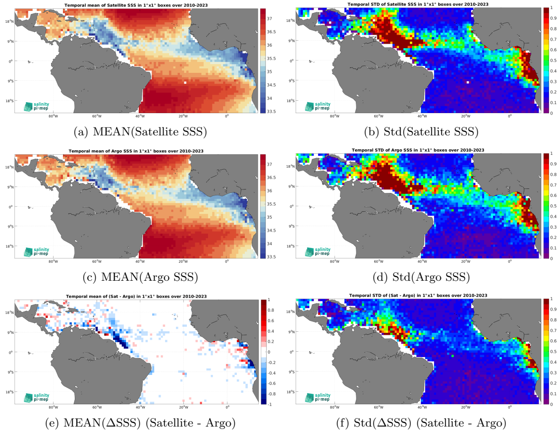
Figure 6: Temporal mean (left) and Std (right) of SSS from SMOS SSS L3 v8 - 18 Days (CATDS-CEC-LOCEAN) (top), Argo (middle), and of \Delta SSS (Satellite - Argo). Only match-up pairs are used to generate these maps.
