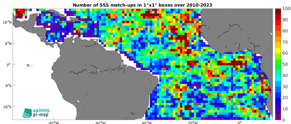
Figure 4: Number of SSS match-ups between Argo SSS and the SMOS SSS L3 v8 - 18 Days (CATDS-CEC-LOCEAN) SSS product for the Tropical Atlantic Ocean Pi-MEP region over 1^\circ \times 1^\circ boxes and for the full satellite product period.
