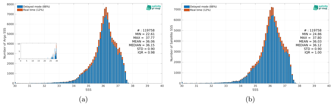
Figure 2: Histograms of SSS from Argo (a) and SMOS SSS L3 v8 - 18 Days (CATDS-CEC-LOCEAN) (b) considering all match-up pairs per bins of 0.1 over the Tropical Atlantic Ocean Pi-MEP region and for the full satellite product period.
