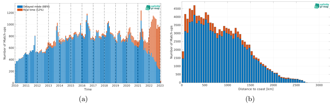
Figure 1: Number of match-ups between Argo and SMOS SSS L3 v8 - 18 Days (CATDS-CEC-LOCEAN) SSS as a function of time (a) and as function of the distance to coast (b) over the Tropical Atlantic Ocean Pi-MEP region and for the full satellite product period.
