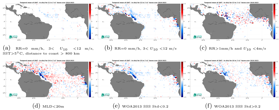
Figure 12: Temporal mean gridded over spatial boxes of size 1^\circ \times 1^\circ of \Delta SSS (SMOS SSS L3 v8 - 18 Days (CATDS-CEC-LOCEAN) - Argo) for 6 different subdatasets corresponding to:RR=0 mm/h, 3 < U_{10} < 12 m/s, SST >5^\circ C, distance to coast > 800 km (a), RR=0 mm/h, 3 < U_{10} < 12 m/s (b), RR >1 mm/h and U_{10} < 4 m/s (c),MLD <20 m (d),WOA2013 SSS Std <0.2 (e),WOA2013 SSS Std >0.2 (f).
