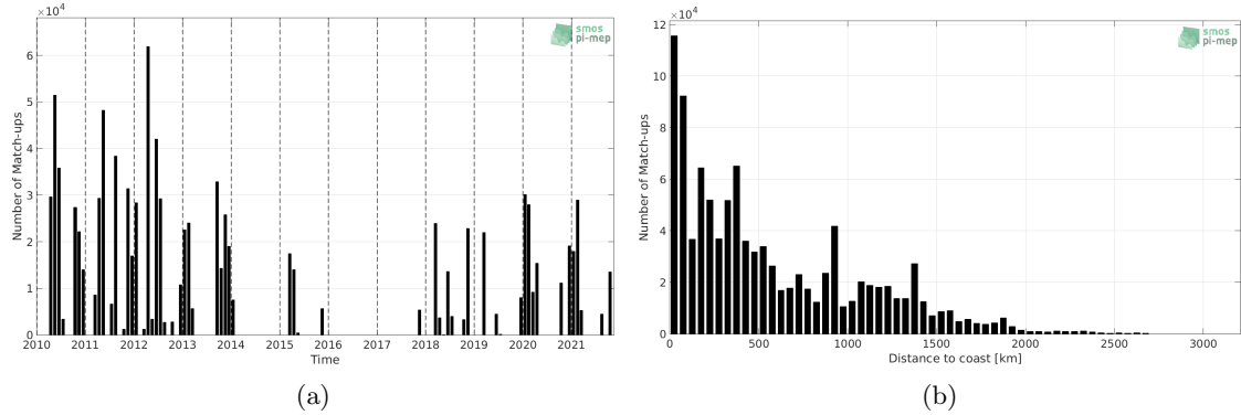
Figure 1: Number of match-ups between TSG (SAMOS) and SMOS SSS L3 v7 - 9 Days (CATDS-CECOS-LOCEAN) SSS as a function of time (a) and as function of the distance to coast (b) over the Tropical Atlantic Ocean Pi-MEP region and for the full satellite product period.
