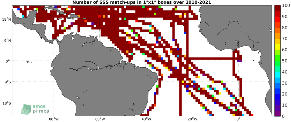
Figure 4: Number of SSS match-ups between TSG (SAMOS) SSS and the SMOS SSS L3 v7 - 9 Days (CATDS-CECOS-LOCEAN) SSS product for the Tropical Atlantic Ocean Pi-MEP region over 1^\circ \times 1^\circ boxes and for the full satellite product period.
