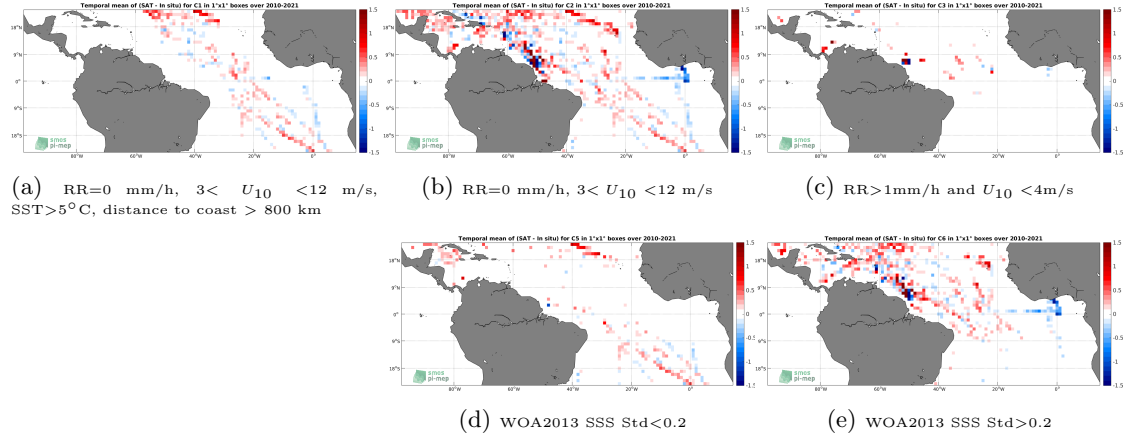
Figure 12: Temporal mean gridded over spatial boxes of size 1^{\circ}\times 1^{\circ} of \Delta\text{SSS} (SMOS SSS L3 v7 - 9 Days (CATDS-CECOS-LOCEAN) - TSG (SAMOS)) for 5 different subdatasets corresponding to: RR=0 mm/h, 3 < U_{10} < 12 m/s, SST >5^{\circ}\text{C} , distance to coast > 800 km (a), RR=0 mm/h, 3 < U_{10} < 12 m/s (b), RR >1 mm/h and U_{10} < 4 m/s (c), WOA2013 SSS Std <0.2 (d), WOA2013 SSS Std >0.2 (e).
