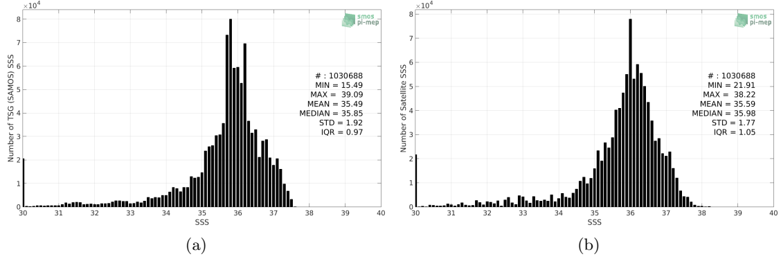
Figure 2: Histograms of SSS from TSG (SAMOS) (a) and SMOS SSS L3 v7 - 9 Days (CATDS-CECOS-LOCEAN) (b) considering all match-up pairs per bins of 0.1 over the Tropical Atlantic Ocean Pi-MEP region and for the full satellite product period.
