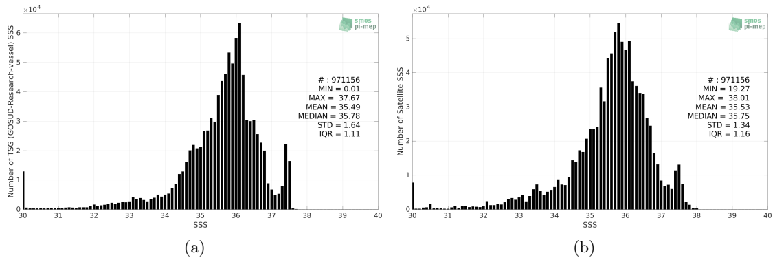
Figure 2: Histograms of SSS from TSG (GOSUD-Research-vessel) (a) and SMOS SSS L3 v7 - 9 Days (CATDS-CECOS-LOCEAN) (b) considering all match-up pairs per bins of 0.1 over the Tropical Atlantic Ocean Pi-MEP region and for the full satellite product period.
