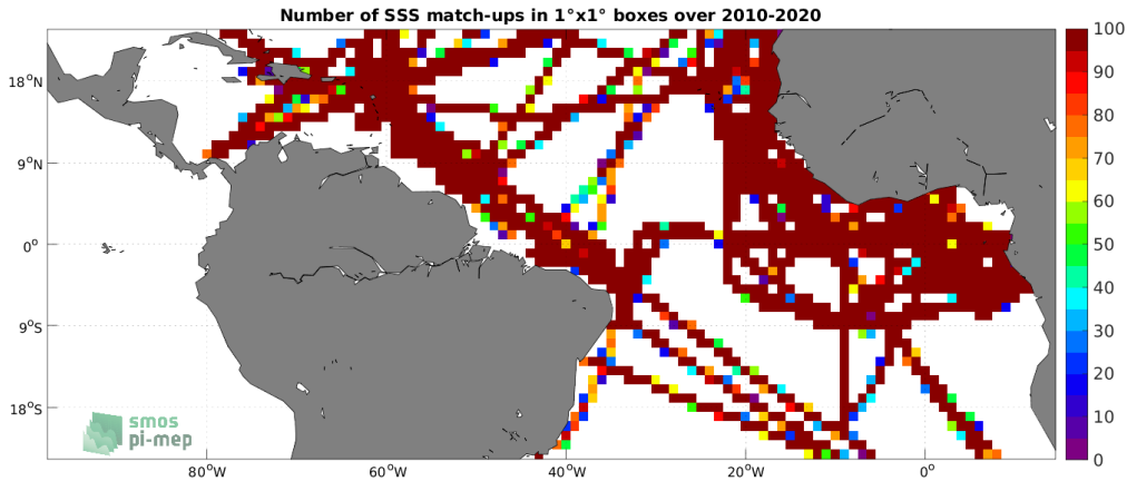
Figure 4: Number of SSS match-ups between TSG (GOSUD-Research-vessel) SSS and the SMOS SSS L3 v7 - 9 Days (CATDS-CECOS-LOCEAN) SSS product for the Tropical Atlantic Ocean Pi-MEP region over 1^\circ \times 1^\circ boxes and for the full satellite product period.
