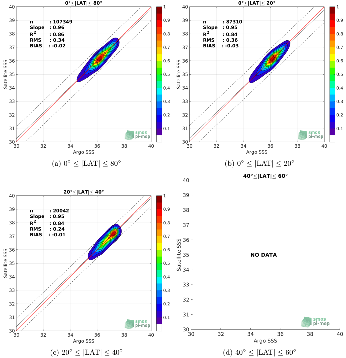
Figure 9: Contour maps of the concentration of SMOS SSS L3 v7 - 9 Days (CATDS-CECOS-LOCEAN) SSS (y-axis) versus Argo SSS (x-axis) at match-up pairs for different latitude bands. For each plot, the red line shows x=y . The black thin and dashed lines indicate a linear fit through the data cloud and the \pm 95\% confidence levels, respectively. The number match-up pairs n , the slope and R^2 coefficient of the linear fit, the root mean square (RMS) and the mean bias between satellite and in situ data are indicated for each latitude band in each plots.
