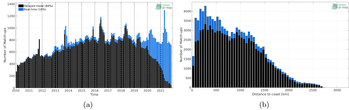
Figure 1: Number of match-ups between Argo and SMOS SSS L3 v7 - 9 Days (CATDS-CECOS-LOCEAN) SSS as a function of time (a) and as function of the distance to coast (b) over the Tropical Atlantic Ocean Pi-MEP region and for the full satellite product period.
