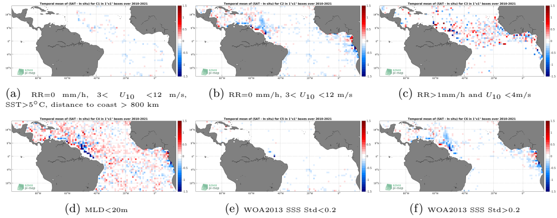
Figure 12: Temporal mean gridded over spatial boxes of size 1^\circ \times 1^\circ of \Delta SSS (SMOS SSS L3 v7 - 9 Days (CATDS-CECOS-LOCEAN) - Argo) for 6 different subdatasets corresponding to: RR=0 mm/h, 3 < U_{10} < 12 m/s, SST > 5^\circ C , distance to coast > 800 km (a), RR=0 mm/h, 3 < U_{10} < 12 m/s (b), RR > 1 mm/h and U_{10} < 4 m/s (c), MLD < 20 m (d), WOA2013 SSS Std < 0.2 (e), WOA2013 SSS Std > 0.2 (f).
