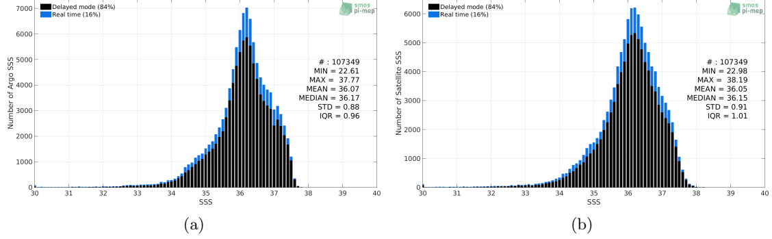
Figure 2: Histograms of SSS from Argo (a) and SMOS SSS L3 v7 - 9 Days (CATDS-CECOS-LOCEAN) (b) considering all match-up pairs per bins of 0.1 over the Tropical Atlantic Ocean Pi-MEP region and for the full satellite product period.
