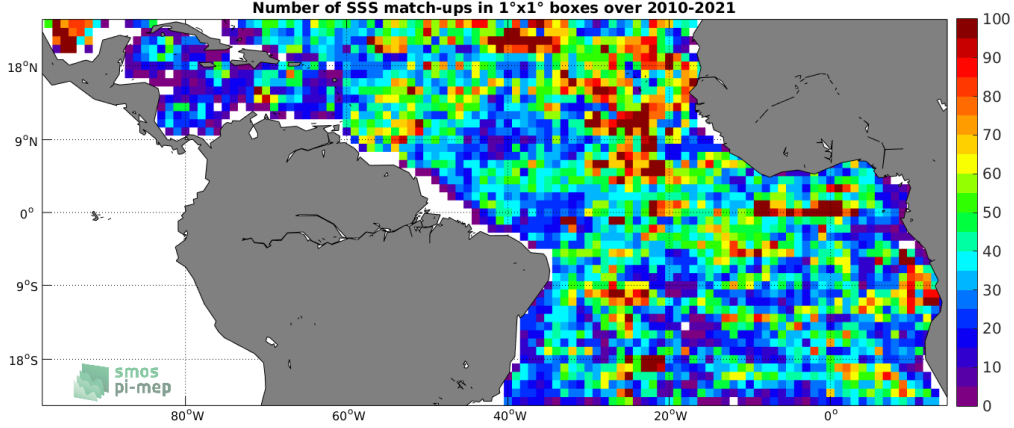
Figure 4: Number of SSS match-ups between Argo SSS and the SMOS SSS L3 v7 - 9 Days (CATDS-CECOS-LOCEAN) SSS product for the Tropical Atlantic Ocean Pi-MEP region over 1^\circ \times 1^\circ boxes and for the full satellite product period.
