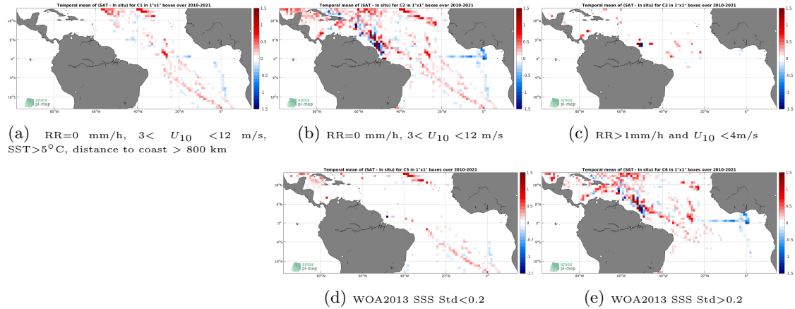
Figure 12: Temporal mean gridded over spatial boxes of size 1^{\circ}\times 1^{\circ} of \Delta\text{SSS} (SMOS SSS L3 v7 - 18 Days (CATDS-CECOS-LOCEAN) - TSG (SAMOS)) for 5 different subdatasets corresponding to:RR=0 mm/h, 3 < U_{10} < 12 m/s, SST >5^{\circ}\text{C} , distance to coast > 800 km (a), RR=0 mm/h, 3 < U_{10} < 12 m/s (b), RR >1 mm/h and U_{10} < 4 m/s (c), WOA2013 SSS Std <0.2 (d), WOA2013 SSS Std >0.2 (e).
