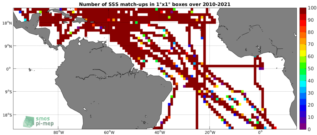
Figure 4: Number of SSS match-ups between TSG (SAMOS) SSS and the SMOS SSS L3 v7 - 18 Days (CATDS-CECOS-LOCEAN) SSS product for the Tropical Atlantic Ocean Pi-MEP region over 1^\circ \times 1^\circ boxes and for the full satellite product period.
