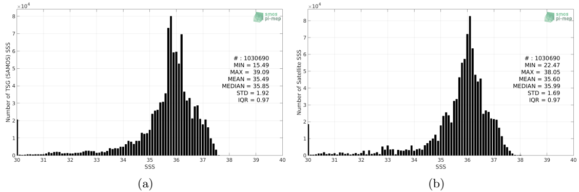
Figure 2: Histograms of SSS from TSG (SAMOS) (a) and SMOS SSS L3 v7 - 18 Days (CATDS-CECOS-LOCEAN) (b) considering all match-up pairs per bins of 0.1 over the Tropical Atlantic Ocean Pi-MEP region and for the full satellite product period.
