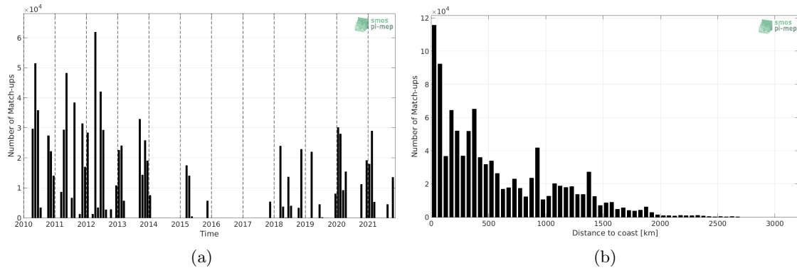
Figure 1: Number of match-ups between TSG (SAMOS) and SMOS SSS L3 v7 - 18 Days (CATDS-CECOS-LOCEAN) SSS as a function of time (a) and as function of the distance to coast (b) over the Tropical Atlantic Ocean Pi-MEP region and for the full satellite product period.
