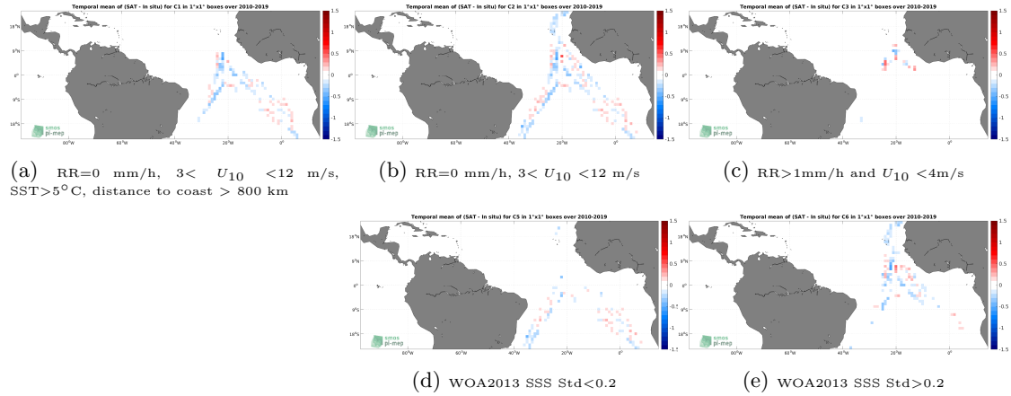
Figure 12: Temporal mean gridded over spatial boxes of size 1^{\circ}\times 1^{\circ} of \Delta\text{SSS} (SMOS SSS L3 v7 - 18 Days (CATDS-CECOS-LOCEAN) - TSG (Polarstern)) for 5 different subdatasets corresponding to:RR=0 mm/h, 3 < U_{10} < 12 m/s, SST > 5^{\circ}\text{C} , distance to coast > 800 km (a), RR=0 mm/h, 3 < U_{10} < 12 m/s (b), RR > 1 mm/h and U_{10} < 4 m/s (c), WOA2013 SSS Std < 0.2 (d), WOA2013 SSS Std > 0.2 (e).
