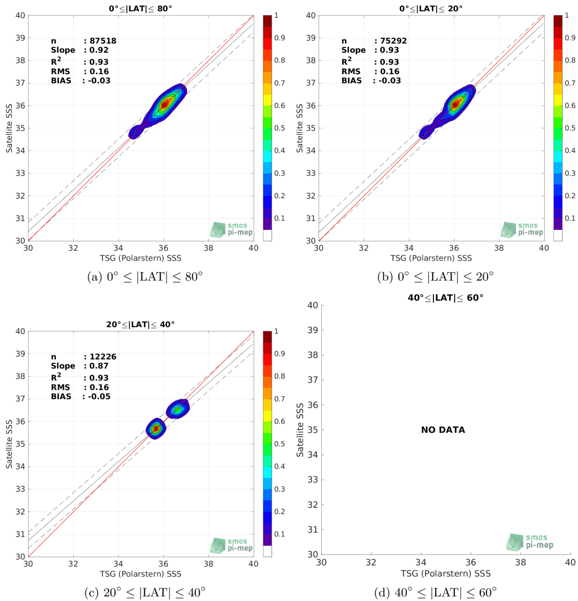
Figure 9: Contour maps of the concentration of SMOS SSS L3 v7 - 18 Days (CATDS-CECOS-LOCEAN) SSS (y-axis) versus TSG (Polarstern) SSS (x-axis) at match-up pairs for different latitude bands. For each plot, the red line shows x=y . The black thin and dashed lines indicate a linear fit through the data cloud and the \pm 95\% confidence levels, respectively. The number match-up pairs n , the slope and R^2 coefficient of the linear fit, the root mean square (RMS) and the mean bias between satellite and in situ data are indicated for each latitude band in each plots.
