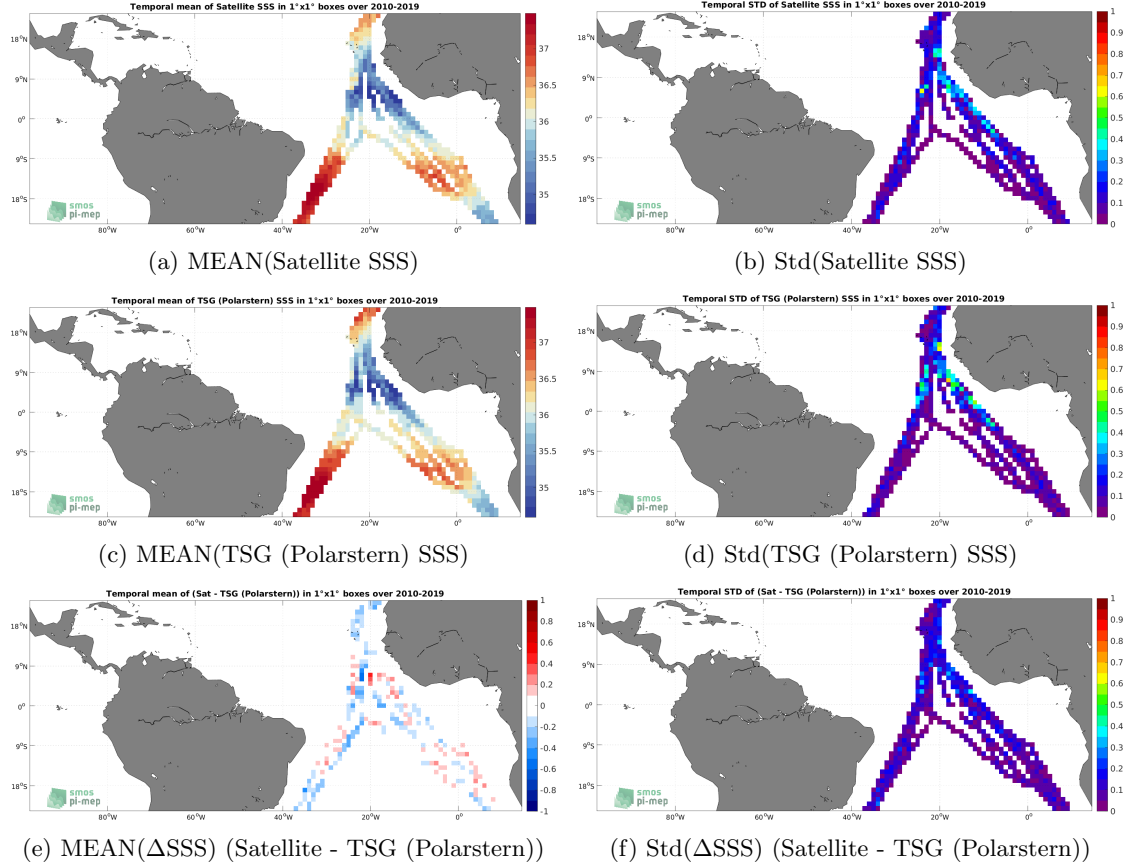
Figure 6: Temporal mean (left) and Std (right) of SSS from SMOS SSS L3 v7 - 18 Days (CATDS-CECOS-LOCEAN) (top), TSG (Polarstern) (middle), and of \Delta\text{SSS} (Satellite - TSG (Polarstern)). Only match-up pairs are used to generate these maps.
