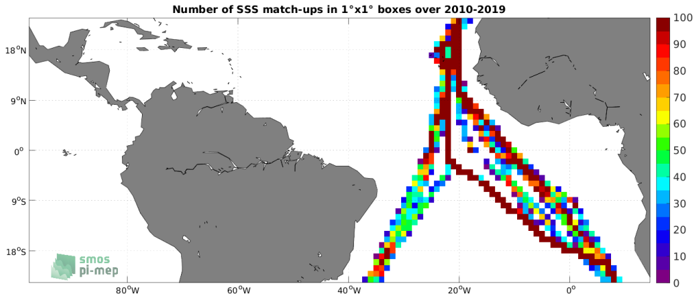
Figure 4: Number of SSS match-ups between TSG (Polarstern) SSS and the SMOS SSS L3 v7 - 18 Days (CATDS-CECOS-LOCEAN) SSS product for the Tropical Atlantic Ocean Pi-MEP region over 1^\circ \times 1^\circ boxes and for the full satellite product period.
