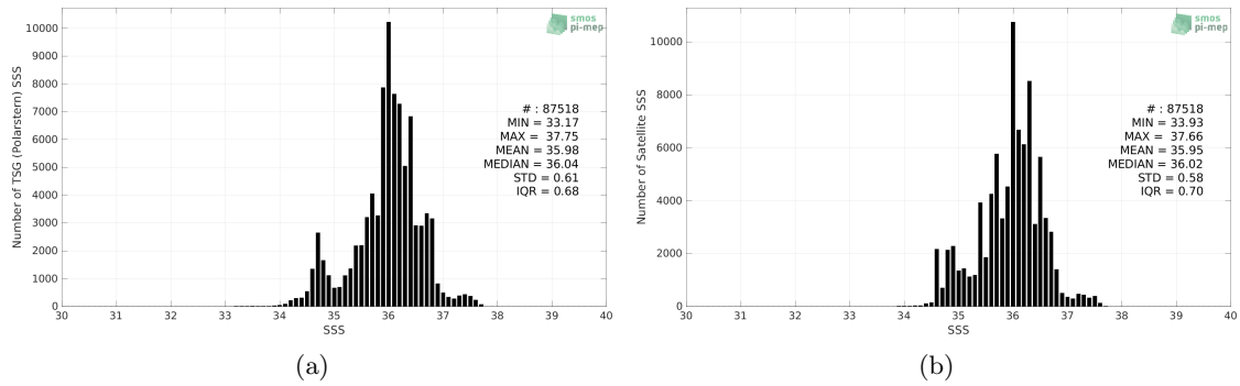
Figure 2: Histograms of SSS from TSG (Polarstern) (a) and SMOS SSS L3 v7 - 18 Days (CATDS-CECOS-LOCEAN) (b) considering all match-up pairs per bins of 0.1 over the Tropical Atlantic Ocean Pi-MEP region and for the full satellite product period.
