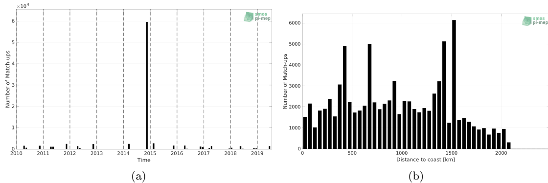
Figure 1: Number of match-ups between TSG (Polarstern) and SMOS SSS L3 v7 - 18 Days (CATDS-CECOS-LOCEAN) SSS as a function of time (a) and as function of the distance to coast (b) over the Tropical Atlantic Ocean Pi-MEP region and for the full satellite product period.
