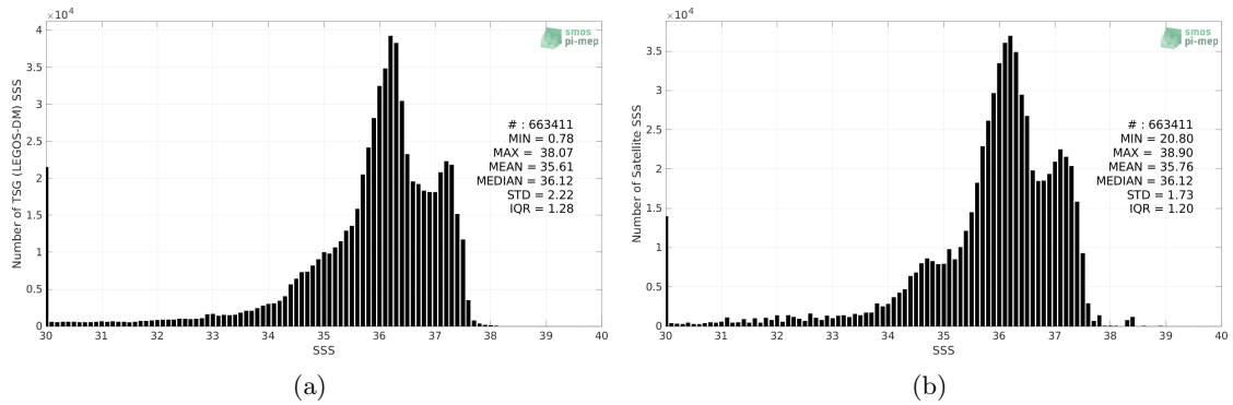
Figure 2: Histograms of SSS from TSG (LEGOS-DM) (a) and SMOS SSS L3 v7 - 18 Days (CATDS-CECOS-LOCEAN) (b) considering all match-up pairs per bins of 0.1 over the Tropical Atlantic Ocean Pi-MEP region and for the full satellite product period.
