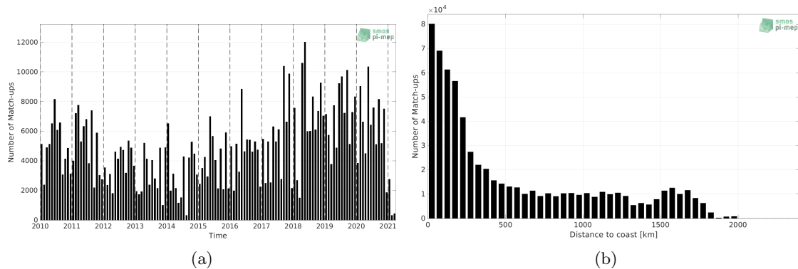
Figure 1: Number of match-ups between TSG (LEGOS-DM) and SMOS SSS L3 v7 - 18 Days (CATDS-CECOS-LOCEAN) SSS as a function of time (a) and as function of the distance to coast (b) over the Tropical Atlantic Ocean Pi-MEP region and for the full satellite product period.
