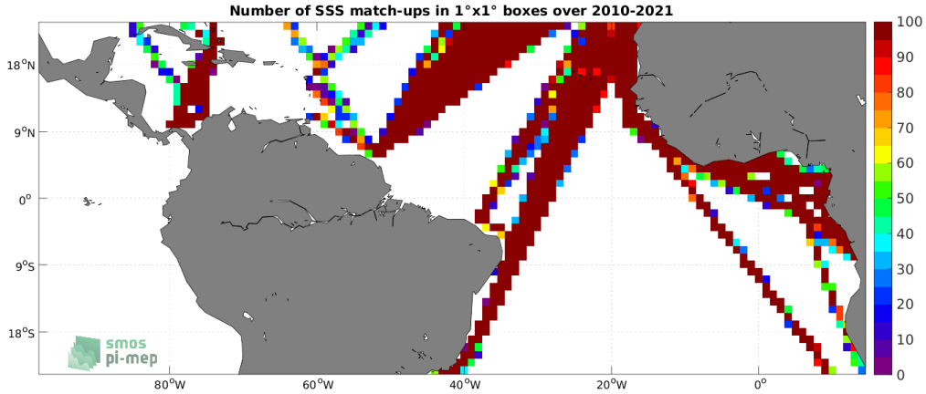
Figure 4: Number of SSS match-ups between TSG (LEGOS-DM) SSS and the SMOS SSS L3 v7 - 18 Days (CATDS-CECOS-LOCEAN) SSS product for the Tropical Atlantic Ocean Pi-MEP region over 1^\circ \times 1^\circ boxes and for the full satellite product period.
