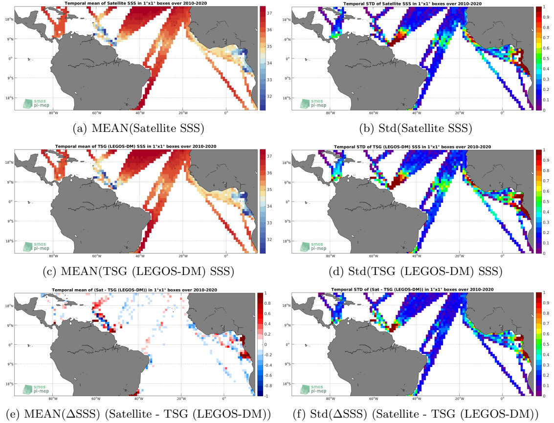
Figure 6: Temporal mean (left) and Std (right) of SSS from SMOS SSS L3 v7 - 18 Days (CATDS-CECOS-LOCEAN) (top), TSG (LEGOS-DM) ( in situ ) (middle), and of \Delta\text{SSS} (Satellite - TSG (LEGOS-DM)). Only match-up pairs are used to generate these maps.
