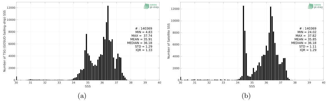
Figure 2: Histograms of SSS from TSG (GOSUD-Sailing-ship) (a) and SMOS SSS L3 v7 - 18 Days (CATDS-CECOS-LOCEAN) (b) considering all match-up pairs per bins of 0.1 over the Tropical Atlantic Ocean Pi-MEP region and for the full satellite product period.
