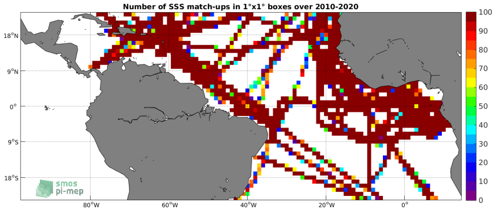
Figure 4: Number of SSS match-ups between TSG (GOSUD-Research-vessel) SSS and the SMOS SSS L3 v7 - 18 Days (CATDS-CECOS-LOCEAN) SSS product for the Tropical Atlantic Ocean Pi-MEP region over 1^\circ \times 1^\circ boxes and for the full satellite product period.
