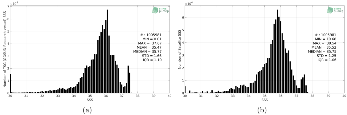
Figure 2: Histograms of SSS from TSG (GOSUD-Research-vessel) (a) and SMOS SSS L3 v7 - 18 Days (CATDS-CECOS-LOCEAN) (b) considering all match-up pairs per bins of 0.1 over the Tropical Atlantic Ocean Pi-MEP region and for the full satellite product period.
