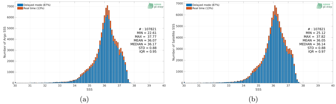
Figure 2: Histograms of SSS from Argo (a) and SMOS SSS L3 v7 - 18 Days (CATDS-CECOS-LOCEAN) (b) considering all match-up pairs per bins of 0.1 over the Tropical Atlantic Ocean Pi-MEP region and for the full satellite product period.
