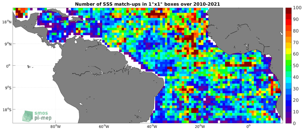
Figure 4: Number of SSS match-ups between Argo SSS and the SMOS SSS L3 v7 - 18 Days (CATDS-CECOS-LOCEAN) SSS product for the Tropical Atlantic Ocean Pi-MEP region over 1^\circ \times 1^\circ boxes and for the full satellite product period.
