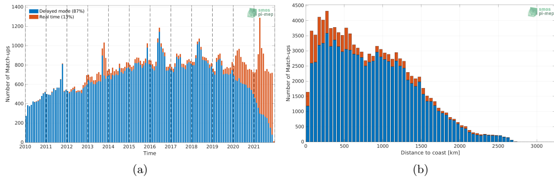
Figure 1: Number of match-ups between Argo and SMOS SSS L3 v7 - 18 Days (CATDS-CECOS-LOCEAN) SSS as a function of time (a) and as function of the distance to coast (b) over the Tropical Atlantic Ocean Pi-MEP region and for the full satellite product period.
