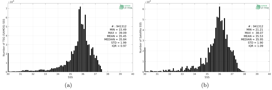
Figure 2: Histograms of SSS from TSG (SAMOS) (a) and SMOS SSS L3 v5 - 9 Days (CATDS-CECOS-LOCEAN) (b) considering all match-up pairs per bins of 0.1 over the Tropical Atlantic Ocean Pi-MEP region and for the full satellite product period.
