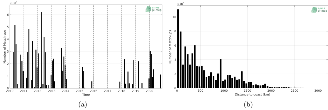
Figure 1: Number of match-ups between TSG (SAMOS) and SMOS SSS L3 v5 - 9 Days (CATDS-CECOS-LOCEAN) SSS as a function of time (a) and as function of the distance to coast (b) over the Tropical Atlantic Ocean Pi-MEP region and for the full satellite product period.
