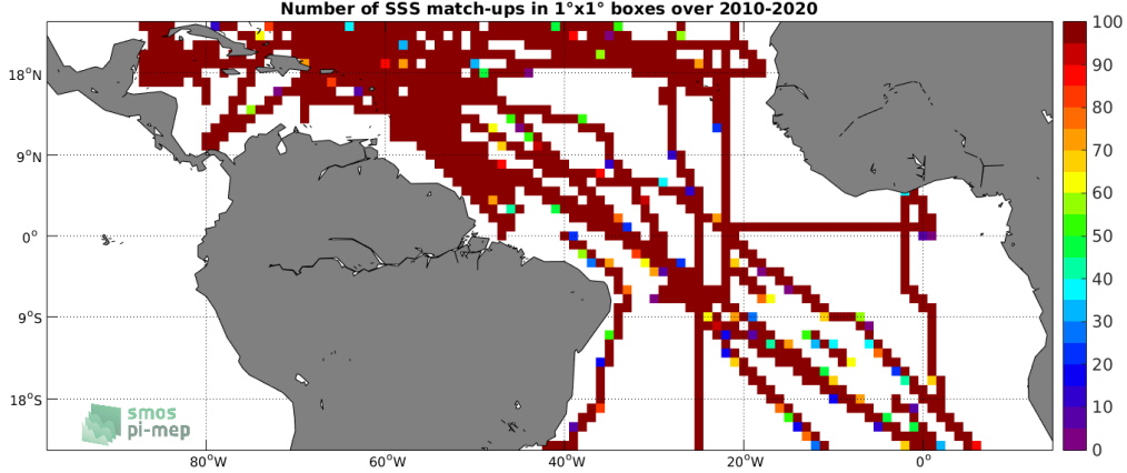
Figure 4: Number of SSS match-ups between TSG (SAMOS) SSS and the SMOS SSS L3 v5 - 9 Days (CATDS-CECOS-LOCEAN) SSS product for the Tropical Atlantic Ocean Pi-MEP region over 1^\circ \times 1^\circ boxes and for the full satellite product period.
