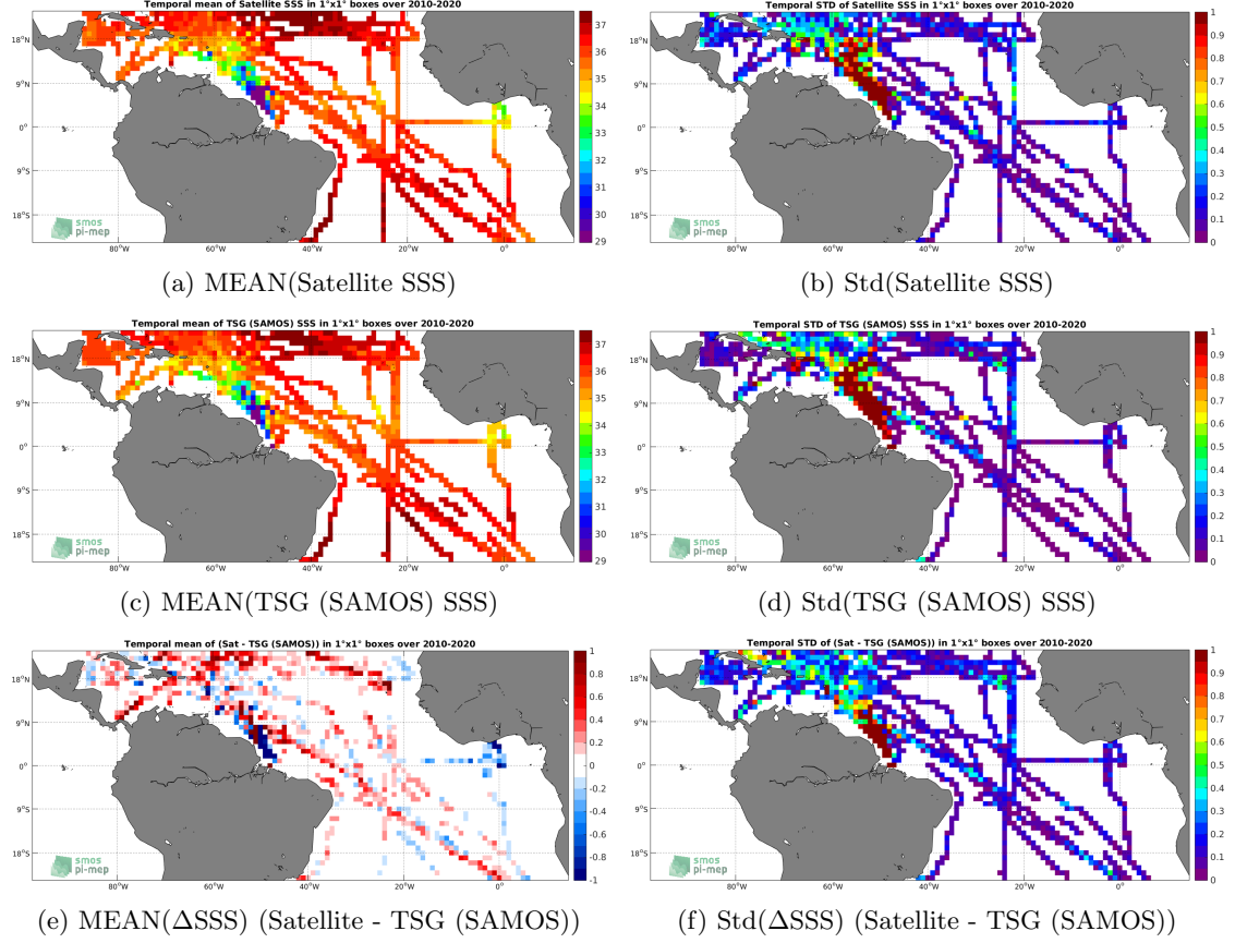
Figure 6: Temporal mean (left) and Std (right) of SSS from SMOS SSS L3 v5 - 9 Days (CATDS-CECOS-LOCEAN) (top), TSG (SAMOS) (middle), and of \Delta\text{SSS} (Satellite - TSG (SAMOS)). Only match-up pairs are used to generate these maps.
