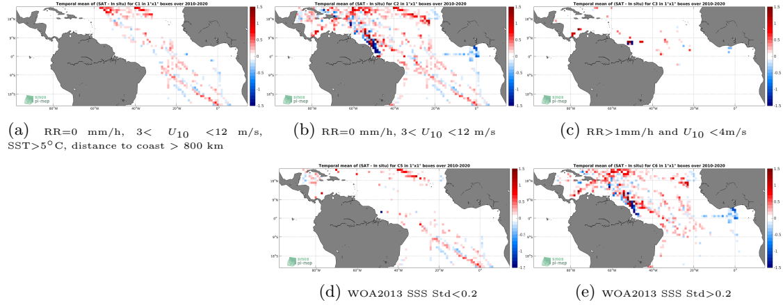
Figure 12: Temporal mean gridded over spatial boxes of size 1^{\circ}\times 1^{\circ} of \Delta\text{SSS} (SMOS SSS L3 v5 - 9 Days (CATDS-CECOS-LOCEAN) - TSG (SAMOS)) for 5 different subdatasets corresponding to: RR=0 mm/h, 3 < U_{10} < 12 m/s, SST >5^{\circ}\text{C} , distance to coast > 800 km (a), RR=0 mm/h, 3 < U_{10} < 12 m/s (b), RR >1 mm/h and U_{10} < 4 m/s (c), WOA2013 SSS Std <0.2 (d), WOA2013 SSS Std >0.2 (e).
