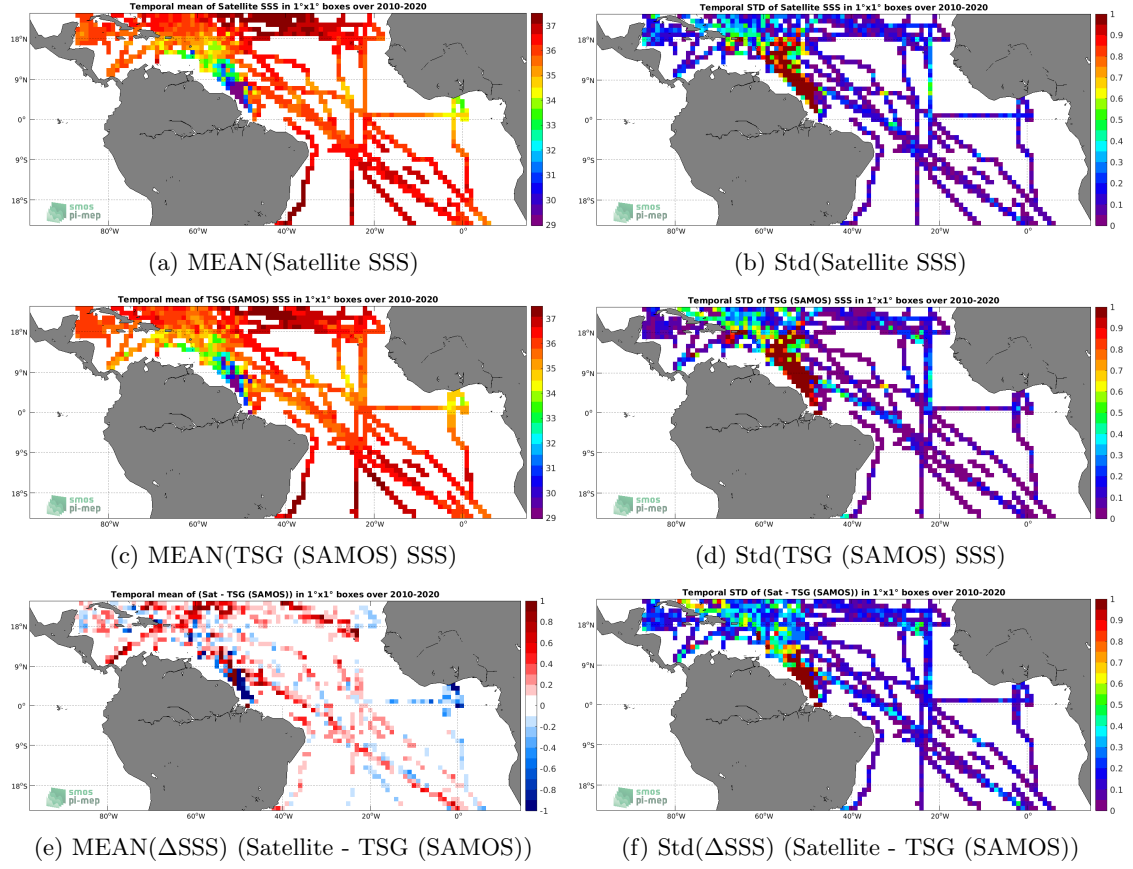
Figure 6: Temporal mean (left) and Std (right) of SSS from SMOS SSS L3 v5 - 9 Days (CATDS-CECOS-LOCEAN) (top), TSG (SAMOS) (middle), and of \Delta SSS (Satellite - TSG (SAMOS)). Only match-up pairs are used to generate these maps.
