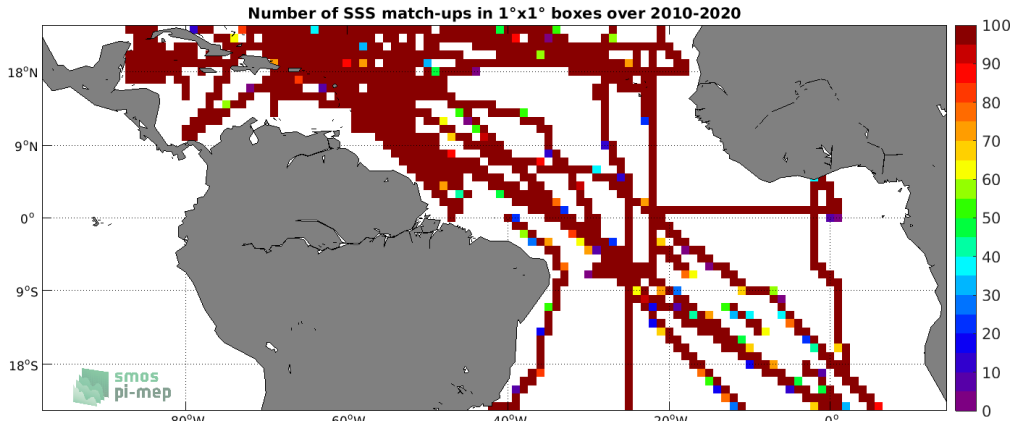
Figure 4: Number of SSS match-ups between TSG (SAMOS) SSS and the SMOS SSS L3 v5 - 9 Days (CATDS-CECOS-LOCEAN) SSS product for the Tropical Atlantic Ocean Pi-MEP region over 1^\circ \times 1^\circ boxes and for the full satellite product period.
