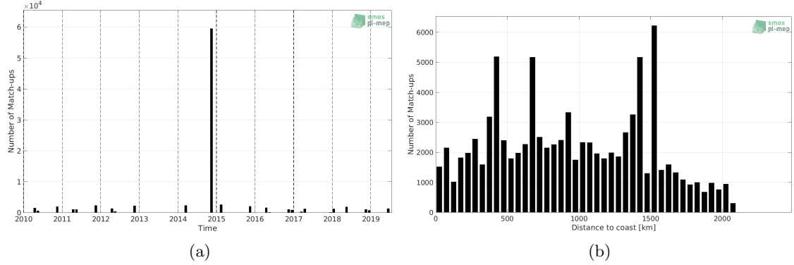
Figure 1: Number of match-ups between TSG (Polarstern) and SMOS SSS L3 v5 - 9 Days (CATDS-CECOS-LOCEAN) SSS as a function of time (a) and as function of the distance to coast (b) over the Tropical Atlantic Ocean Pi-MEP region and for the full satellite product period.
