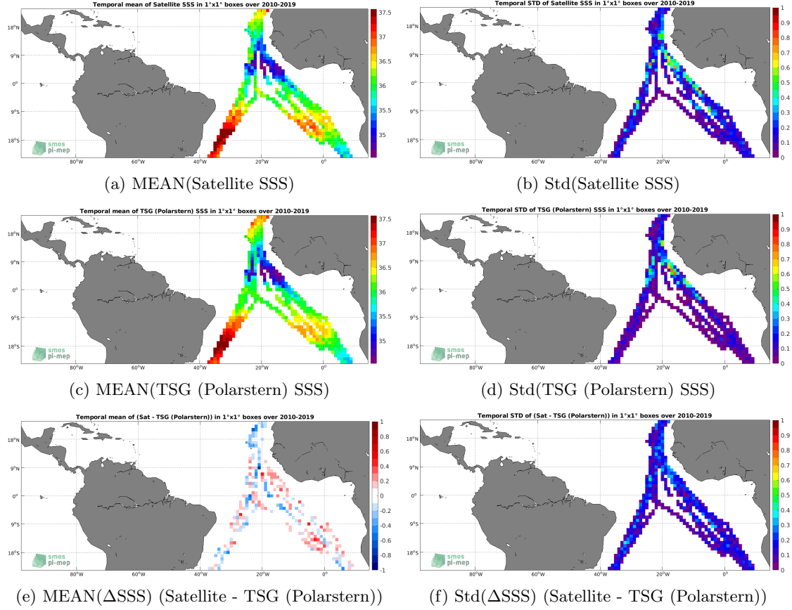
Figure 6: Temporal mean (left) and Std (right) of SSS from SMOS SSS L3 v5 - 9 Days (CATDS-CECOS-LOCEAN) (top), TSG (Polarstern) (middle), and of \Delta\text{SSS} (Satellite - TSG (Polarstern)). Only match-up pairs are used to generate these maps.
