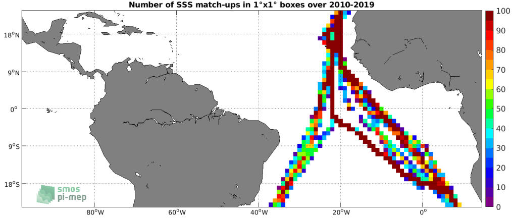
Figure 4: Number of SSS match-ups between TSG (Polarstern) SSS and the SMOS SSS L3 v5 - 9 Days (CATDS-CECOS-LOCEAN) SSS product for the Tropical Atlantic Ocean Pi-MEP region over 1^\circ \times 1^\circ boxes and for the full satellite product period.
