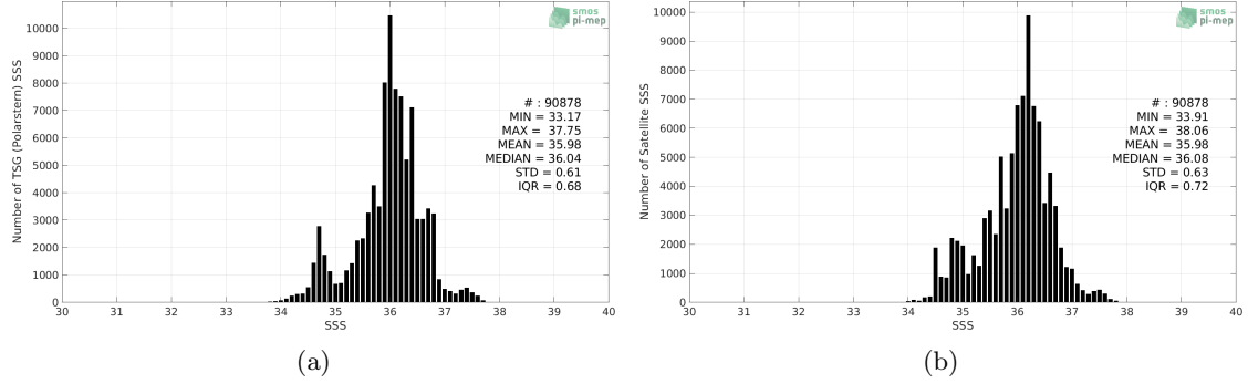
Figure 2: Histograms of SSS from TSG (Polarstern) (a) and SMOS SSS L3 v5 - 9 Days (CATDS-CECOS-LOCEAN) (b) considering all match-up pairs per bins of 0.1 over the Tropical Atlantic Ocean Pi-MEP region and for the full satellite product period.
