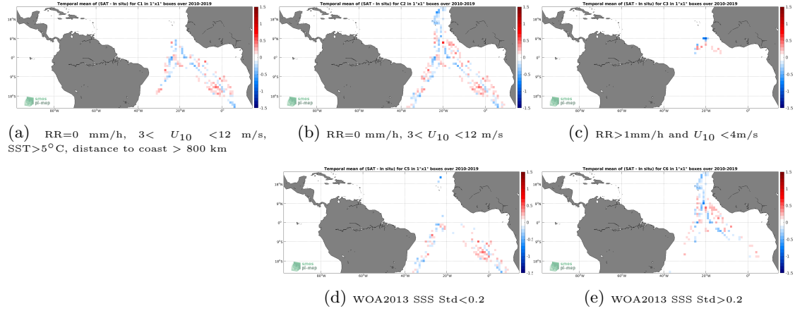
Figure 12: Temporal mean gridded over spatial boxes of size 1^{\circ}\times 1^{\circ} of \Delta\text{SSS} (SMOS SSS L3 v5 - 9 Days (CATDS-CECOS-LOCEAN) - TSG (Polarstern)) for 5 different subdatasets corresponding to:RR=0 mm/h, 3 < U_{10} < 12 m/s, SST >5^{\circ}\text{C} , distance to coast > 800 km (a), RR=0 mm/h, 3 < U_{10} < 12 m/s (b), RR >1 mm/h and U_{10} < 4 m/s (c), WOA2013 SSS Std <0.2 (d), WOA2013 SSS Std >0.2 (e).
