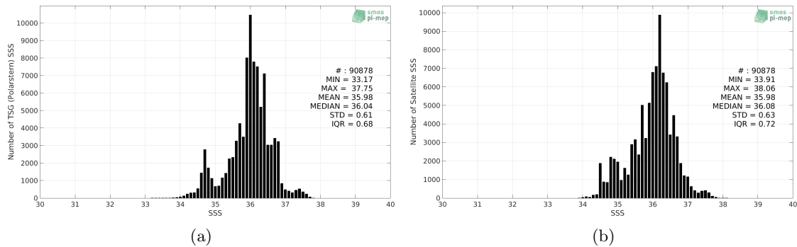
Figure 2: Histograms of SSS from TSG (Polarstern) (a) and SMOS SSS L3 v5 - 9 Days (CATDS-CECOS-LOCEAN) (b) considering all match-up pairs per bins of 0.1 over the Tropical Atlantic Ocean Pi-MEP region and for the full satellite product period.
