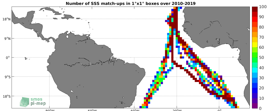
Figure 4: Number of SSS match-ups between TSG (Polarstern) SSS and the SMOS SSS L3 v5 - 9 Days (CATDS-CECOS-LOCEAN) SSS product for the Tropical Atlantic Ocean Pi-MEP region over 1^\circ \times 1^\circ boxes and for the full satellite product period.
