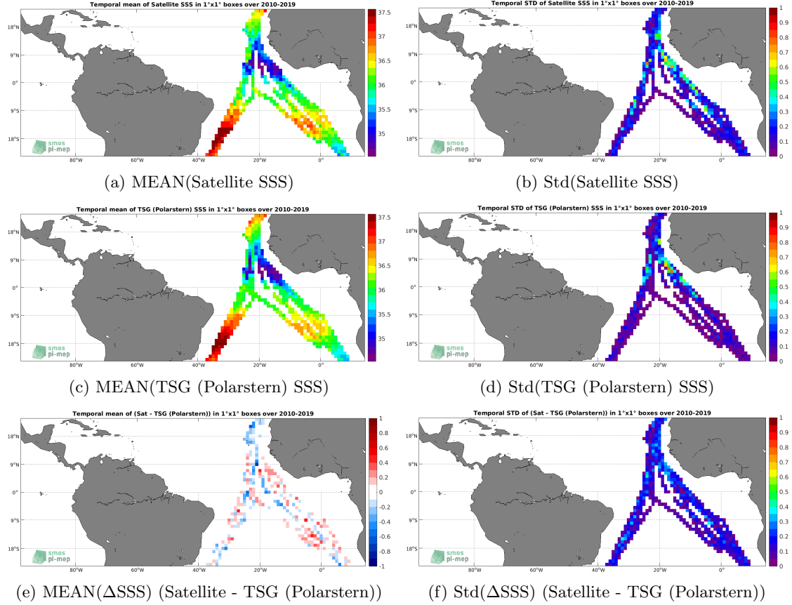
Figure 6: Temporal mean (left) and Std (right) of SSS from SMOS SSS L3 v5 - 9 Days (CATDS-CECOS-LOCEAN) (top), TSG (Polarstern) (middle), and of \Delta SSS (Satellite - TSG (Polarstern)). Only match-up pairs are used to generate these maps.
