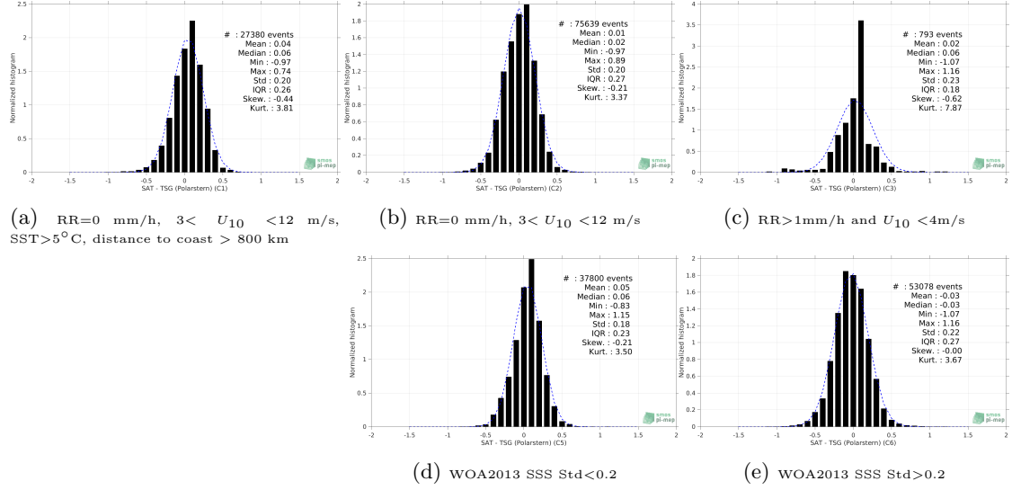
Figure 13: Normalized histogram of \Delta SSS (SMOS SSS L3 v5 - 9 Days (CATDS-CECOS-LOCEAN) - TSG (Polarstern)) for 5 different subdatasets corresponding to: RR=0 mm/h, 3 < U_{10} < 12 m/s, SST>5°C, distance to coast > 800 km (a), RR=0 mm/h, 3 < U_{10} < 12 m/s (b), RR>1mm/h and U_{10} < 4 m/s (c), WOA2013 SSS Std<0.2 (d), WOA2013 SSS Std>0.2 (e).
