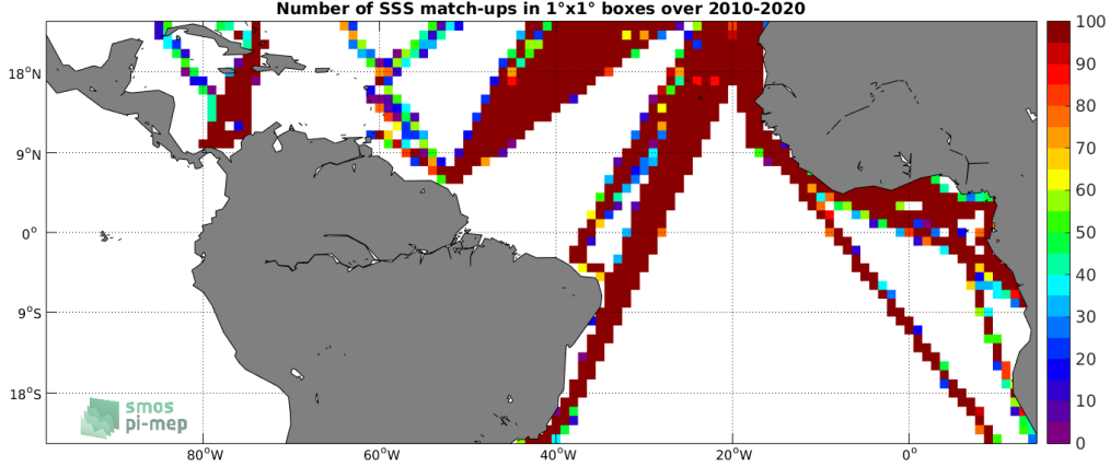
Figure 4: Number of SSS match-ups between TSG (LEGOS-DM) SSS and the SMOS SSS L3 v5 - 9 Days (CATDS-CECOS-LOCEAN) SSS product for the Tropical Atlantic Ocean Pi-MEP region over 1^\circ \times 1^\circ boxes and for the full satellite product period.
