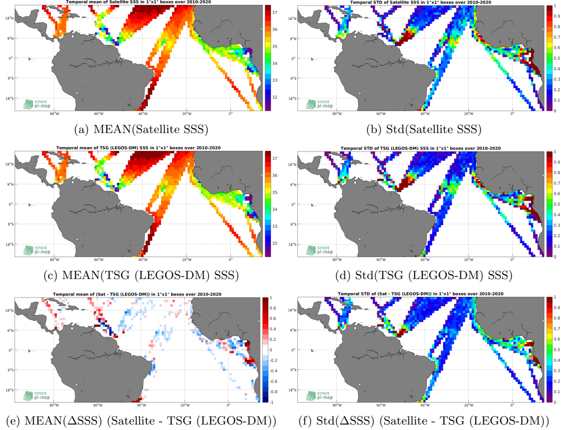
Figure 6: Temporal mean (left) and Std (right) of SSS from SMOS SSS L3 v5 - 9 Days (CATDS-CECOS-LOCEAN) (top), TSG (LEGOS-DM) (middle), and of \Delta\text{SSS} (Satellite - TSG (LEGOS-DM)). Only match-up pairs are used to generate these maps.
