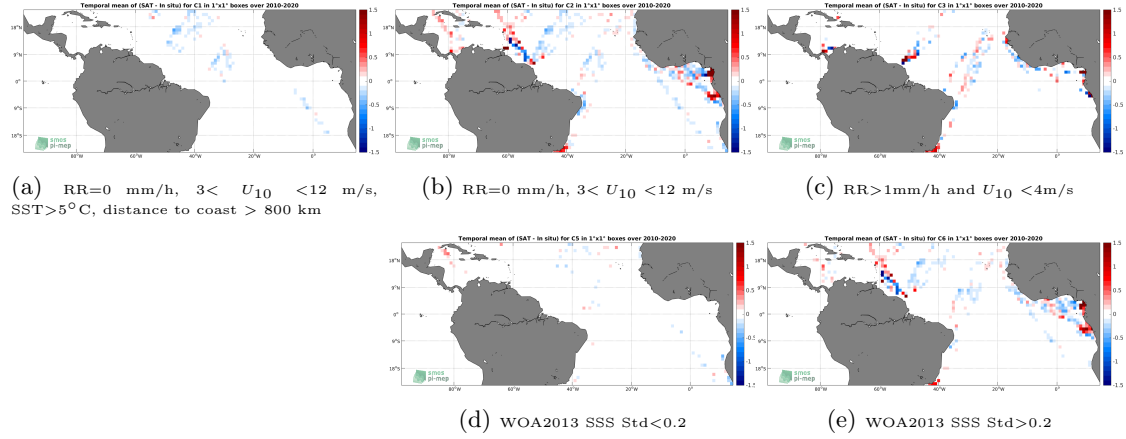
Figure 12: Temporal mean gridded over spatial boxes of size 1^{\circ}\times 1^{\circ} of \Delta\text{SSS} (SMOS SSS L3 v5 - 9 Days (CATDS-CECOS-LOCEAN) - TSG (LEGOS-DM)) for 5 different subdatasets corresponding to: RR=0 mm/h, 3 < U_{10} < 12 m/s, SST > 5^{\circ}\text{C} , distance to coast > 800 km (a), RR=0 mm/h, 3 < U_{10} < 12 m/s (b), RR > 1 mm/h and U_{10} < 4 m/s (c), WOA2013 SSS Std < 0.2 (d), WOA2013 SSS Std > 0.2 (e).
