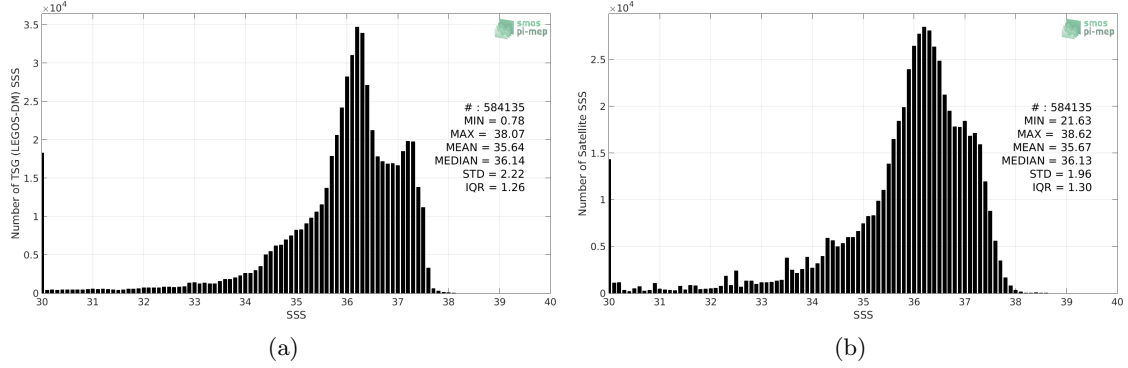
Figure 2: Histograms of SSS from TSG (LEGOS-DM) (a) and SMOS SSS L3 v5 - 9 Days (CATDS-CECOS-LOCEAN) (b) considering all match-up pairs per bins of 0.1 over the Tropical Atlantic Ocean Pi-MEP region and for the full satellite product period.
