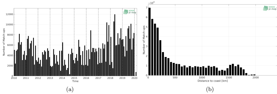
Figure 1: Number of match-ups between TSG (LEGOS-DM) and SMOS SSS L3 v5 - 9 Days (CATDS-CECOS-LOCEAN) SSS as a function of time (a) and as function of the distance to coast (b) over the Tropical Atlantic Ocean Pi-MEP region and for the full satellite product period.
