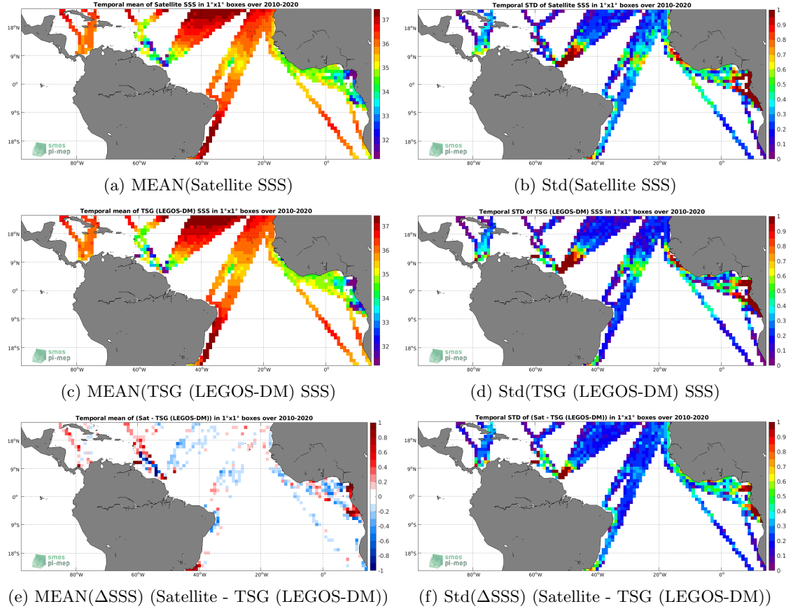
Figure 6: Temporal mean (left) and Std (right) of SSS from SMOS SSS L3 v5 - 9 Days (CATDS-CECOS-LOCEAN) (top), TSG (LEGOS-DM) (middle), and of \Delta SSS (Satellite - TSG (LEGOS-DM)). Only match-up pairs are used to generate these maps.
