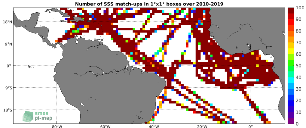
Figure 4: Number of SSS match-ups between TSG (GOSUD-Research-vessel) SSS and the SMOS SSS L3 v5 - 9 Days (CATDS-CECOS-LOCEAN) SSS product for the Tropical Atlantic Ocean Pi-MEP region over 1^\circ \times 1^\circ boxes and for the full satellite product period.
