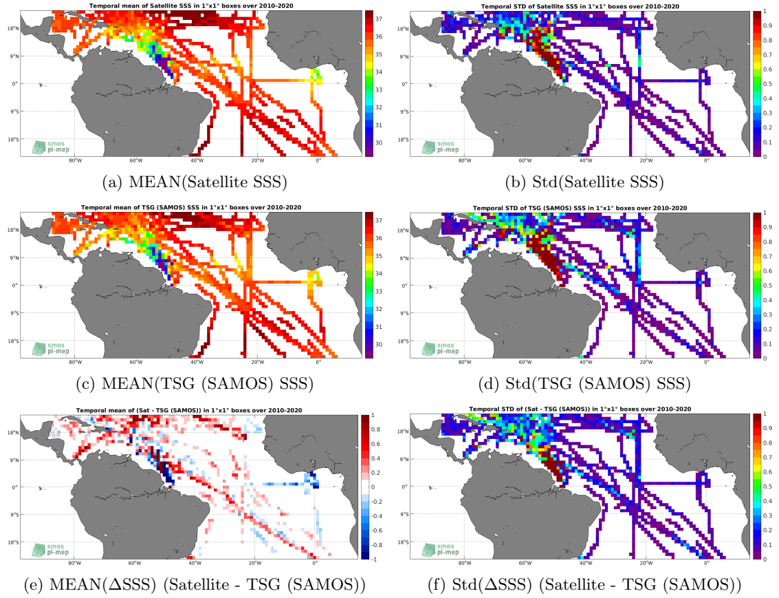
Figure 6: Temporal mean (left) and Std (right) of SSS from SMOS SSS L3 v5 - 18 Days (CATDS-CECOS-LOCEAN) (top), TSG (SAMOS) (middle), and of \Delta SSS (Satellite - TSG (SAMOS)). Only match-up pairs are used to generate these maps.
