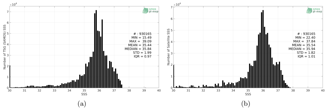
Figure 2: Histograms of SSS from TSG (SAMOS) (a) and SMOS SSS L3 v5 - 18 Days (CATDS-CECOS-LOCEAN) (b) considering all match-up pairs per bins of 0.1 over the Tropical Atlantic Ocean Pi-MEP region and for the full satellite product period.
