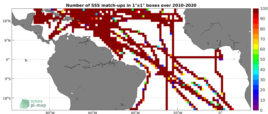
Figure 4: Number of SSS match-ups between TSG (SAMOS) SSS and the SMOS SSS L3 v5 - 18 Days (CATDS-CECOS-LOCEAN) SSS product for the Tropical Atlantic Ocean Pi-MEP region over 1^\circ \times 1^\circ boxes and for the full satellite product period.
