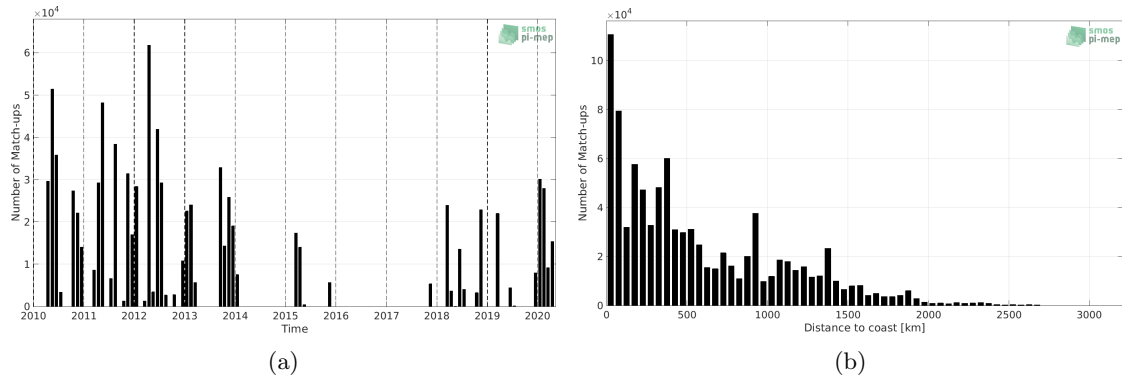
Figure 1: Number of match-ups between TSG (SAMOS) and SMOS SSS L3 v5 - 18 Days (CATDS-CECOS-LOCEAN) SSS as a function of time (a) and as function of the distance to coast (b) over the Tropical Atlantic Ocean Pi-MEP region and for the full satellite product period.
