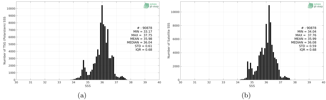
Figure 2: Histograms of SSS from TSG (Polarstern) (a) and SMOS SSS L3 v5 - 18 Days (CATDS-CECOS-LOCEAN) (b) considering all match-up pairs per bins of 0.1 over the Tropical Atlantic Ocean Pi-MEP region and for the full satellite product period.
