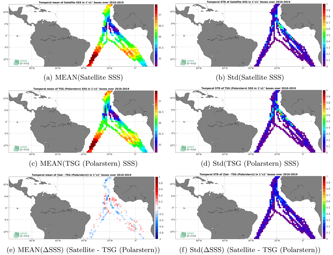
Figure 6: Temporal mean (left) and Std (right) of SSS from SMOS SSS L3 v5 - 18 Days (CATDS-CECOS-LOCEAN) (top), TSG (Polarstern) (middle), and of \Delta\text{SSS} (Satellite - TSG (Polarstern)). Only match-up pairs are used to generate these maps.
