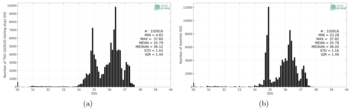
Figure 2: Histograms of SSS from TSG (GOSUD-Sailing-ship) (a) and SMOS SSS L3 v5 - 18 Days (CATDS-CECOS-LOCEAN) (b) considering all match-up pairs per bins of 0.1 over the Tropical Atlantic Ocean Pi-MEP region and for the full satellite product period.
