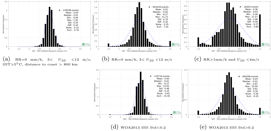
Figure 13: Normalized histogram of \Delta\text{SSS} (SMOS SSS L3 v5 - 18 Days (CATDS-CECOS-LOCEAN) - TSG (GOSUD-Research-vessel)) for 5 different subdatasets corresponding to: RR=0 mm/h, 3 < U_{10} < 12 m/s, SST > 5^\circ\text{C} , distance to coast > 800 km (a), RR=0 mm/h, 3 < U_{10} < 12 m/s (b), RR > 1 mm/h and U_{10} < 4 m/s (c), WOA2013 SSS Std < 0.2 (d), WOA2013 SSS Std > 0.2 (e).
